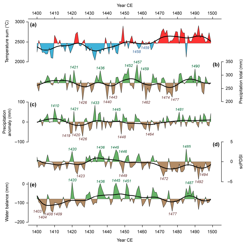
295 Figure 4. Estimated variability of climate variables over the territory of the Czech Lands in the 1400–1499 CE period: (a) annual temperature sum from oak ( Quercus spp. ) \delta^{18}\text{O} stable isotopes (Torbensoen et al., 2023); (b) March–July precipitation totals reconstructed from fir ( Abies alba ) TRWs for South Moravia (Brázdil et al., 2002); (c) May–July precipitation totals reconstructed from oak TRWs for Bohemia (Dobrovolný et al., 2018); (d) June–August self-calibrating Palmer Drought Severity Index (scPDSI) reconstructed from oak \delta^{18}\text{O} and \delta^{13}\text{C} (Büntgen et al., 2021); and (e) June–August water balance from oak \delta^{13}\text{C} (Torbensoen et al., 300 2023). Anomalies of mean annual values with respect to the 15th-century mean (with the exception of scPDSI, which is plotted in absolute values) are expressed in green and brown colours (in red and blue for temperature sums). Bold black lines indicate series smoothed by a low-pass Gaussian filter for 15 years. For each of the hydroclimate series (b)–(e), the five wettest and five driest years are indicated.
