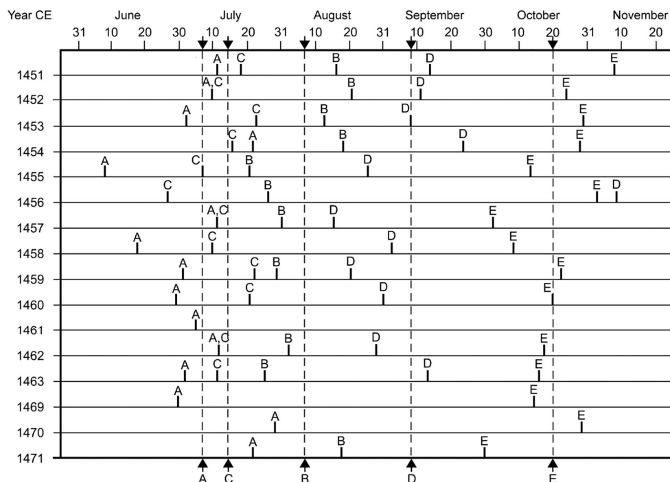
210 Figure 1. Changes in the beginnings and endings of haymaking, grain harvest and grape harvest (always in the week before the given date) in the Louny region for 1451–1463 and 1469–1471 CE according to Liber rationum : A – beginning of haymaking, B – end of haymaking, C – beginning of grain harvest, D – end of grain harvest, E – beginning of grape harvest. Vertical broken lines indicate mean dates in 1451–1471 (Table 1) (corrected according to Brázdil and Kotyza, 2000).
