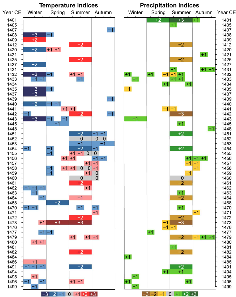
Figure 2. Monthly and seasonal temperature and precipitation indices reconstructed from Czech documentary evidence for the 15th century.
