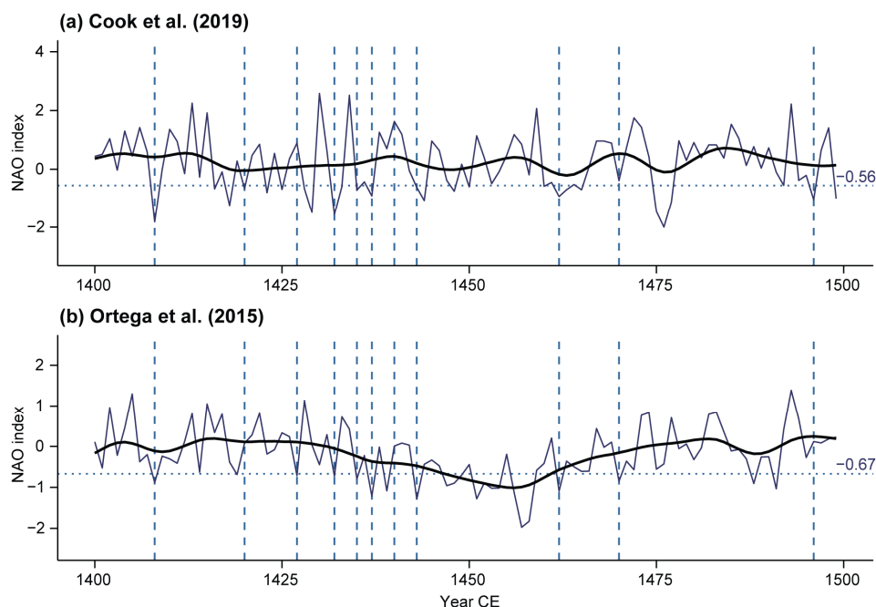
560 Figure A2. North Atlantic Oscillation (NAO) reconstructions by (a) Cook et al. (2019) and (b) Ortega et al. (2015) for the 15th century. Smoothed by a 10-year Gaussian filter. Vertical dashed lines denote cold winters according to the Czech documentary indices. Horizontal dotted lines show the mean NAO index during the cold winters ( -0.56 for Cook et al., 2019 and -0.67 for Ortega et al., 2015).
