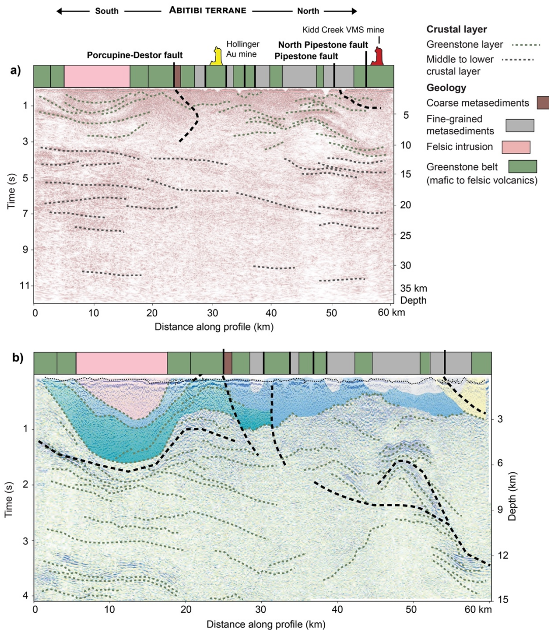
295 Figure 8. Deep seismic reflection section across the Porcupine–Destor fault zone and Timmins gold camp of the Abitibi terrane: the Metal Earth South Timmins transect (Fig. 1). Line located in Fig. 6. (a) Strip geology and interpreted seismic reflection section (Simmons et al., 2024; Adetunji et al., 2025); and (b) detailed (note vertical exaggeration) interpreted seismic reflection section of upper crust (Snyder et al., 2008). This section illustrates strongly layered reflectors (dotted black form lines) throughout much of the (middle) crustal layer beneath thrust and fold belt greenstones. This interpretation differs from Adetunji et al. (2025) because of the additional consideration of local 3-D structure in the near-surface gleaned from confidential mine observations. 300
