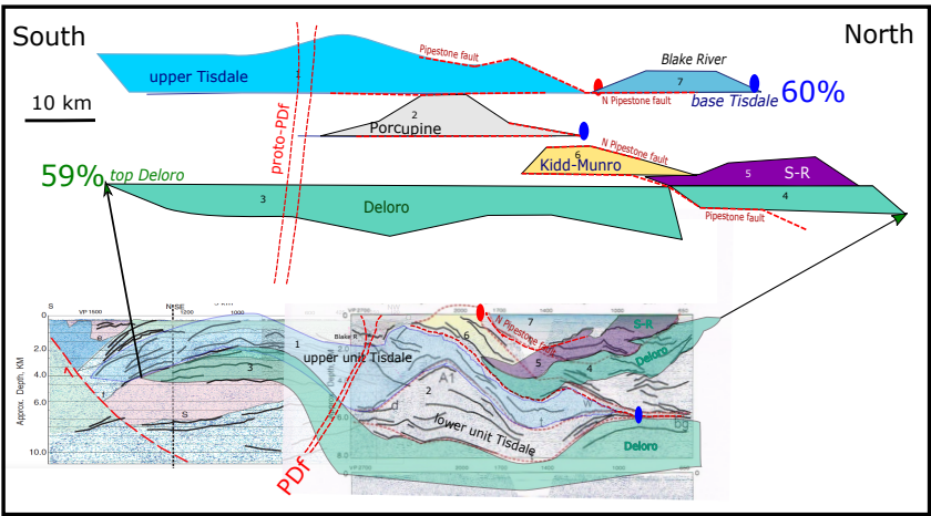
Figure 7. Crawchest geologic cross section: palinspastically restored (a) and interpreted (b) based primarily on Snyder et al. (2008) with their seismic sections shown. Corresponding assemblage names (e.g., Tisdale), numbered tectonic blocks (e.g., 2) and piercing points (upright blue ovals) indicated in both a and b. Estimated horizontal lengths at two assemblage contacts indicate final length has about 60% of the length of the original. PDF is the Porcupine–Destor fault zone.
