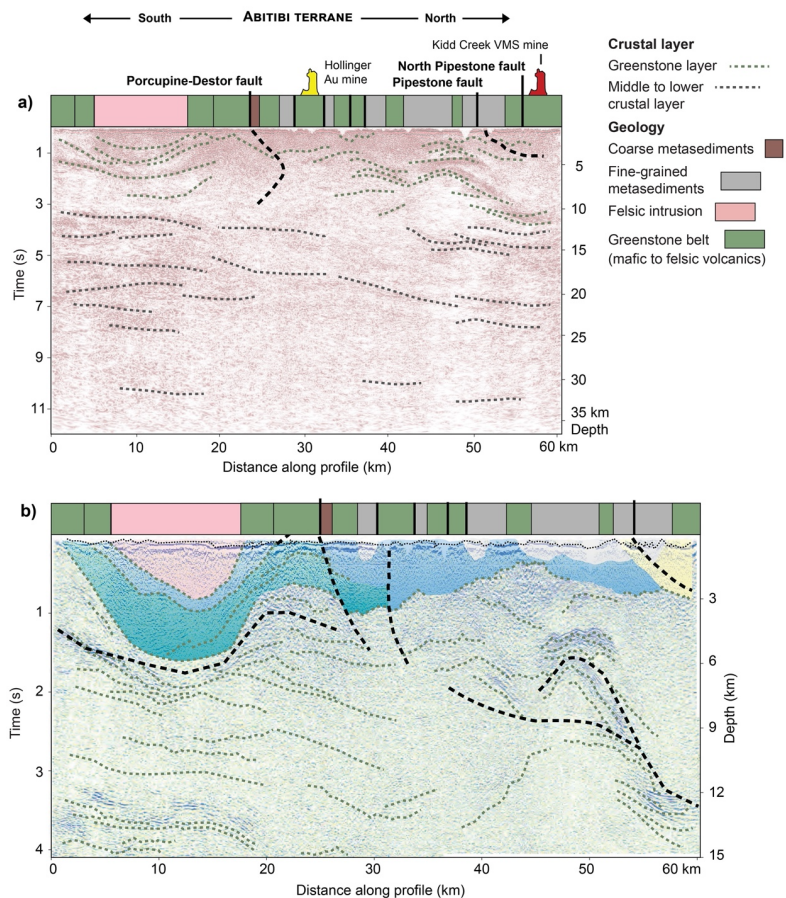
330 Figure 8. Deep seismic reflection section across the Porcupine–Destor fault zone and Timmins gold camp of the Abitibi terrane: the Metal Earth South Timmins transect (Fig. 1). Line located in Fig. 6. (a) Strip geology and interpreted seismic reflection section (Simmons et al., 2024; Adetunji et al., 2025); and (b) detailed (note vertical exaggeration) interpreted seismic reflection section of upper crust (Snyder et al., 2008). This section illustrates strongly layered reflectors (dotted black form lines) throughout much of the (middle) crustal layer beneath thrust and fold belt greenstones. This interpretation differs from Adetunji et al. (2025) because 335 of the additional consideration of local 3-D structure in the near-surface gleaned from confidential mine observations.
