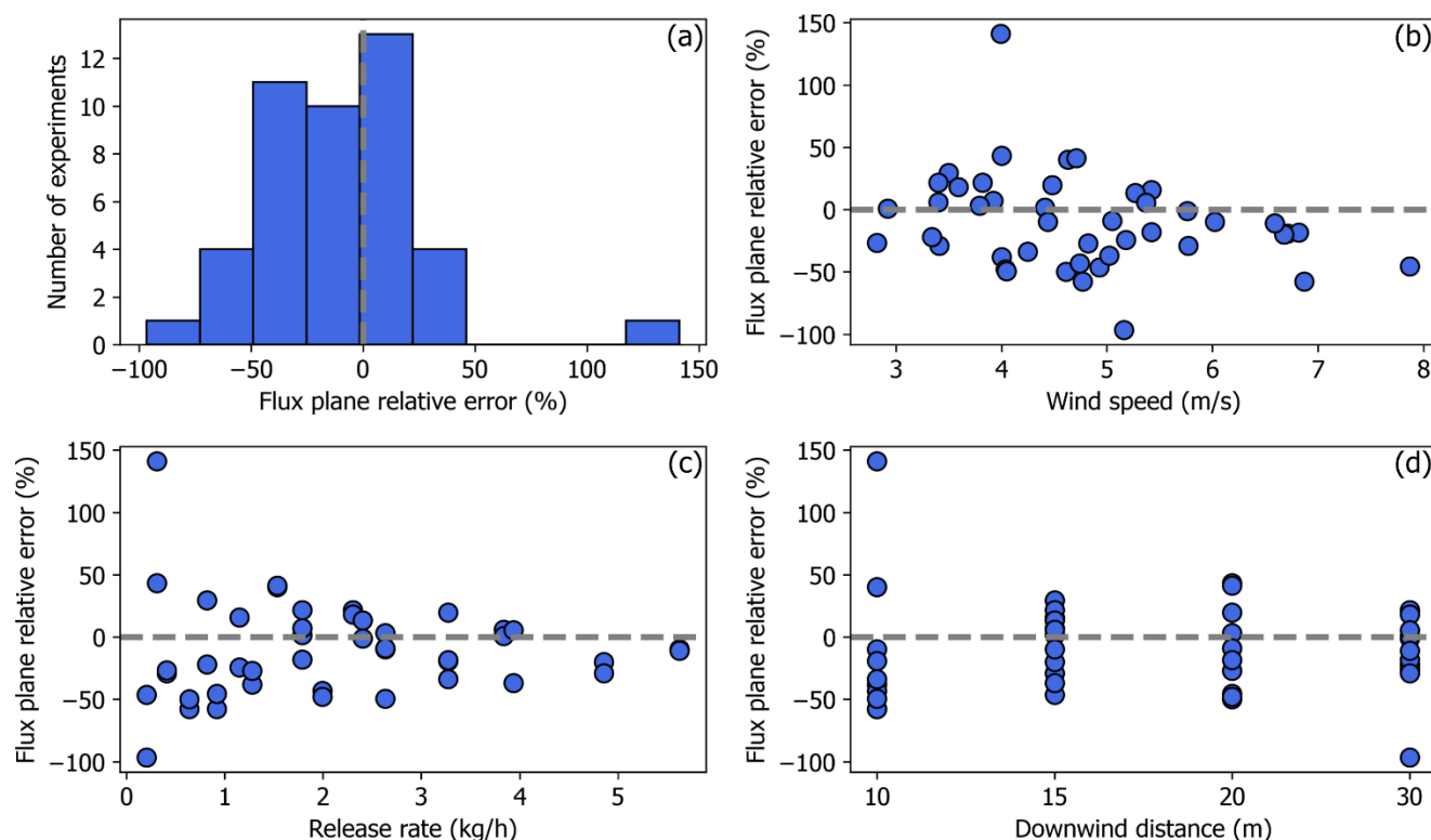
Figure 8. (a) Percent relative error distribution of the \text{CH}_4 release rates quantified with the flux plane method. (b), (c), and (d): percent relative error as a function of wind speed, release rate, and downwind measurement distance, respectively.
