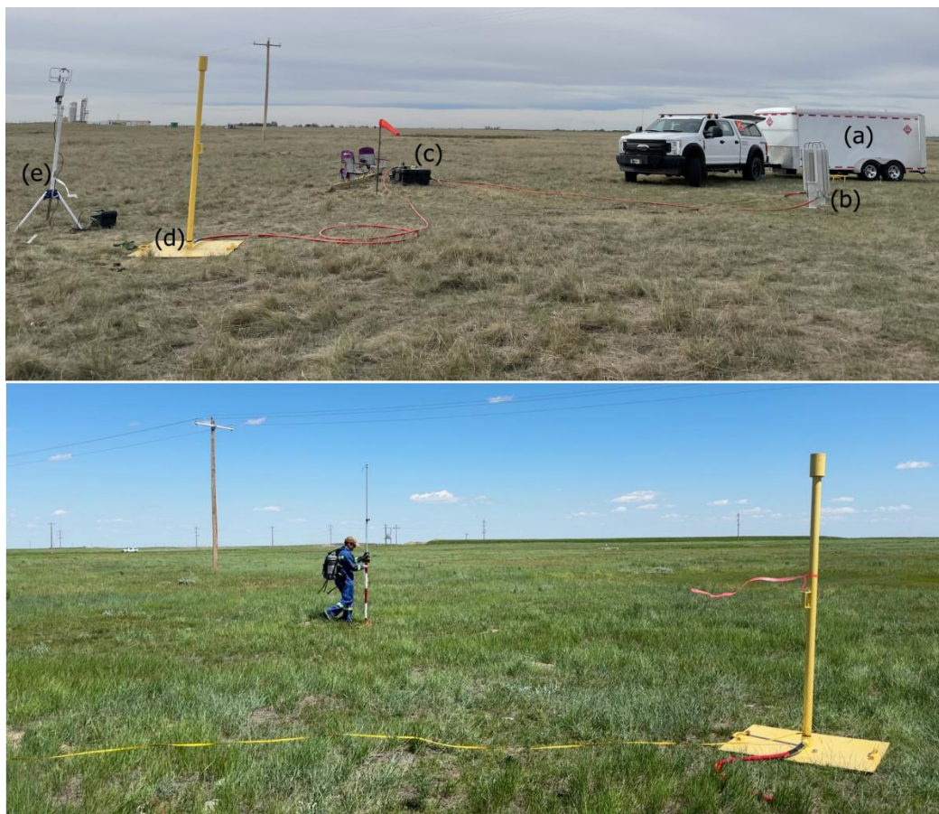
120 Figure 1. Top panel—Controlled release setup. (a) CNG trailer with tanks. (b) ambient heat exchanger. (c) flow controller. (d) release 125 stack. (e) anemometer. Bottom panel—the pole-based measurement system in operation during a controlled release test on 12 June 130 2024. The operator carried a CH 4 sensor in a backpack harness and a long length of hose was run from the sensor's inlet to the end of the pole where air was drawn in. Photo credits Zhenyu Xing and Chris Hugenholtz.
