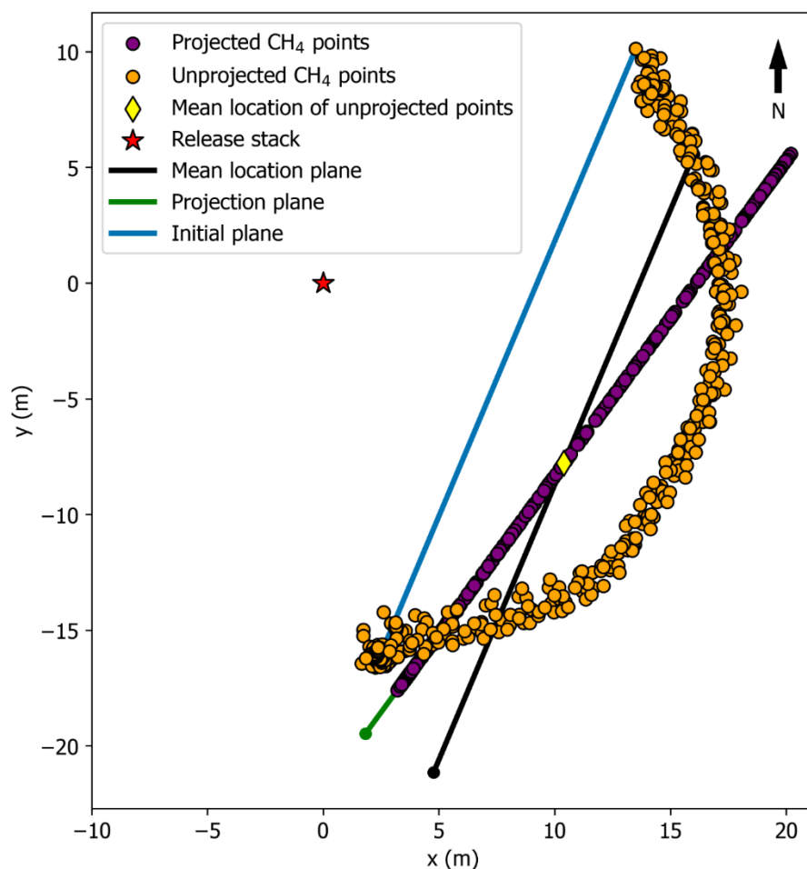
225 Figure 3. Flux plane definition and projection of CH 4 measurement points within a cartesian coordinate system for a 2.4 kg CH 4 /h release on 12 June 2024 ~15m downwind. See the associated description of the procedure to define the flux plane and project the data in the text.
