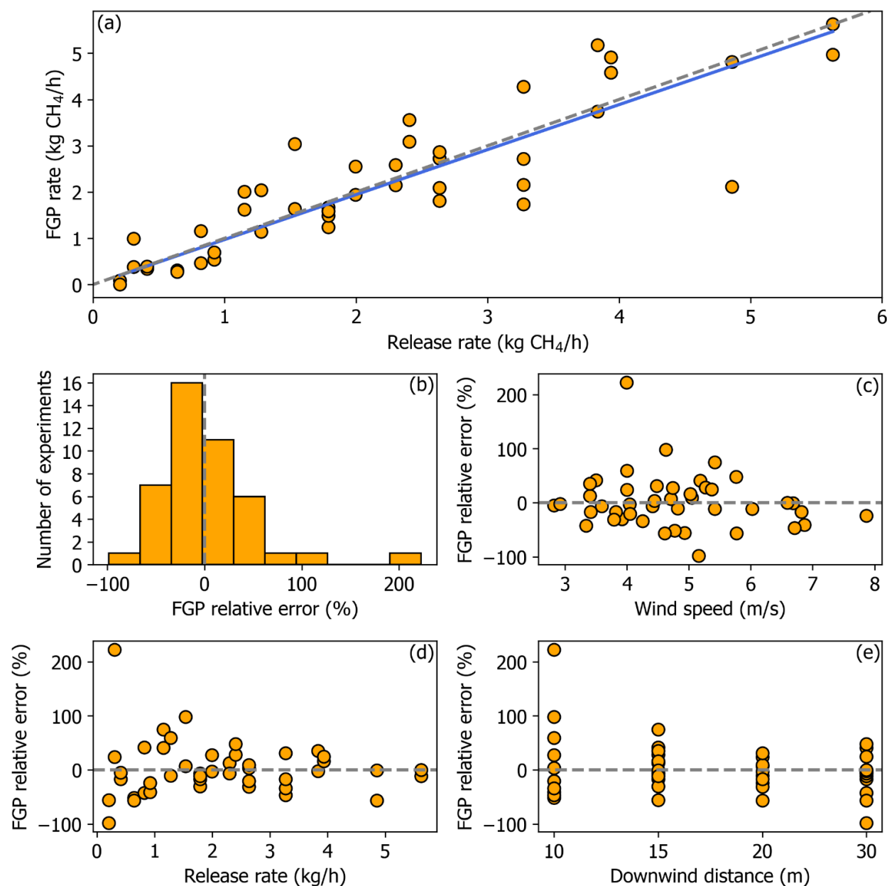
455 Figure 9. (a) Ordinary Least Squares (OLS) regression of optimized forward Gaussian plume (FGP) model estimated CH 4 emissions rates on the release rates. The blue line shows the model fit and the grey dashed line is 1:1. (b) percent relative error distribution of the CH 4 release rates quantified with the forward Gaussian optimization method. (c), (d), and (e): percent relative error as a function of wind speed, release rate, and downwind measurement distance, respectively.
