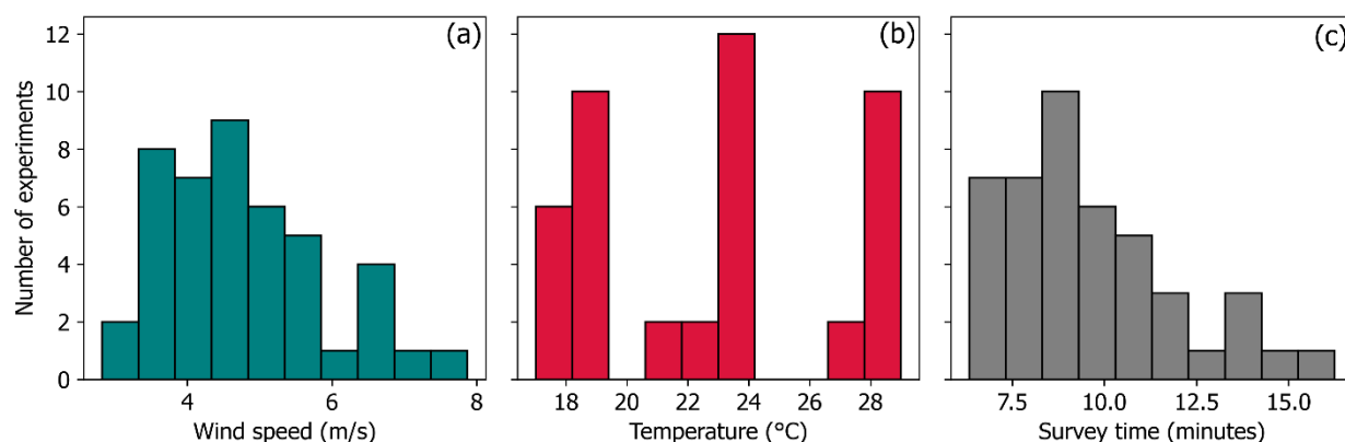
410 Figure 6. Envelope of testing conditions for controlled release experiments on 11, 12 of June and 6 of August 2024. (a) wind speed, (b) temperature, and (c) survey time. Temperature data was acquired from the ECCC weather station for Brooks, AB (WMO ID: 71457).
