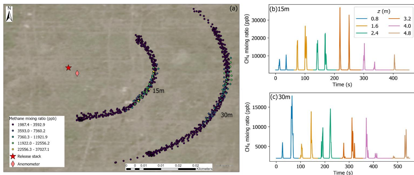
Figure 2. (a) semi-circle transects walked with the backpack-mounted CH 4 sensor and telescoping pole at 15 m and 30 m downwind of the controlled release stack during a release of 2.4 kg CH 4 /h on 12 June 2024. Circle colors correspond to CH 4 mixing ratios in the legend. (b) and (c) CH 4 mixing ratios by measurement height during the experiments at 15m and 30m downwind distances. The legend in (b) corresponds to measurement height by color in (b) and (c) . Each group of two peaks corresponds to two passes of the plume at a single measurement level. Low or no visible enhancements towards the end of the experiments at higher measurement heights suggests the highest measurement heights captured the vertical extent of the plume.
