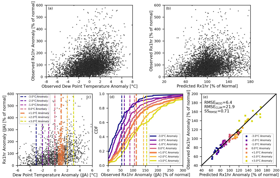
Figure 6. (a) plots the relationship between the normalized average monthly dew point temperature (our predictor) and normalized Rx1hr (our predictand) for all stations and all months. (b) plots the individual cross-validated predictions of Rx1hr versus observed Rx1hr using the normalized data model with a spatial extent of 100 km and a 3-month temporal window. In (a), our predictor corresponds to the x-axis, while in (b) our cross-validated predictions corresponds to the x-axis. The values along the y-axis of both (a) and (b) are the observed Rx1hr anomalies and they are the same in each subplot. (c) Dashed lines show the different dew point temperature anomalies over which the mean predicted versus observed Rx1hr anomalies are evaluated. This subplot shows the observed data for the 3-month window centered about July. The orange points show the distribution of Rx1hr along the y-axis corresponding to a +1^{\circ}\text{C} dew point temperature anomaly. (d) The empirical CDFs, for the different distributions corresponding to different temperature anomalies, are plotted as the lines. The dashed lines show the mean shift of the observed distributions. The thicker orange dashed line shows along the x-axis the observed mean shift in Rx1hr (i.e., average of orange points from (d)) given the example case of a +1^{\circ}\text{C} dew point temperature anomaly. (e) plots all of the seven predicted mean versus observed mean Rx1hr precipitation anomalies for the 12 months of the year, giving us 84 points. The larger orange diamond corresponds to the example case illustrated in (d) and (e).
