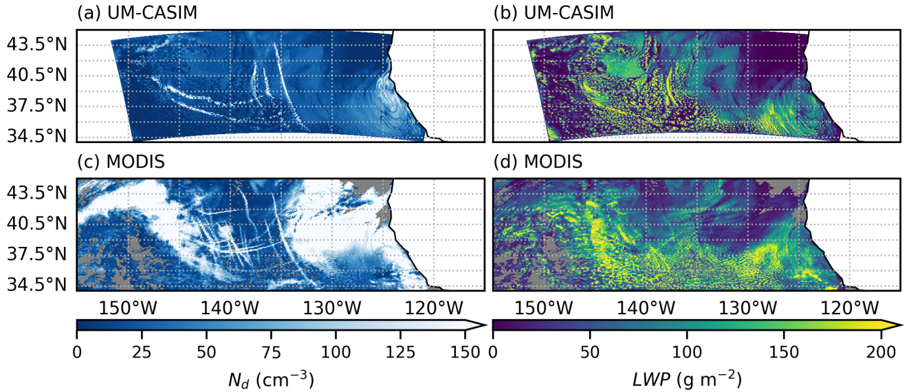
Figure 7. Modelled and Observed N_d and LWP for 12th July 2018 ship tracks. Plotted is a composite of the Aqua and Terra overpasses from Fig. 1, co-located with model nearest output time steps.
