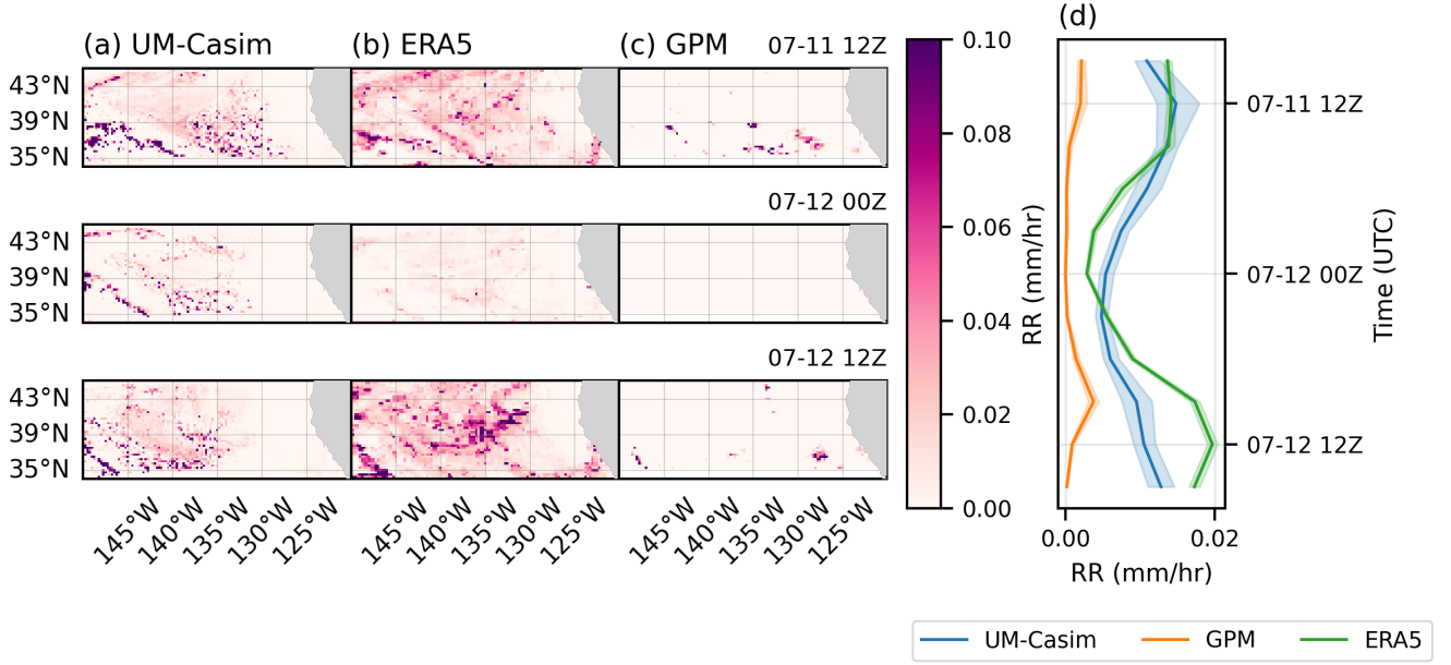
Figure 5. Evaluation of domain wide surface precipitation at 12-hourly intervals. a) UM-CASIM simulated surface precipitation (regridged to ERA5 resolution), b) ERA5 surface precipitation, c) GPM surface precipitation. d) The domain-wide mean across the simulation runtime, demonstrating the diurnal cycle.
