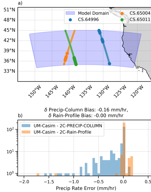
Figure 6. Evaluation of surface against CloudSat CPR products. a) Location of CloudSat overpasses during the 48 hour simulation, with bold points showing locations where surface precipitation from the 2C-Precip-Column product are greater than zero. Associated times of overpass are roughly as follows: CS.64996 at 2200Z 11th July, CS.65004 at 1200Z on 12th July, and CS.65011 at 2300Z on 12th July.
