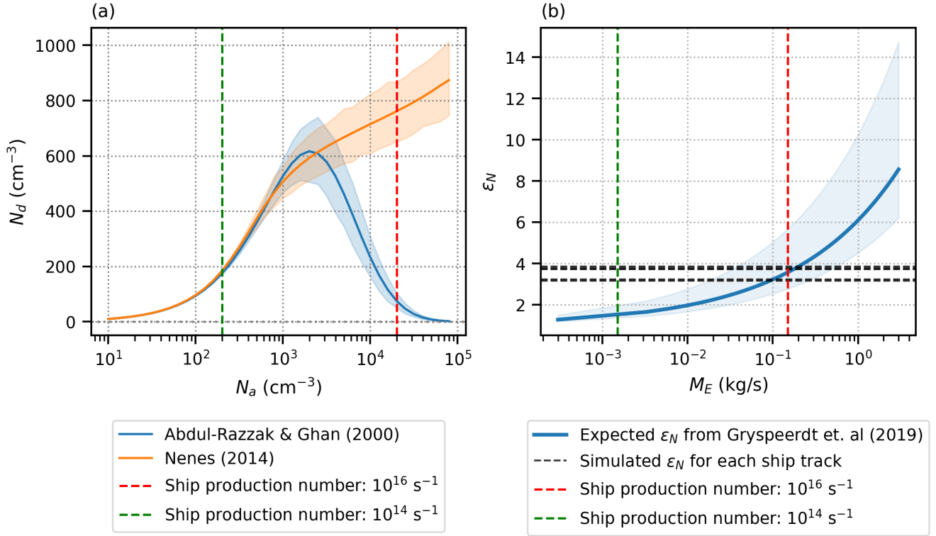
Figure 3. (a) Number of aerosol particles ( N_a ) activated to cloud droplets ( N_d ) in different activation parameterisations calculated in a simple adiabatic cloud parcel model. Confidence intervals given by the range of temperature, pressure and updrafts simulated in our case study. (b) The expected enhancement in cloud droplets ( \epsilon_N ) as a function of aerosol mass emission rate ( M_E ), based on equation (1) from Gryspeddt et al. (2019b). Vertical lines are the emissions from different ship production numbers. Horizontal lines are the enhancements produced from our simulations for each individual ship. Confidence interval is given by the range of background droplet number concentrations in our simulation.
