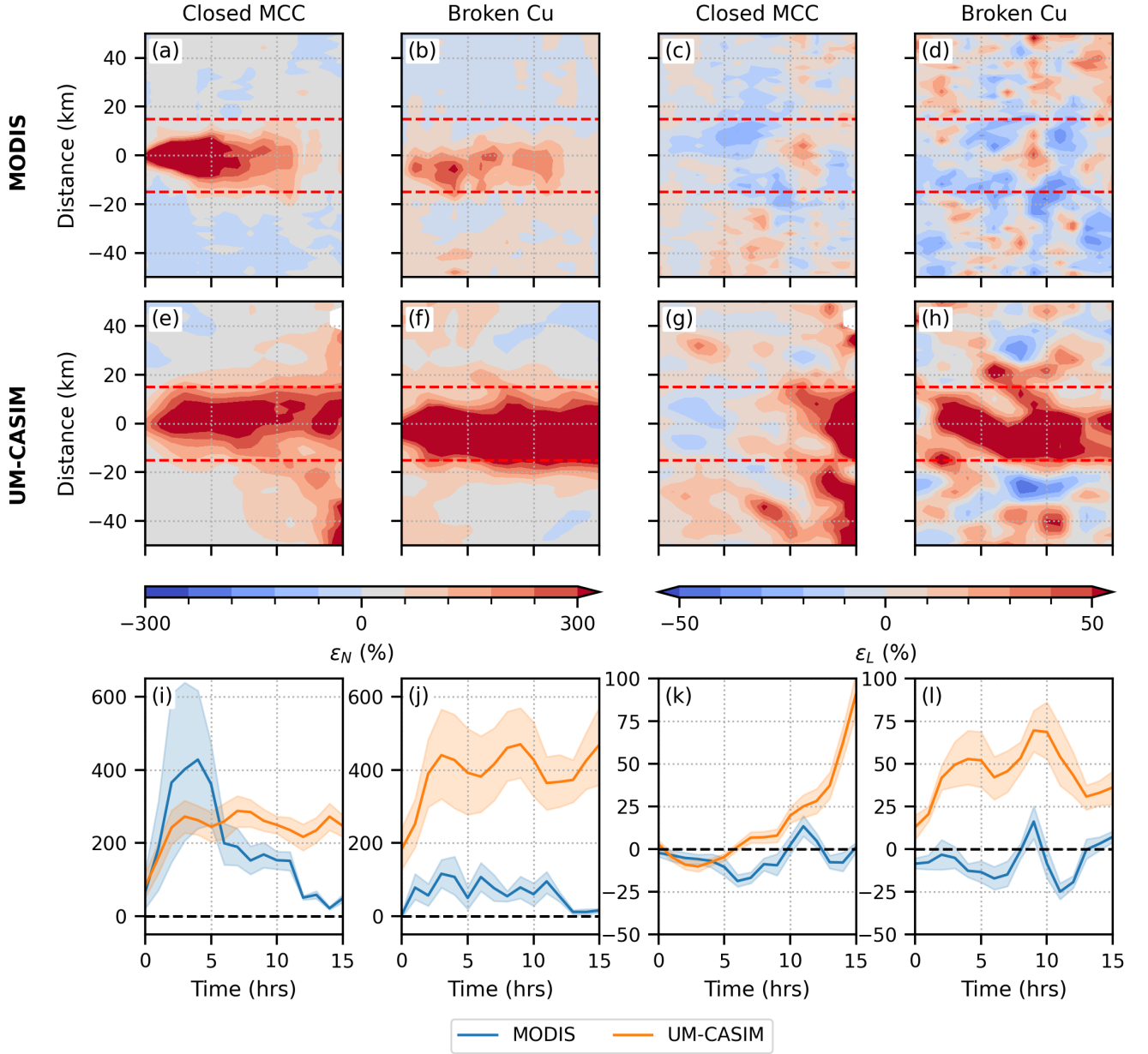
Figure 9. Percentage enhancements from the “unpolluted” references background state. (a)-(d) show observations of ship tracks in in the Eastern Pacific region of the domain (ships A-C) and the Central Pacific region (ships D & E) conditions for N_d (left) and LWP (right). (e)-(h) shows the same but for modelled ship tracks. (i)-(l) show the average of the “inside track” region, as defined by the red dashed lines in (a)-(h).
