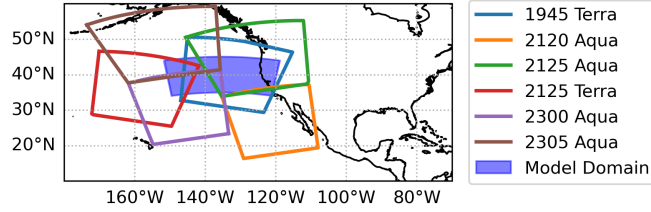
Figure 1. Granules from Aqua and Terra overpasses on 12th July 2018 that intersect with the model domain of this study.
