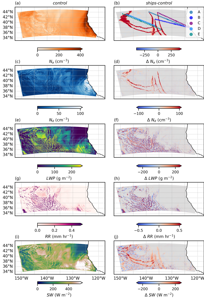
Figure 4. Left column: control simulations of 12th July 2018 at 20:00 without ship emissions turned on. Panel (b) contains the locations of the ships simulated during this study, up until the time step of this figure. Right column: difference from control for simulation with shipping emissions on. Stochastic noise between two model runs can be seen in the difference plots. Variables shown are aerosol number concentration ( N_a ), cloud droplet number concentration ( N_d ), liquid water path (LWP), surface rain rate (RR), and top of atmosphere outgoing short wave radiation (SW). N_d and N_a are mean values across model level numbers below 1km.
