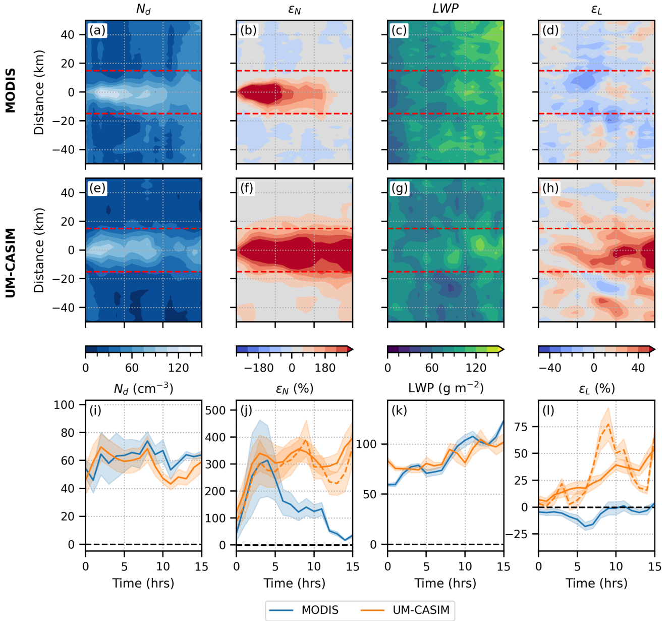
Figure 8. (a)-(d) Observed N_d and LWP across all observations of our 5 ship tracks, as well as the percentage enhancement of the “inside track” region (defined by <15 km from the centre). Percentage enhancement is calculated from the mean of the region between 30-45 km away from the centre of the track. (e)-(h) The same as above, but for modelled ship tracks. The percentage enhancement is instead calculated as the percentage change from the control model run (solid orange line). Percentage enhancement using the lateral offset method (as in the observations) is shown in the orange dashed line. (i)-(j) Mean of the observed and modelled N_d in-track values, and enhancements, in the “inside track” region. (k)-(l) The same, but for LWP. Whilst inside-track values for both N_d and LWP are similar between observations and model output, enhancements vary significantly.
