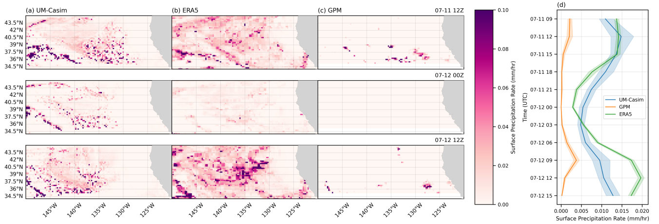
Figure 5. Evaluation of domain wide surface precipitation at 12-hourly intervals. a) UM-CASIM simulated surface precipitation (regrided to ERA5 resolution), b) ERA5 surface precipitation, c) GPM surface precipitation. d) The domain-wide mean across the simulation runtime, demonstrating the diurnal cycle.
