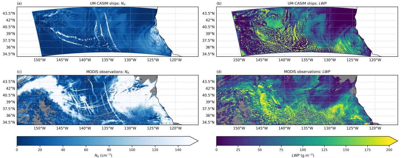
Figure 7. Modelled and Observed N_d and LWP for 12th July 2018 ship tracks. Plotted is a composite of the Aqua and Terra overpasses from Fig. 1, co-located with model nearest output time steps.
