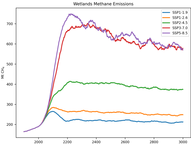
Figure A1. 50-year running mean of Wetland methane emissions, reproduced from Figure 2 in Kleinen et al. (2021a).
