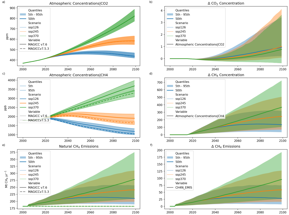
Figure 1. Left column: Comparisons of the atmospheric CO 2 and CH 4 concentrations and natural CH 4 emissions between MAGICC v7.5.3 (dashed lines) and v7.6 (solid lines) for three SSP scenarios. Right column: The differences between versions in concentrations of CO 2 and CH 4 and natural emissions of CH 4 . As the older version of MAGICC held natural methane sources constant, it has a flat line in the emissions plot. The 5 th and 95 th quantiles are shown for all. In sub-figure a , the difference in atmospheric CO 2 is so small that the change in median and the upper and lower quantiles is not visible here. In e , natural methane in v7.5.3 has no quantiles as these were constant in all scenarios. And in c , the lower and upper quantile boundaries are indicated with thinner lines than the median (solid for v7.6, dashed for v7.5.3), and slight overlap between the lowest quantiles of v7.6 and the highest of v7.5.3 can be seen where the filled-in colour is darker.
