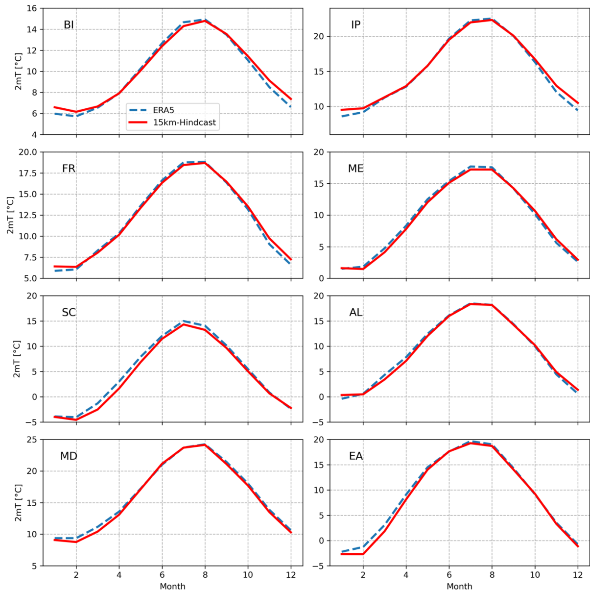
200 Figure 2: Seasonal cycle of the T_{2m} ( ^{\circ}\text{C} ) on the Prudence subdomains: ERA5 reanalyses (blue dashed line), 15-Hindcast simulation (red solid line).
