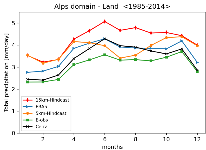
Figure 5: Seasonal variability of P over the Alps domain (AL) averaged over land only. Experiments 15km-Hindcast (red/diamonds), 5km-Hindcast (orange/dots). Reference datasets: ERA5 (blue/arrows), E-OBS (green/squares), CERRA (black/crosses)
