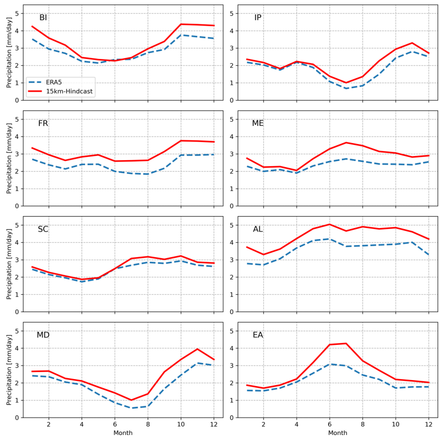
Figure 3: Seasonal cycle of the total precipitation P(\text{mm/day}) on the Prudence subdomains: driving ERA5 reanalysis (blue dashed line ), hindcast simulation 15Km-Hindcast (red solid line ).
