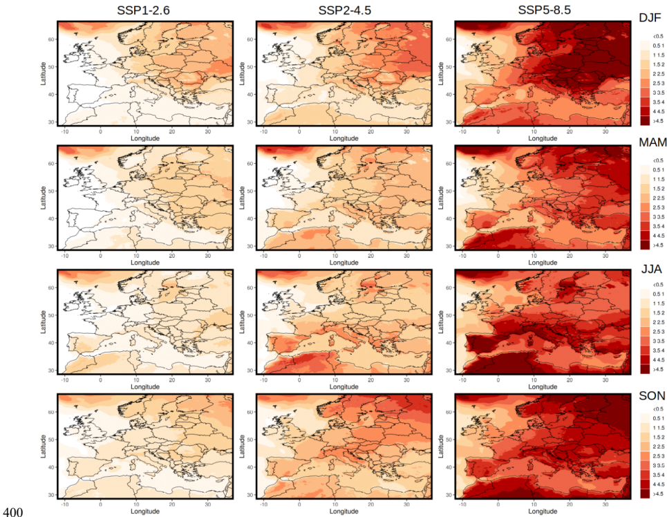
Figure 12: Projections of temperature change at the end of the century in the multi-scenario experiments – 15km SSPs (°C)
