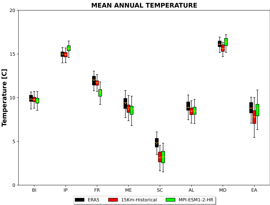
Figure 10: Box plot of historical simulation of T2m: mean (yellow points), median (orange lines within the box), 1 st -3 rd interquartile range (IQR, color box). The whiskers extend from the box to the farthest data point lying within 1.5x the inter-quartile range (IQR) from the box. 15km-Historical experiment (red), ERA5 (black), GCM (green).
