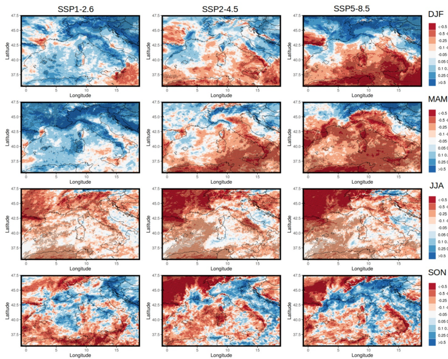
435 Figure 15: Projections of precipitation change at the end of the century in the multi-scenario experiments 5km-SSPs_ (mm/day)
