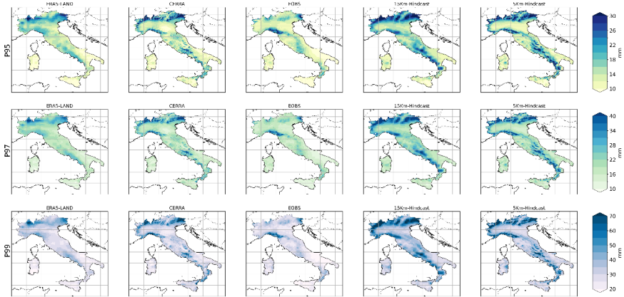
Figure 9 Annual P95 (top), P97 (mid), and P99 (bottom) of daily rainfall from ERA5-LAND, CERRA, E-OBS and the simulations 15Km-Hindcast and 5Km-Hindcast.
