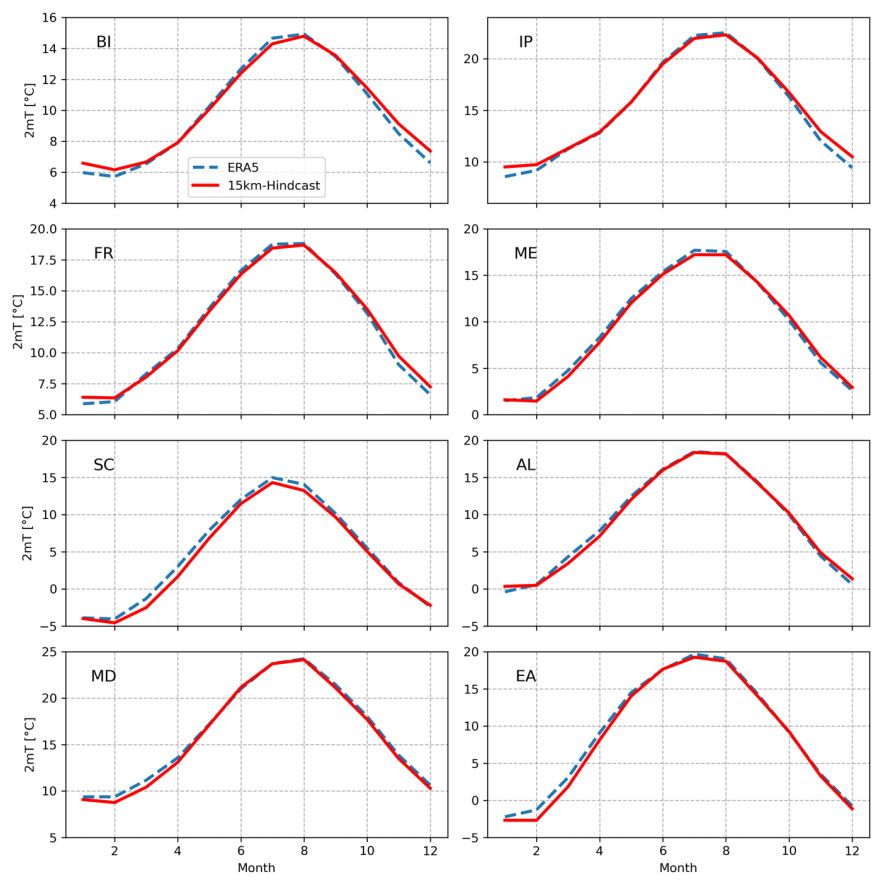
Figure 2: Seasonal cycle of the T2m(°C) on the Prudence subdomains: ERA5 reanalyses (blue dashed line), 15-Hindcast simulation (red solid line).
