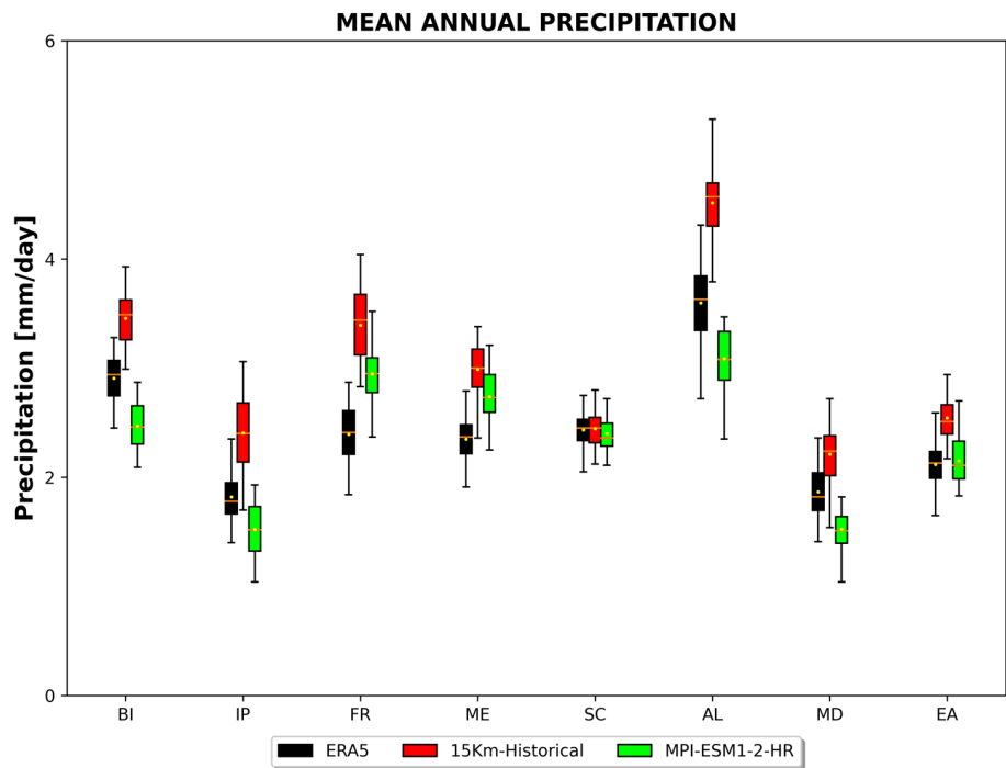
Figure 11: Same as Figure 10 but for mean precipitation.
