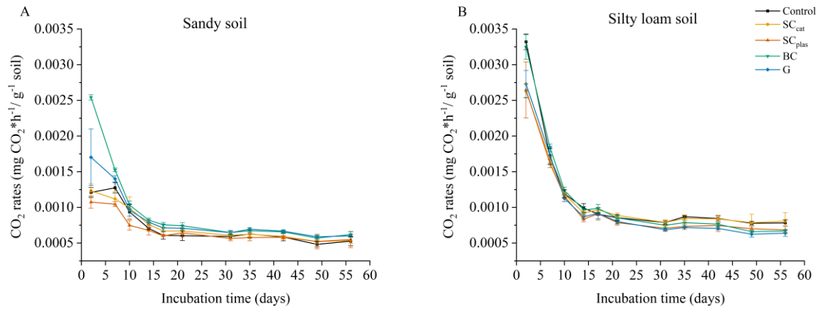
Figure S1 CO 2 production rates evolved during 56 days of incubation after addition of 40 t ha -1 test material (mean and standard error, n = 4). Treatments were C: control, SC cat : solid carbon from catalytic pyrolysis, SC plas : solid carbon plasma pyrolysis, BC: Biochar, and G: Graphite.
