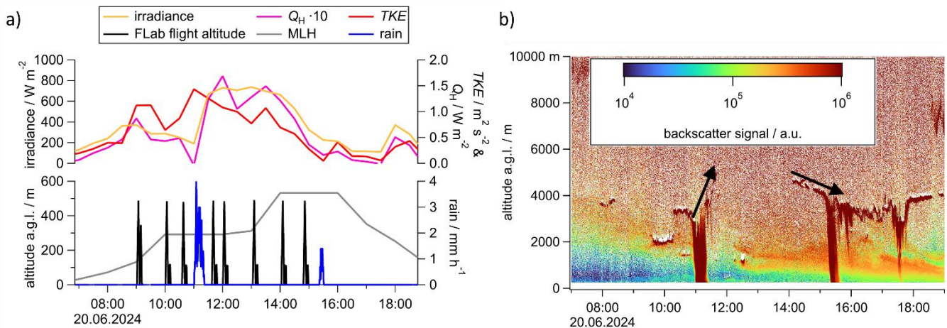
Figure 2: a) Temporal development of the ground-based measured irradiance (orange), the turbulent kinetic energy ( TKE , red), the sensible heat flux ( Q_H , pink, all 30 min averages, multiplied by a factor of 10 for better visibility) and precipitation (blue) throughout the day. The hourly mixing layer height (ICON model MLH, gray) increase during the daytime, so that the FLab (flight track, black, 1 s data) was measuring below and aloft the MLH depending on the daytime. b) The ceilometer in MoLa monitors an uplift of clouds (dark red) from 3 km to 5 km immediately after the rainfall at 11:00 and a later decrease of layers before the second rainfall (red color reaching ground level indicates precipitation). Data of the lowermost 200 m were removed due to high uncertainties.
