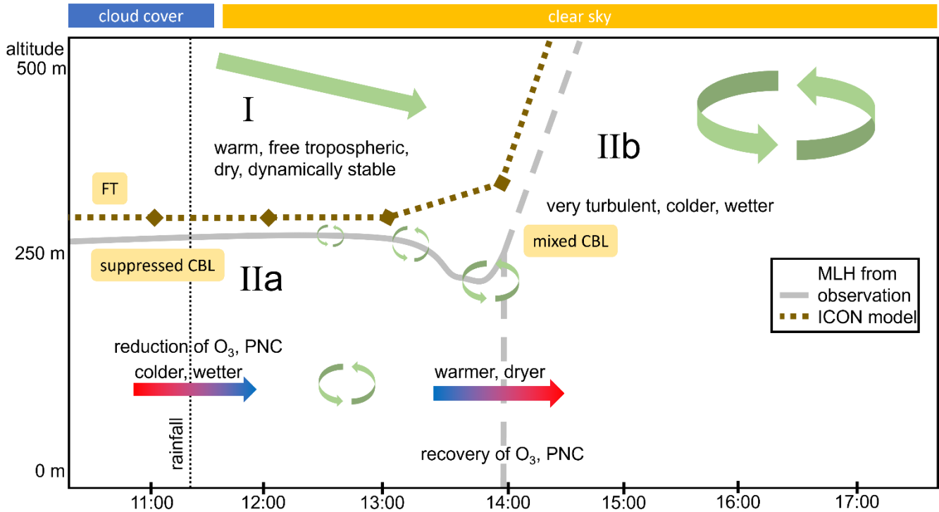
Figure 1: A reconstruction of different characteristics and dynamics of the air masses (I, IIa and IIb, separated by grey lines) observed before and after the rainfall event. The estimated MLH from the ICON model is presented in olive with markers indicating hourly time stamps and lines between the data points to guide the eyes. Greenish arrows represent dynamic processes, multi-colored arrows thermal processes.
