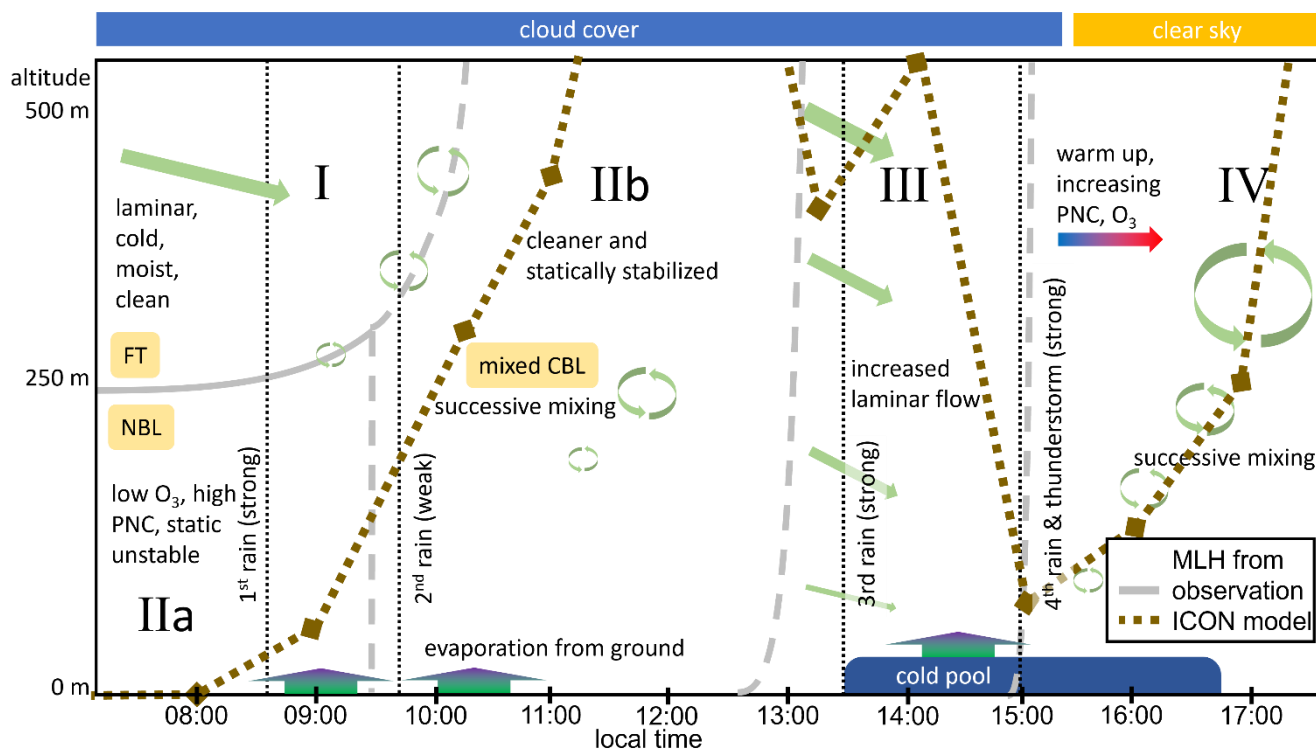
295 Figure 5: A reconstruction of different characteristics and dynamics of the air masses (I, IIa, IIb, III, and IV, separated by grey lines; solid line illustrates stratification, dashed lines transition periods) on 12 August 2023. The estimated MLH from the ICON model (1-h resolution) is presented in olive with dashed lines between the data points to guide the eye. Greenish arrows display dynamic processes, multi-colored arrows thermal processes.
