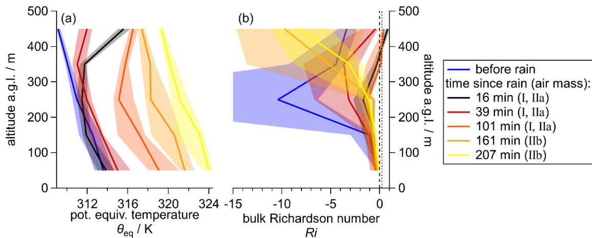
235 Figure 3: The gradient of the equivalent potential temperature d\theta_{eq}/dz (a) indicates unstable conditions throughout the day below 300 m, while the air mass above 300 m is stabilized after the rain at 11:00. The bulk Richardson number Ri (right) is consistent with a successive destabilization after the rain and indicates a stratification between 200 m and 300 m before the rain. The solid traces show the median and the shaded area is the interquartile range of the binned data. Dashed lines indicate Ri = 0 and Ri = 0.25 .
