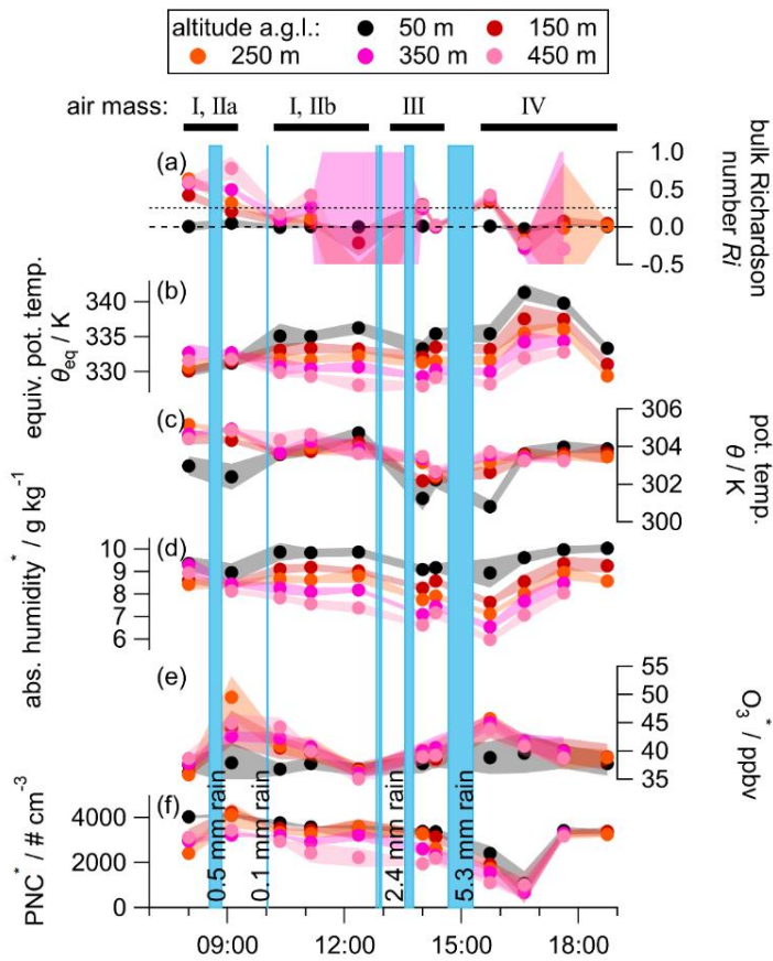
Figure 7: Development of medians of 100 m altitude increments of the bulk Richardson number Ri (a), equivalent potential temperature \theta_{eq} (b), potential temperature \theta (c), absolute humidity (d), O_3 mixing ratio (e), and the particle number concentration (PNC, f) with time on 12 August 2023. Variables marked with * are corrected for temporal variation using the corresponding MoLa data. Error bars are derived from interquartile ranges. Dotted lines indicate Ri = 0 and Ri = 0.25 . Rainfall periods are marked in blue with the amount of rain noted (precipitation at 13:00 and 14:00 were summed).
