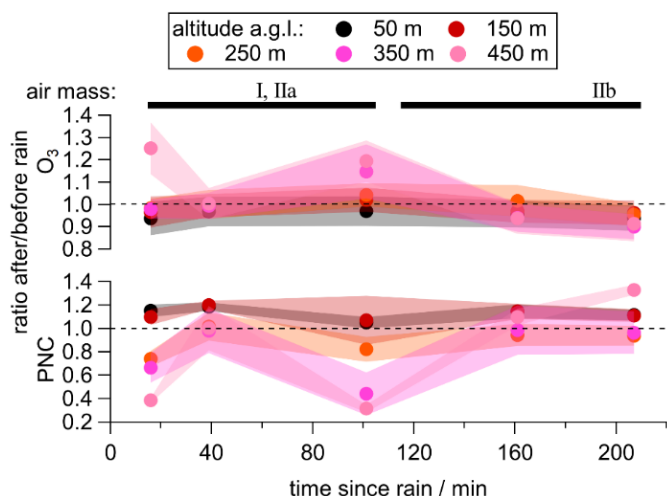
Figure 4: The ratios of the O 3 mixing ratio (top) and the particle number concentrations PNC (bottom) after to before the rainfall (at 11:00) were calculated for different altitude increments (color-scale) for five vertical profiles measured at different times after the rain. Error bars represent the combined standard error of flights before and after the rain. Attributed air masses that are identified within a flight are indicated at the top of the graph.
