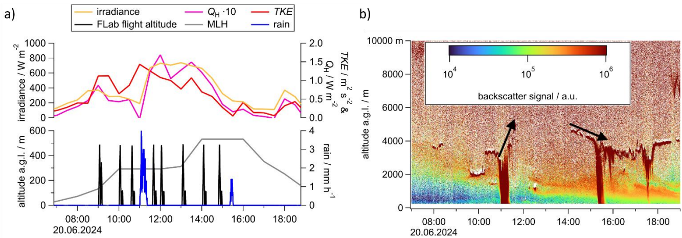
185 Figure 2: a) Temporal development of the ground-based measured irradiance (orange), the turbulent kinetic energy ( TKE , red), the sensible heat flux (pink, all 30 min averages, multiplied by a factor of 10 for better visibility) and precipitation (blue) throughout the day. The hourly mixing layer height (ICON model MLH, gray) increase during the daytime, so that the FLab (flight track, black, 1 s data) was measuring below and aloft the MLH depending on the daytime. b) The ceilometer in MoLa monitors an uplift of clouds (dark red) from 3 km to 5 km immediately after the rainfall at 11:00 and a later decrease of layers before the second rainfall (red color reaching ground level indicates precipitation). Data of the lowermost 200 m were removed due to high uncertainties. 190
