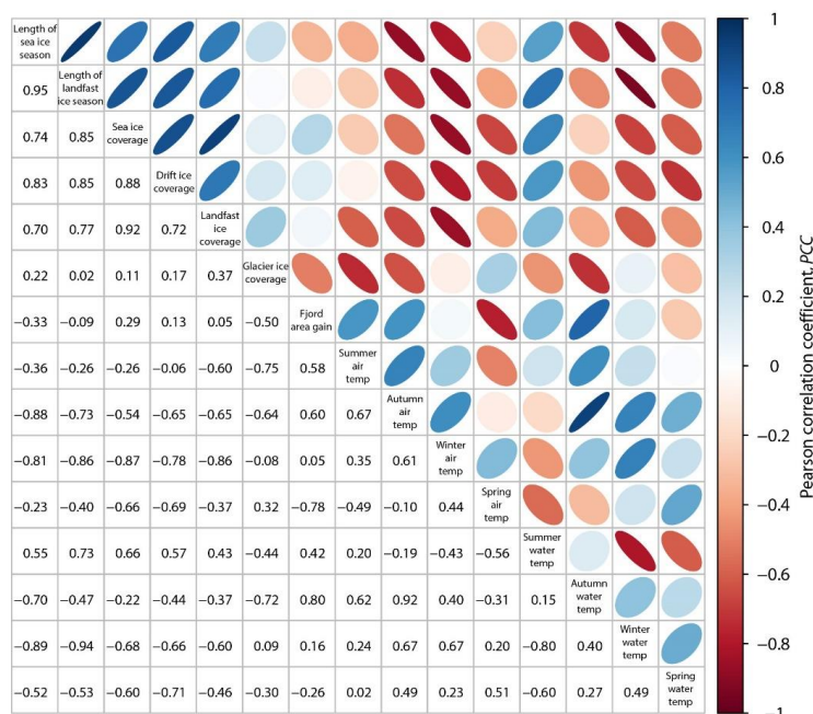
Figure 15. Relationships between ice parameters and environmental forcings. Temperatures refer to the mean monthly for July-September (summer), October-December (autumn), January-March (winter) and April-June (spring). For the values and units see Tables 2, 5, 6 and 7.
