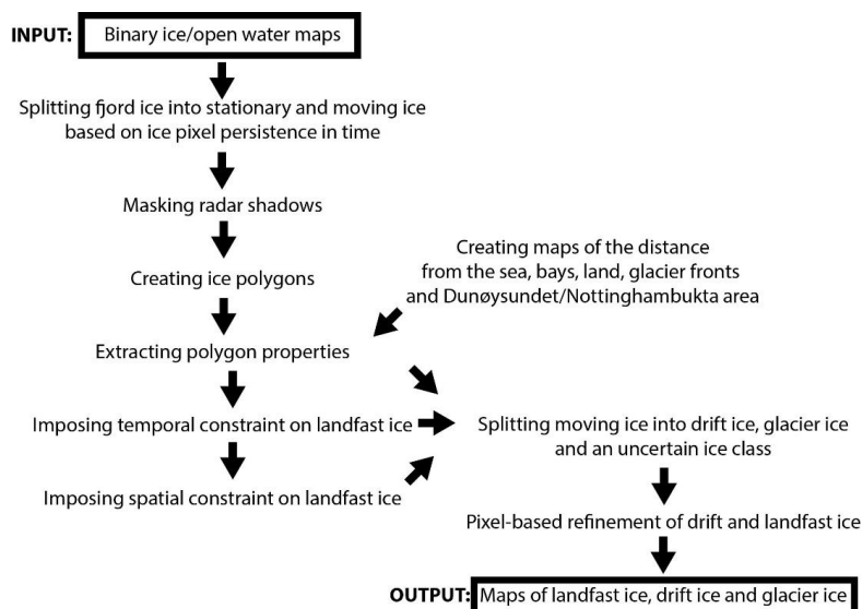
Figure 3. Fjord ice type separation workflow.
