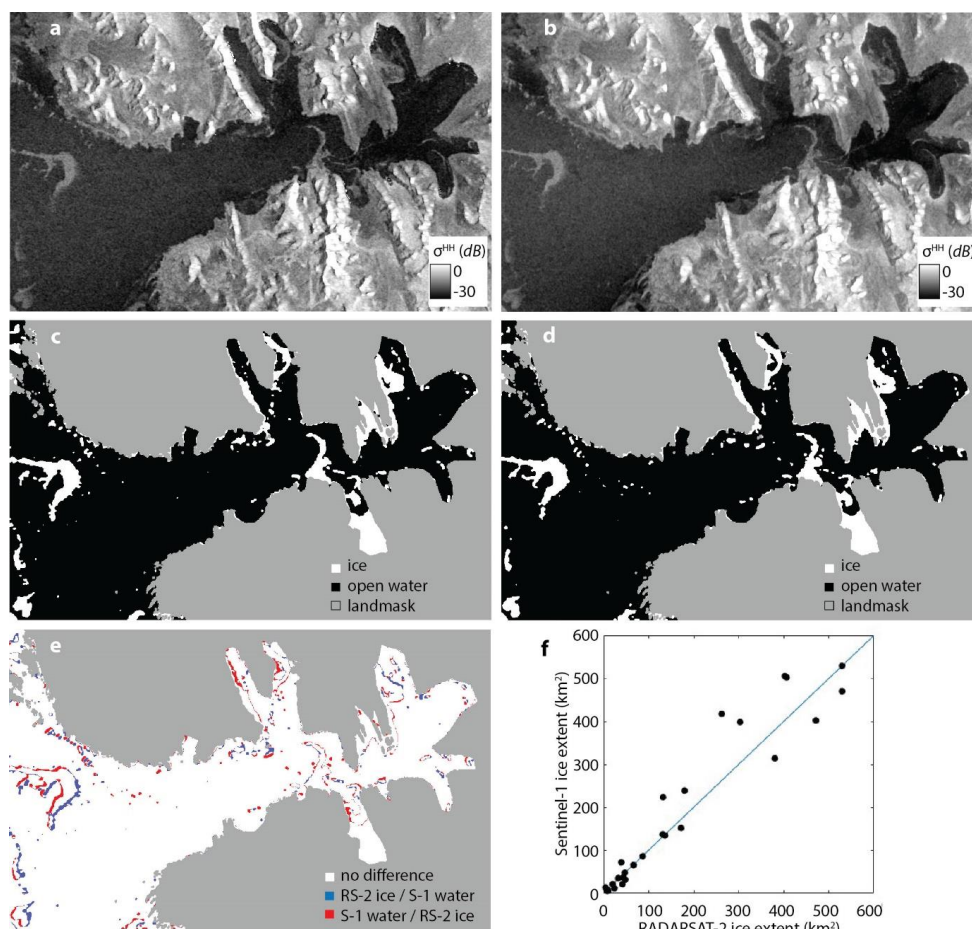
150 Figure 2. Inter-sensor comparison of fjord ice mapping: a) RADARSAT-2 (RS-2) scene RS2_SCWA_20150105_053323_DES_152, b) Sentinel-1 (S-1) scene S1_EWM_20150105_054924_DES_110, c) RS-2 binary map, d) S-1 binary map, e) difference map, f) fjord ice extent for the 29 overlapping dates.
