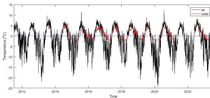
Figure 14. Time series of daily air and water temperature in Hornsund between 2011-07-01 and 2023-06-30.
