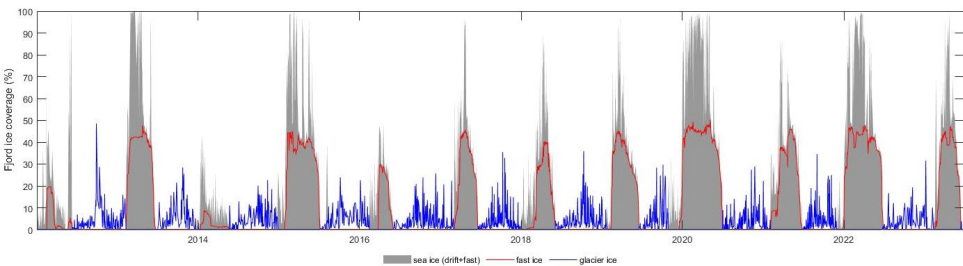
Figure 10. Time series of fjord ice coverage in Hornsund from 2012-2023.
