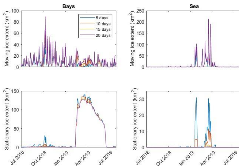
190 Figure 4. The extent of moving and stationary ice between 2018-07-01 and 2019-07-31 depending on the minimal number of consecutive days of ice presence in the bays and open sea as delimited in Fig. 1.
