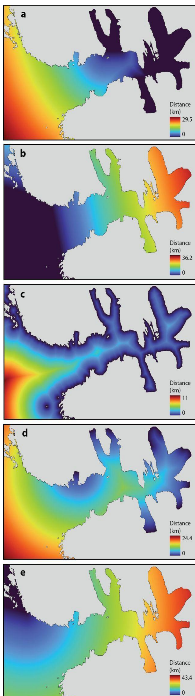
Figure 6. Maps of the distance from: a) the bays, b) the sea, c) the land, d) the glacier fronts, and e) the Dunøysundet/Nottinghambukta (DN) area as delimited in Fig. 1 for July 2018 - June 2019.
