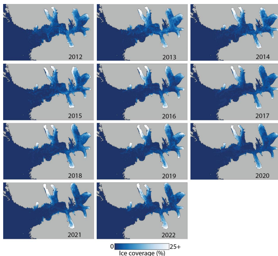
370 Figure 12. Average glacier ice presence in Hornsund for the sea-ice-free seasons 2012 to 2022 (for dates see Table 2).
