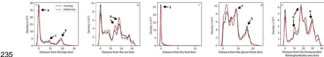
Figure 7. Kernel density distribution of the mean distance from a) the bays, b) the sea, c) the land, d) the glacier fronts, and e) the Dunøysundet/Nottinghambukta (DN) area for the moving and stationary ice polygons in 2012-2023.
