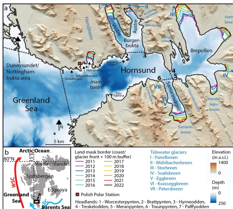
70 Figure 1. Study area: a) Hornsund, b) Svalbard. WSC - West Spitsbergen Current. SC- Sørkapp Current. DEM courtesy of the Polar Geospatial Center; bathymetry IBCAO V5.0 Grid at 100 m and Norwegian Hydrographic Service at 5 m.
