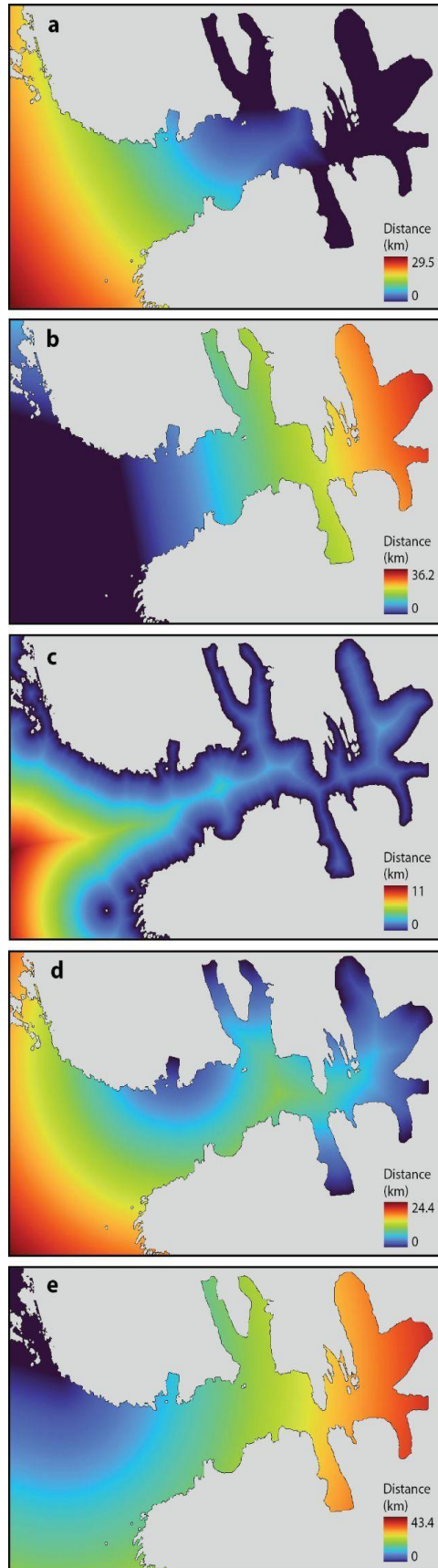
Figure 6. Maps of the aerial distance from: a) the bays, b) the sea, c) the land, d) the glacier fronts, and e) the Dunøysundet/Nottinghambukta (DN) area as delimited in Fig. 1 for July 2018 - June 2019.
