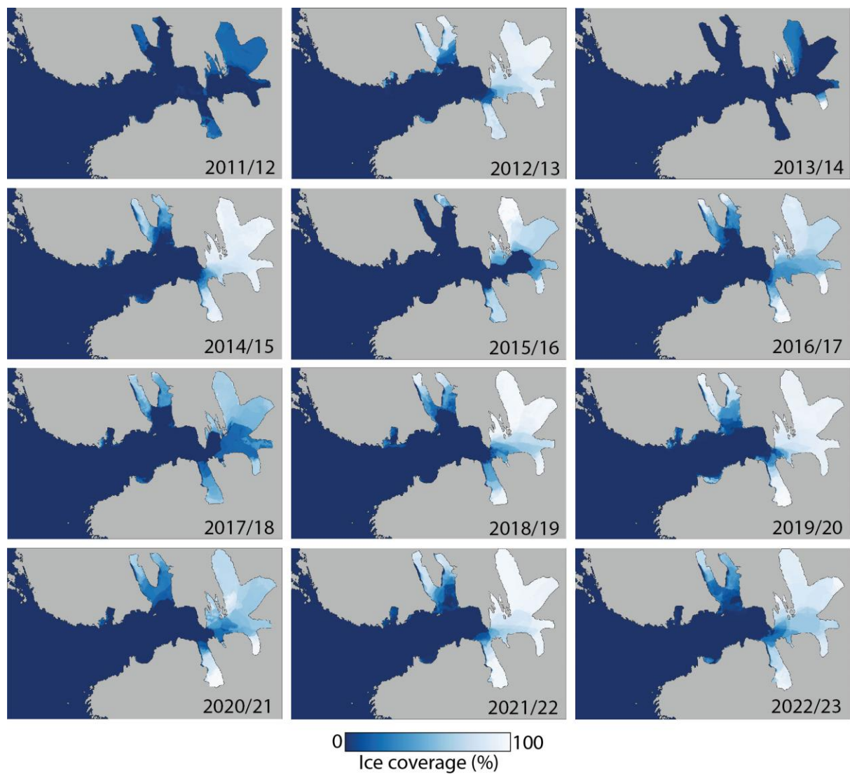
Figure 11. Average landfast ice presence in Hornsund for the landfast ice seasons 2011/12 to 2022/23 (for dates see Table 2).
