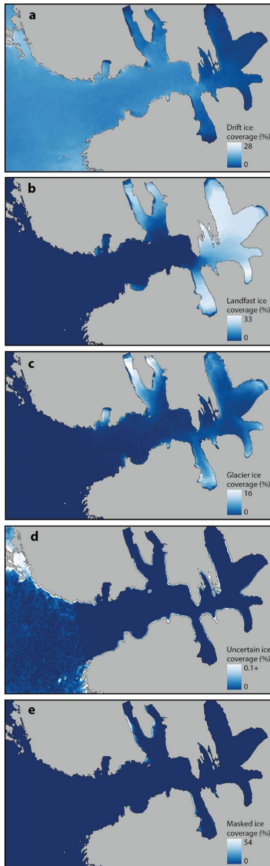
Figure 9. Average ice presence in Hornsund between 2012-01-02 and 2023-06-29: a) drift ice, b) landfast ice, c) glacier ice, d) uncertain ice, and e) masked ice.
