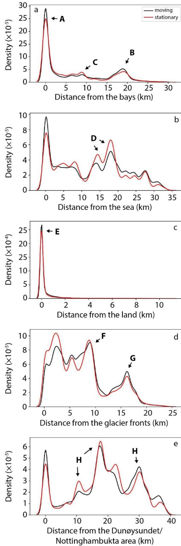
240 Figure 7. Kernel density distribution of the mean distance from a) the bays, b) the sea, c) the land, d) the glacier fronts, and e) the Dunøysundet/Nottinghambukta (DN) area for the moving and stationary ice polygons in 2012-2023.
