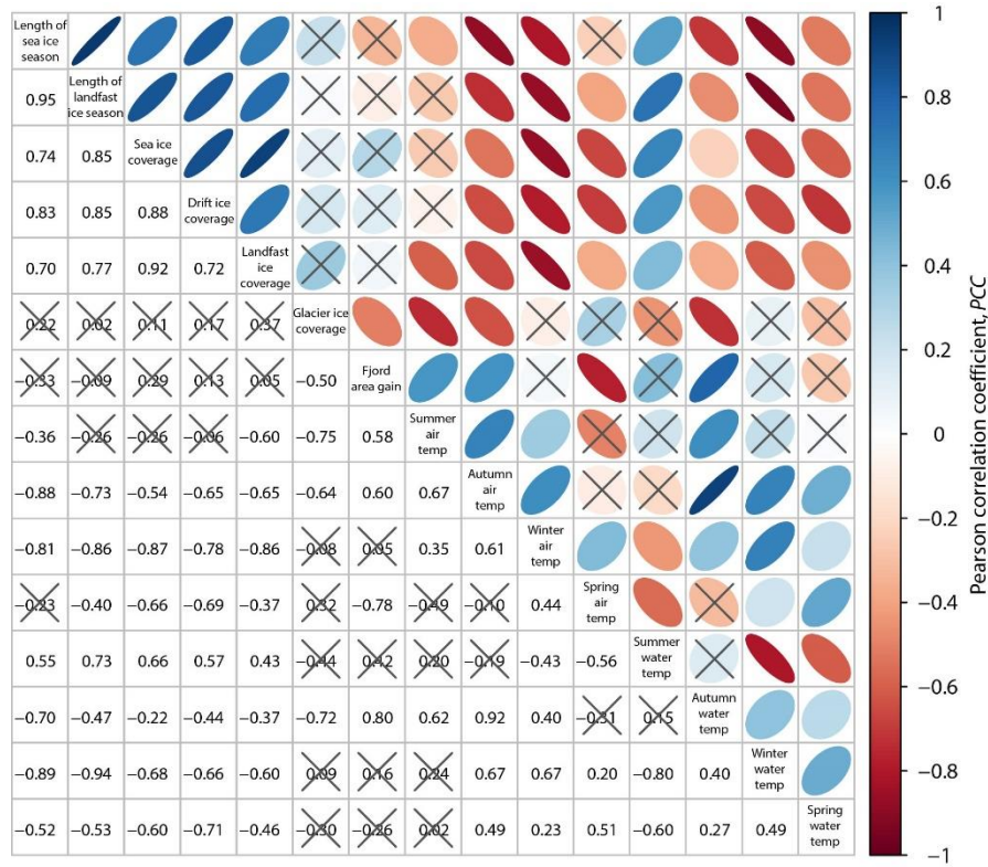
Figure 15. Matrix of correlation coefficients and best-fit ellipses for ice parameters and environmental forcings obtained for seasons with complete observations using the Pearson correlation in R. The Pearson correlation coefficient (PCC) is represented by the colour bar and describes both the strength (absolute value) and sign of relationships. Strength and sign of relationships are also represented by, respectively, width and orientation of the ellipses. Insignificant relationships ( p > 0.05 ) are crossed out. Temperatures refer to the mean monthly for July-September (summer), October-December (autumn), January-March (winter) and April-June (spring). For the values and units see Tables 2, 5, 6 and 7.
