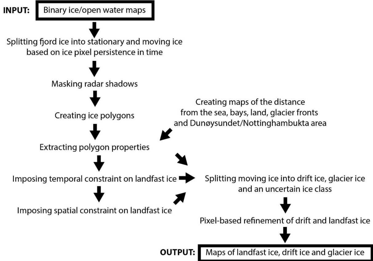
Figure 3. Fjord ice type separation workflow.
