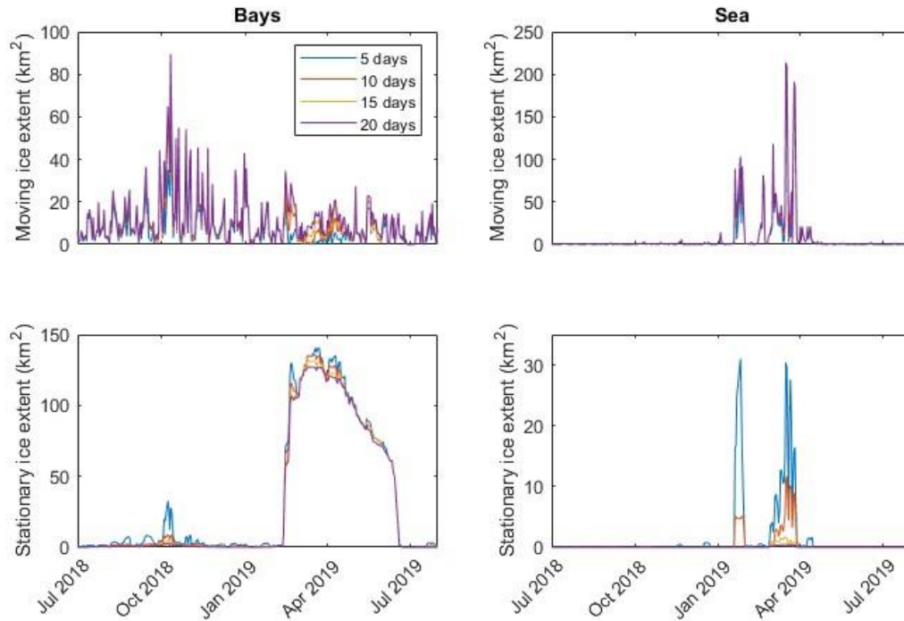
Figure 4. The extent of moving and stationary ice between 2018-07-01 and 2019-07-31 depending on the minimal number of consecutive days of ice presence in the bays and open sea as delimited in Fig. 1.
