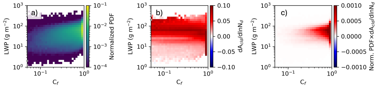
Figure 10. Radiative kernel for computing the Twomey effect using predictions of A_{cld} from the random forest model for the California region using 1^\circ grid-spacing data. Number of retrievals falling into log-bins of LWP and CF are normalized by the total (a), sensitivity of changes in A_{cld} for each bin determined using finite differences of the random forest predictions (b), and resulting Twomey radiative kernel (c) given by the product of (a) and (b).
