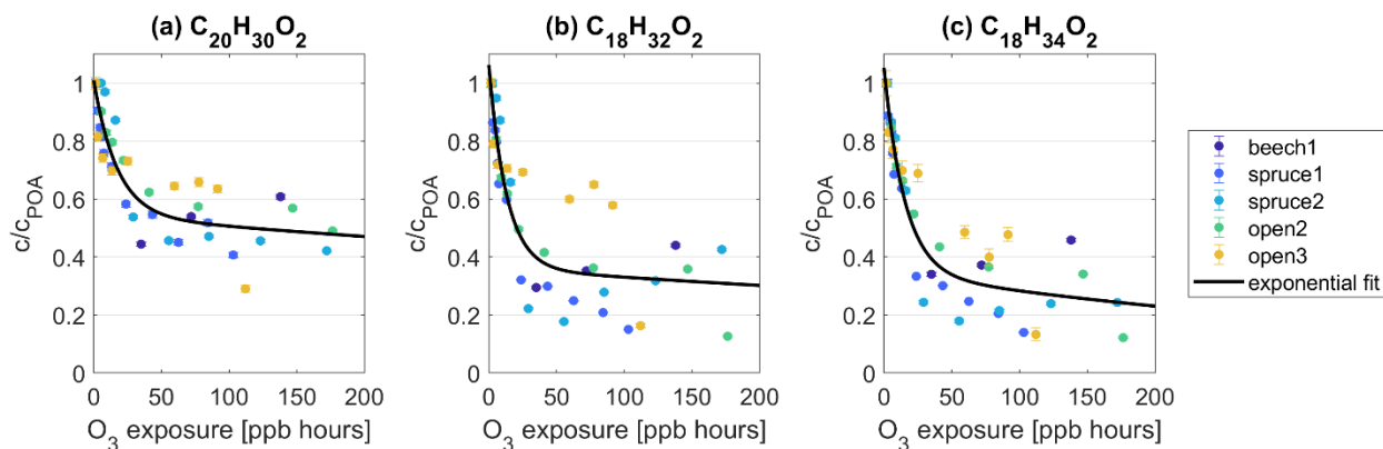
Figure 4: Intensity c of species (a) C_{20}H_{30}O_2 , (b) C_{18}H_{32}O_2 , (c) C_{18}H_{34}O_2 as fraction of their intensity at POA conditions c_{POA} and as function of O_3 exposure. The data points from all experiments were combined and are fitted with an exponential function of c/c_{POA} = a * \exp(b * p_{O_3} * t) + c * \exp(d * p_{O_3} * t) . The fit coefficients for C_{20}H_{30}O_2 ( C_{18}H_{32}O_2 , C_{18}H_{34}O_2 ) are a = 0.46 (0.70, 0.70), b = -56 (-76, -65) \cdot 10^3 (ppb hrs) ^{-1} , c = 0.54 (0.36, 0.35), and d = -0.7 (-0.9, -2) \cdot 10^3 (ppb hrs) ^{-1} . p_{O_3} is the O_3 concentration in ppb, t = 160 s is the reaction time in the OFR.
