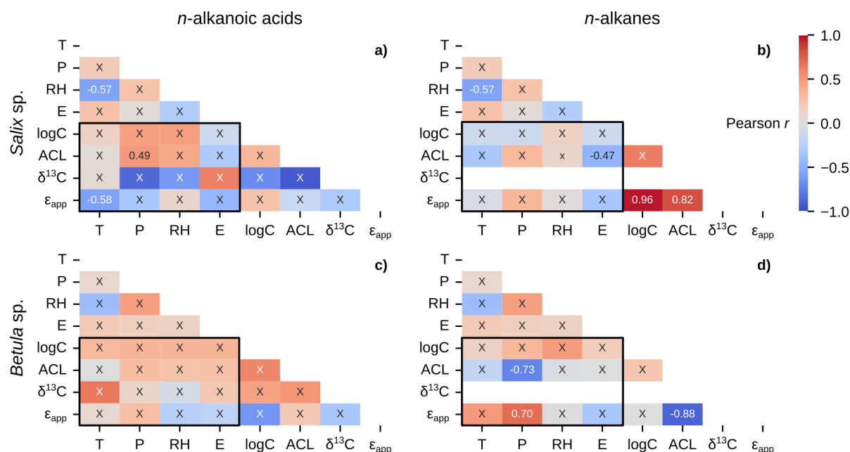
Figure 9. Matrices of Pearson correlation results using environmental parameters (T = MAF temperature; P = MAF precipitation amount; RH = MAF relative humidity; E = elevation) and chain-length amount-weighted plant wax indices of individual plant genera/species, with black boxes highlighting the correlation tests between the two. Left column panels (a, c) use plant wax n -alkanoic acid data and right column panels (b, d) use plant wax n -alkane data. (a-b) All plants within the Salix genus only. (c-d) Betula genus only. “X” annotations indicate the correlation is not significant ( p > 0.05 ).
