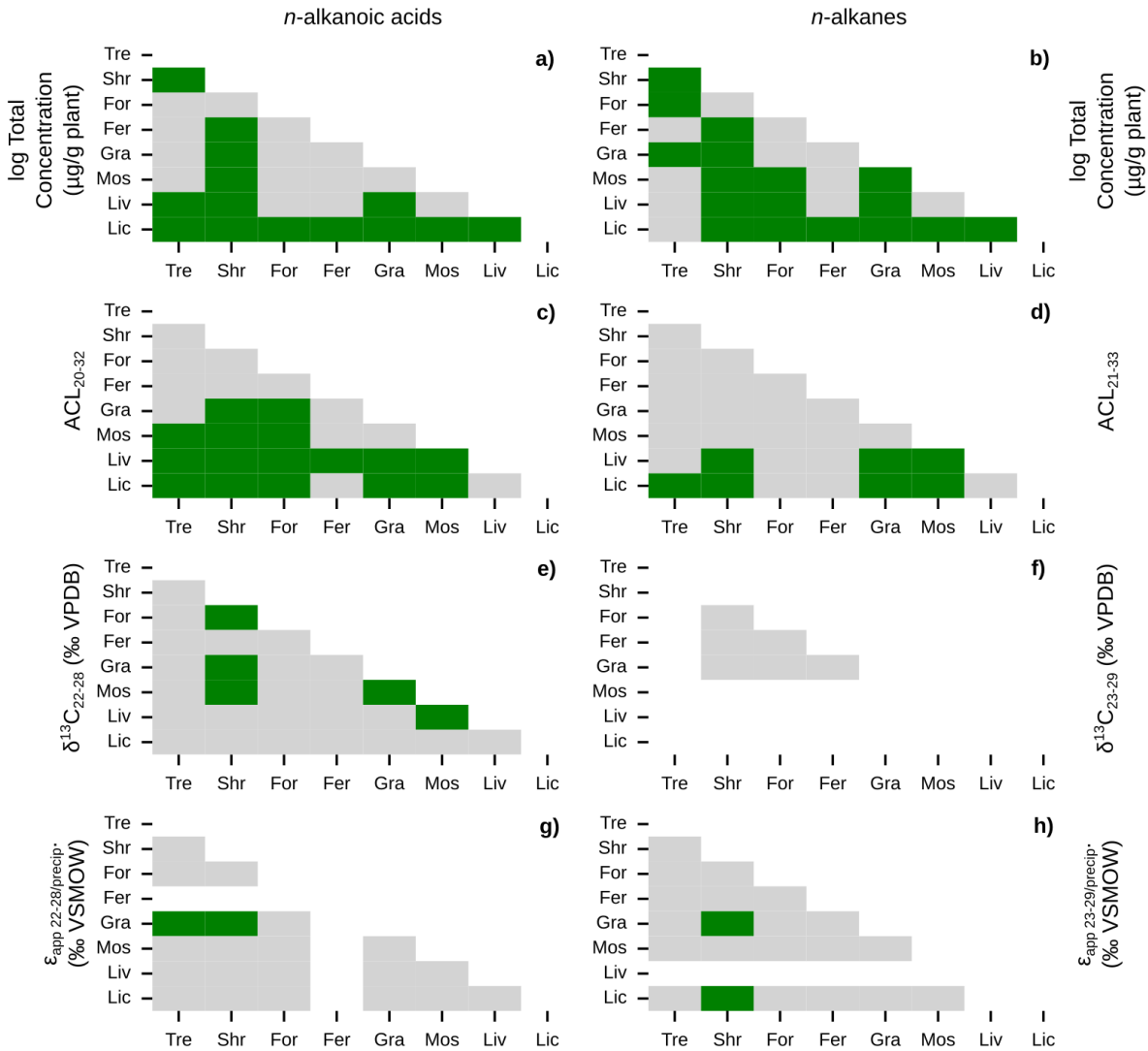
Figure 4. Similarities of plant wax data between plant growth forms. Matrices of Mann-Whitney U test p-values between pan-Arctic plant wax indices of major plant growth forms (Tre = trees, Shr = shrubs, For = forbs, Fer = ferns, Gra = graminoids, Mos = mosses, Liv = liverworts, Lic = lichens). Left column panels (a, c, e, g) use plant wax n -alkanoic acid data and right column panels (b, d, f, h) use plant wax n -alkane data. (a-b) Total plant wax concentration ( \mu\text{g/g} plant). (c-d) Plant wax ACL. (e-f) Plant wax \delta^{13}\text{C} . (g-h) Plant wax \epsilon_{app} relative to MAF precipitation amount-weighted \delta^2\text{H} . Green cells represent p -values < 0.05 , indicating the two datasets are significantly different from each other, grey cells represent p -values \geq 0.05 , and white cells indicate that there was an insufficient number of observations to perform the test.
