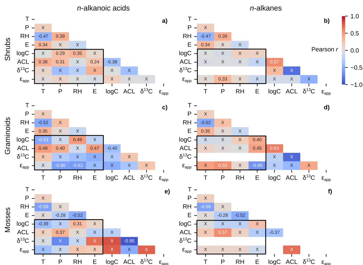
Figure 8. Matrices of Pearson correlation results using environmental parameters (T = MAF temperature; P = MAF precipitation amount; RH = MAF relative humidity; E = elevation) and chain-length amount-weighted plant wax indices of individual plant growth forms, with black boxes highlighting the correlation tests between the two. Left column panels (a, c, e) use plant wax n -alkanoic acid data and right column panels (b, d, f) use plant wax n -alkane data. (a-b) Shrubs. (c-d) Graminoids. (e-f) Mosses. “X” annotations indicate the correlation is not significant ( p > 0.05 ).
