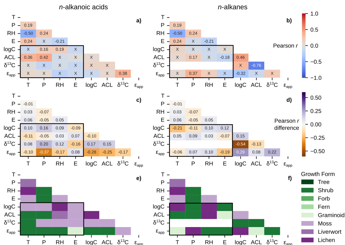
Figure 6. Matrices of Pearson correlation results using environmental parameters (T = MAF temperature; P = MAF precipitation amount; RH = MAF relative humidity; E = elevation) and chain-length amount-weighted plant wax indices, with black boxes highlighting the correlation tests between the two. Left column panels (a, c, e) use plant wax n -alkanoic acid data and right column panels (b, d, f) use plant wax n -alkane data. (a-b) Pearson correlation r values with all plant growth forms included. “X” annotations indicate the correlation is not significant ( p > 0.05). (c-d) Maximum, positive or negative, Pearson r value difference between the full dataset and tests removing one plant growth form at a time. (e-f) Plant growth form removed that is responsible for the values in panels c and d.
