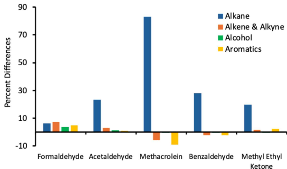
Figure 5: Sensitivity of carbonyl compounds to changes in NMO precursor groups (MCMv331 output). The bars represent the changes in carbonyl mixing ratios due to an increase in the NMO mixing ratio of 50%.
