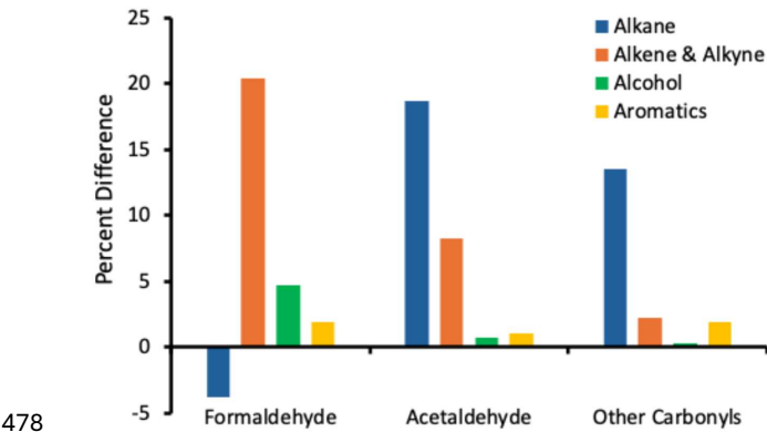
479 Figure 8: Sensitivity of hydrocarbons to carbonyl compounds (CB6 Output). The bars represent the changes in carbonyl 480 mixing ratios due to the increase in the hydrocarbon initial mixing ratio by 50%.
