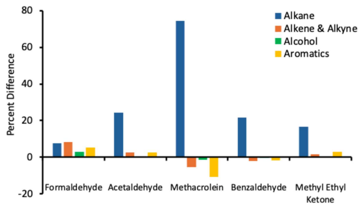
447 Figure 6: Sensitivity of hydrocarbons to carbonyl compounds (SAPRC07 Output). The bars represent the changes in 448 carbonyl mixing ratios due to the increase in the hydrocarbon initial mixing ratio by 50%.
