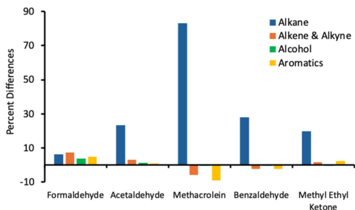
443 Figure 5: Sensitivity of carbonyl compounds to changes in NMOC precursor groups (MCMv331 output). The bars 444 represent the changes in carbonyl mixing ratios due to an increase in the NMOC mixing ratio of 50%.
