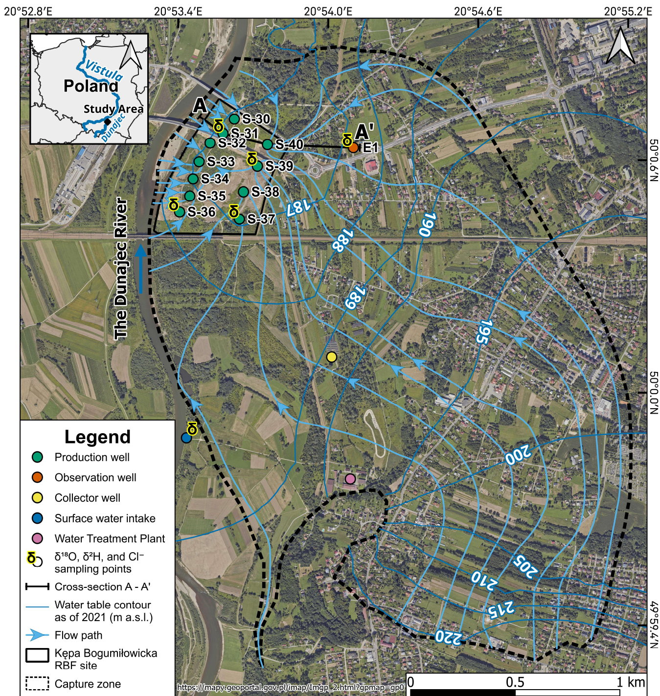
Figure 12: Overview of the study area. Average groundwater flow conditions (spring of 2021), groundwater table contour lines and flow directions, as well as the capture zone extension, are based on steady-state groundwater flow modelling results (Sitek et al., 2025).
