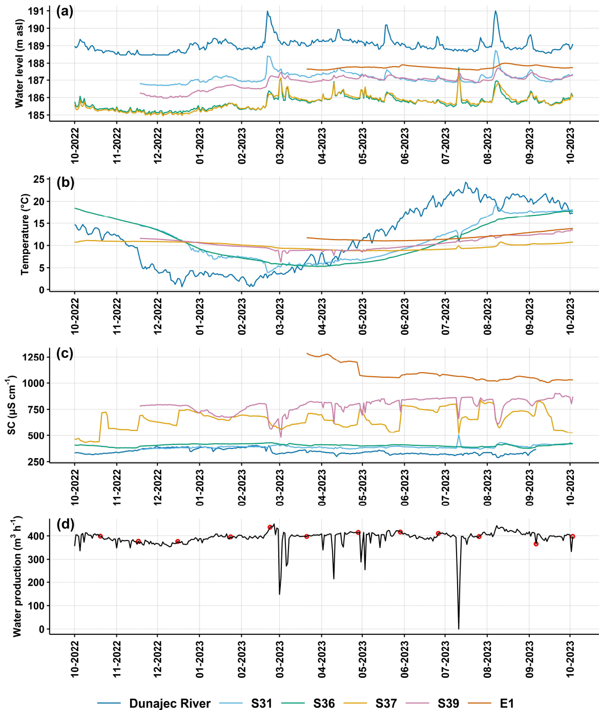
335 Figure 6: Datalogger (sensor) observations of mean daily Dunajec and groundwater levels (a), temperature (b), and specific conductance - SC (c), as well as the mean daily water production (groundwater abstraction rate) of the analysed well field (d). Sampling days are marked as red circles on (d).
