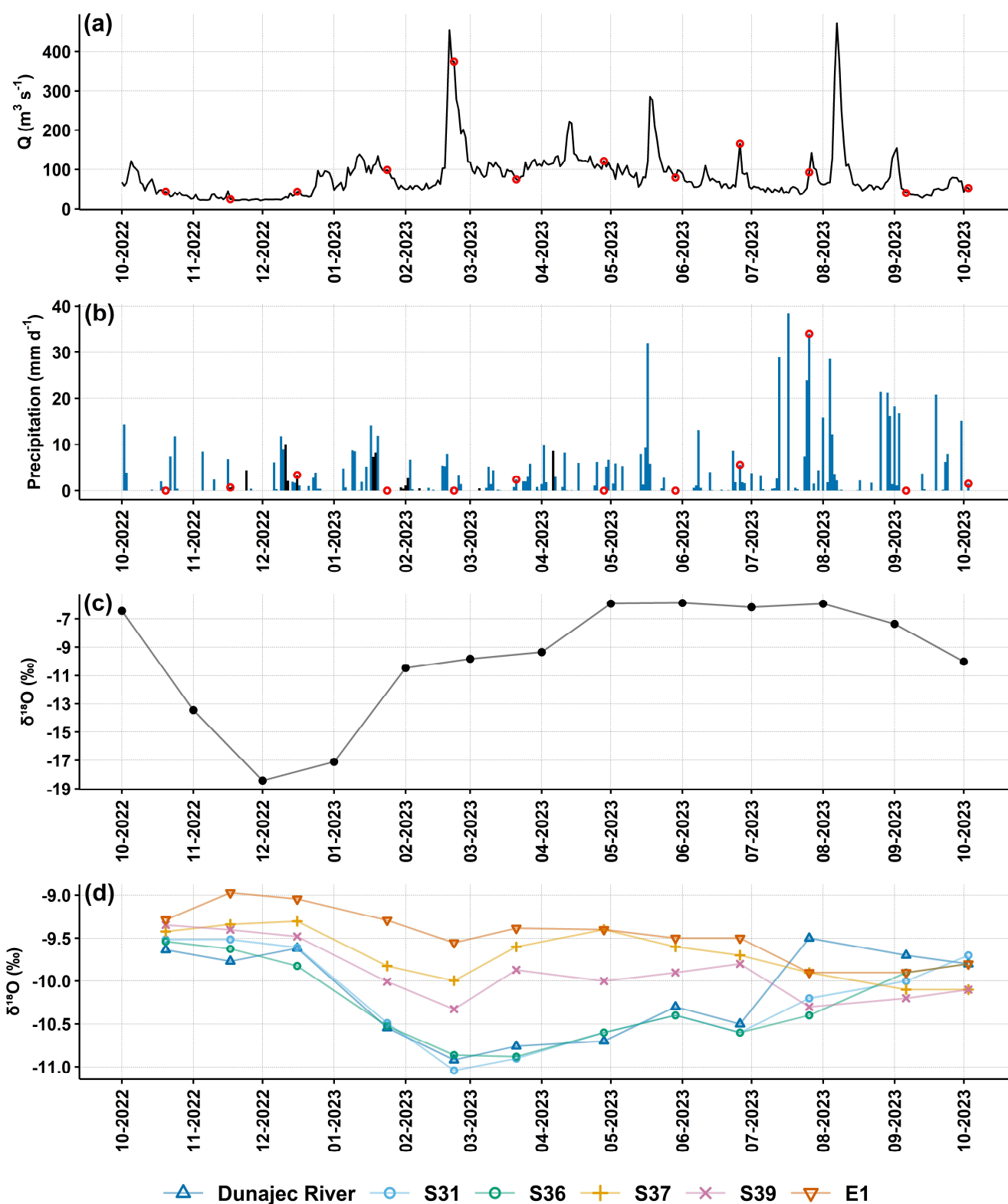
Figure 4: Mean daily flow rates of the Dunajec River Mean-daily-Dunajec-River-flow-rate at the Zglobice water-gauging station (a), daily precipitation in Tarnów in the form of rain (blue) or snow (black) (b), monthly means of \delta^{18}\text{O} in precipitation (Kraków station) (c), as well as \delta^{18}\text{O} in the Dunajec River water and groundwater in the study area throughout the sampling period (October 2022–October 2023). Red circles on plots (a) and (b) indicate the days of water sampling.
