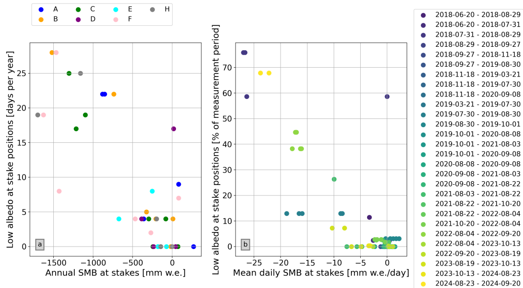
Figure 6. Panel a) Cumulative annual surface mass balance at the stakes plotted against the estimated number of "low albedo" (<0.40) days per year at each stake position. Panel b) Mean daily surface mass balance (SMB per measurement period divided by the length of the period) for each measurement period at the stakes plotted against the percentage of "low albedo" (<0.40) days at the respective stakes during the same measurement period.
