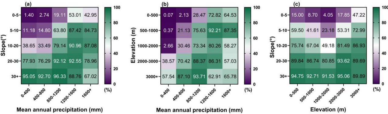
Figure. 6: Area proportions (%) of median to very high landslide susceptibility within inhabited areas of China during the historical baseline period (1950–2014), based on combinations of key continuous variables: (a) mean annual precipitation and slope, (b) mean annual precipitation and elevation, and (c) elevation and slope. Each cell represents the proportion of areas with median to very high susceptibility (classes 3–5) within the total area corresponding to that specific combination of factor ranges.
