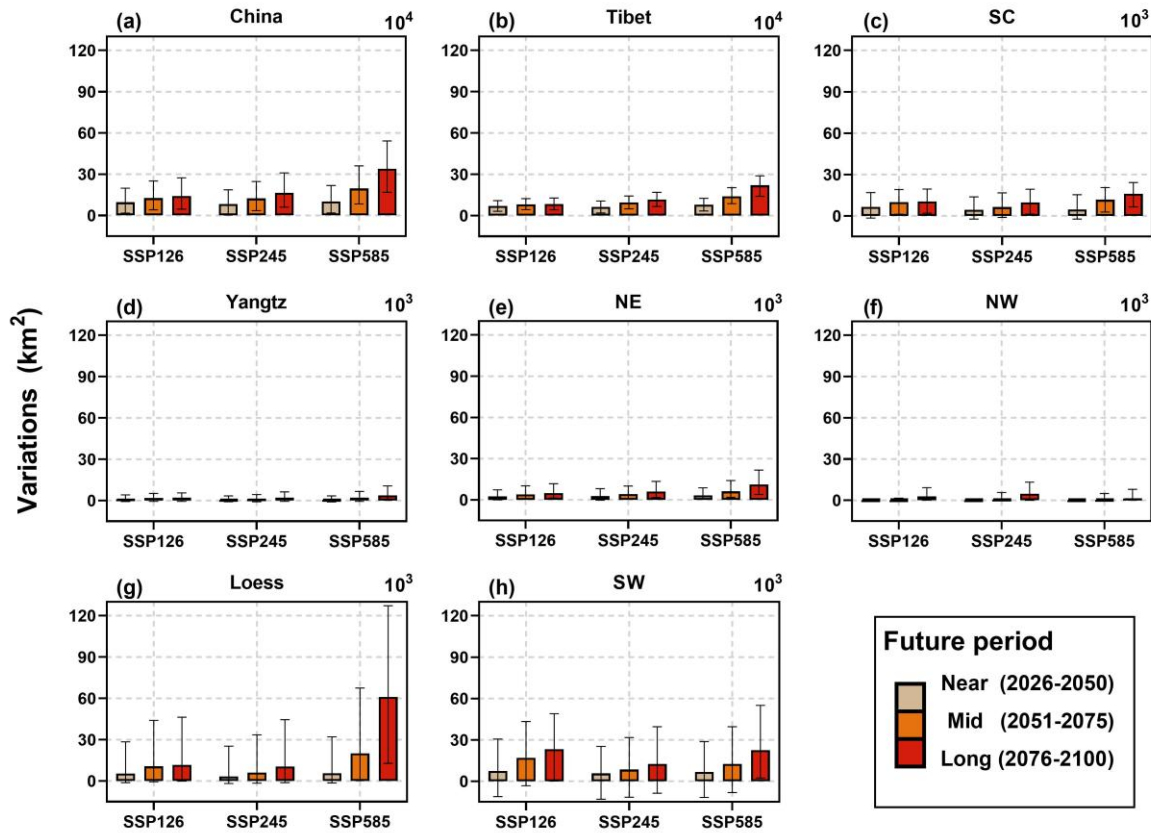
Figure. 9: Changes in the area of regions with median to very high landslide susceptibility under different future periods and SSPs, relative to the baseline period. Bars represent the multimodel ensemble mean changes, and error bars indicate the 95% confidence interval of the ensemble mean.
