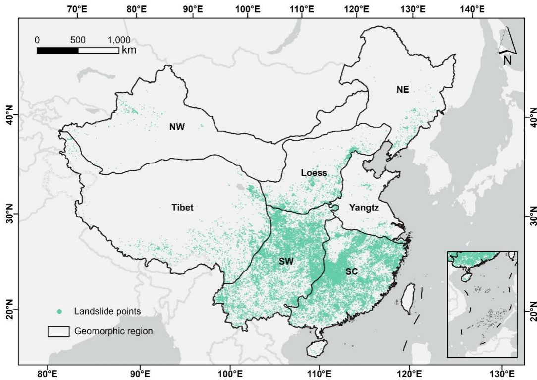
Figure. 1: Spatial distribution of rainfall-induced geological disaster events and major geological environmental regions in China. Geological environmental regions boundaries were obtained from https://geocloud.cgs.gov.cn/ . NE: Northeastern wetland ecology region; Yangtz: Huang-Huaihai-Yangtze River Delta plain region; SC: South China bedrock hills region; Loess: Northwest Loess Plateau region; SW: Southwest karst mountain region; NW: Northwest arid desert region; Tibet: permafrost region of the Qinghai-Tibet Plateau.
