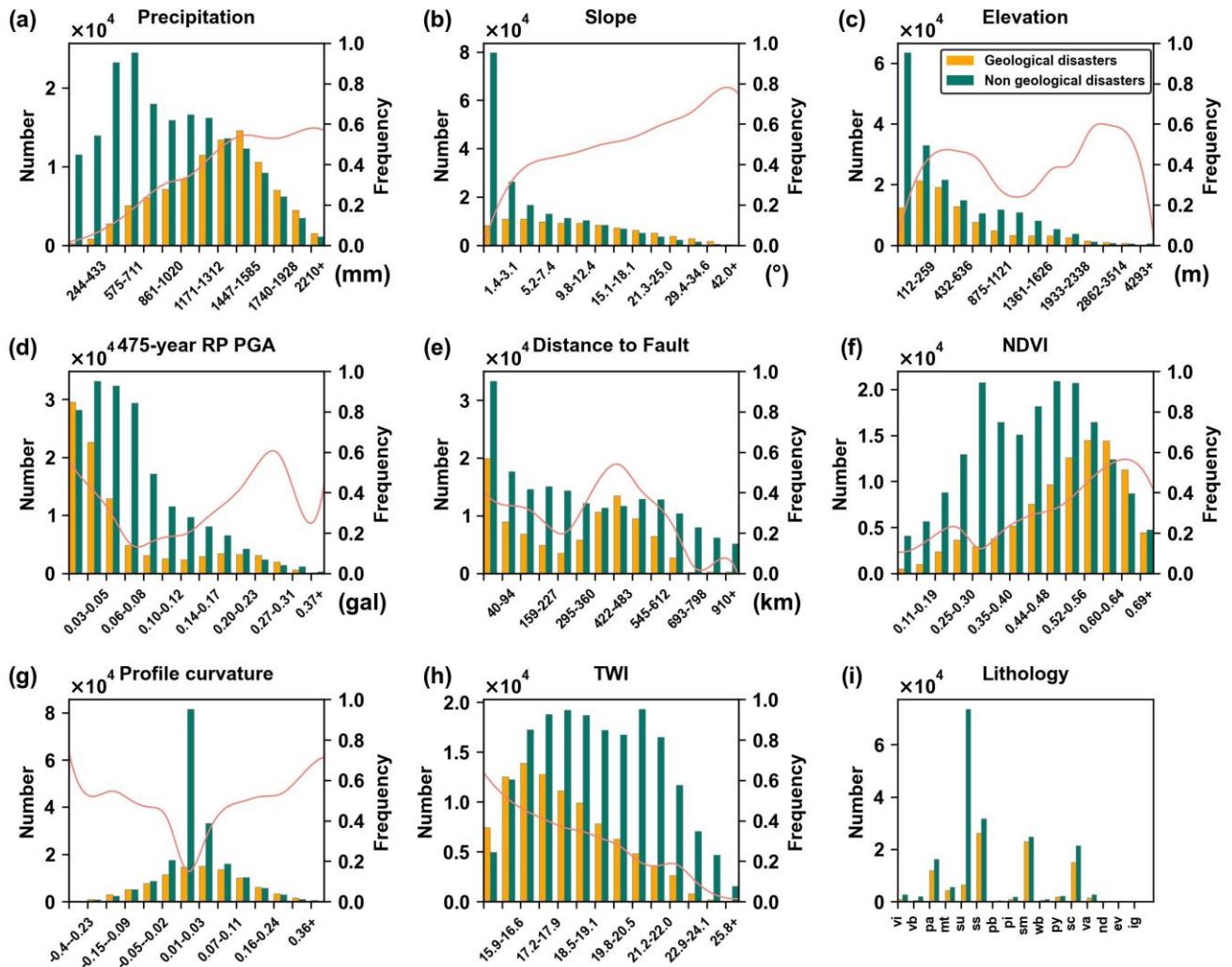
Figure. 10 The relationship between landslide points and non-landslide points and conditioning factors. (a) Precipitation: Annual total precipitation, (b) Slope, (c) Elevation, (d) 475-year return period PGA, (e) Distance to Fault, (f) NDVI, (g) Profile curvature, (h) TWI, and (i) Lithology.
