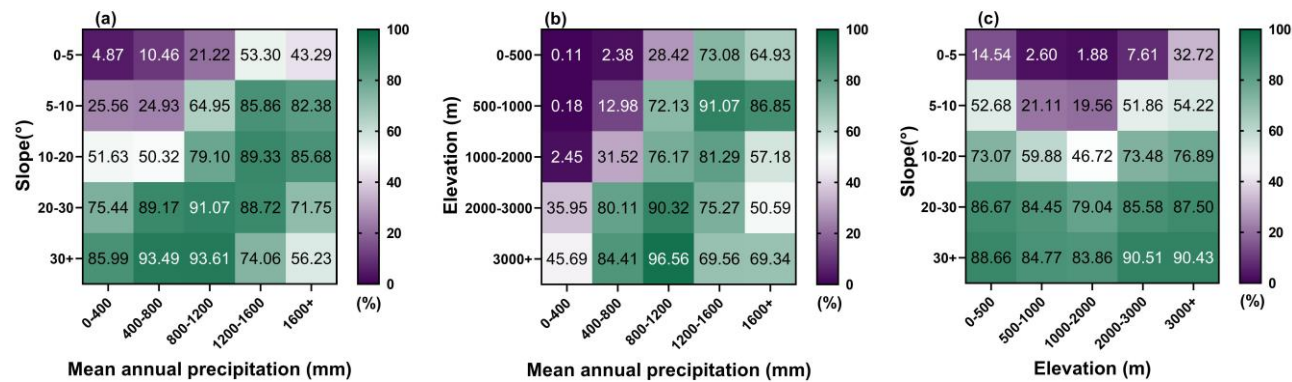
Figure. 6: Area proportions (%) of median to very high landslide susceptibility during the historical baseline period (1950–2014), based on combinations of key continuous variables: (a) mean annual precipitation and slope, (b) mean annual precipitation and elevation, and (c) elevation and slope. Each cell represents the proportion of areas with median to very high susceptibility (classes 3–5) within the total area corresponding to that specific combination of factor ranges.
