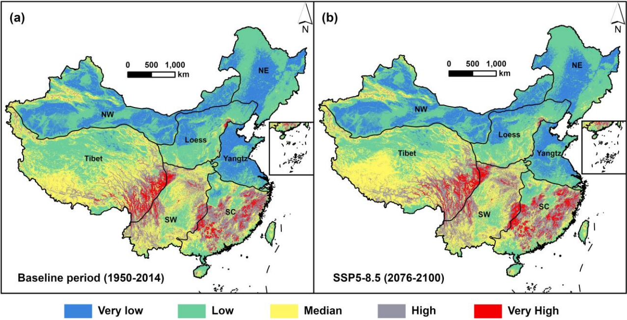
380 Figure. 8: Spatial pattern of landslide susceptibility in China during (a) the baseline period (1950–2014), and (b) the long-term future (2076–2100) under the SSP5-8.5.
