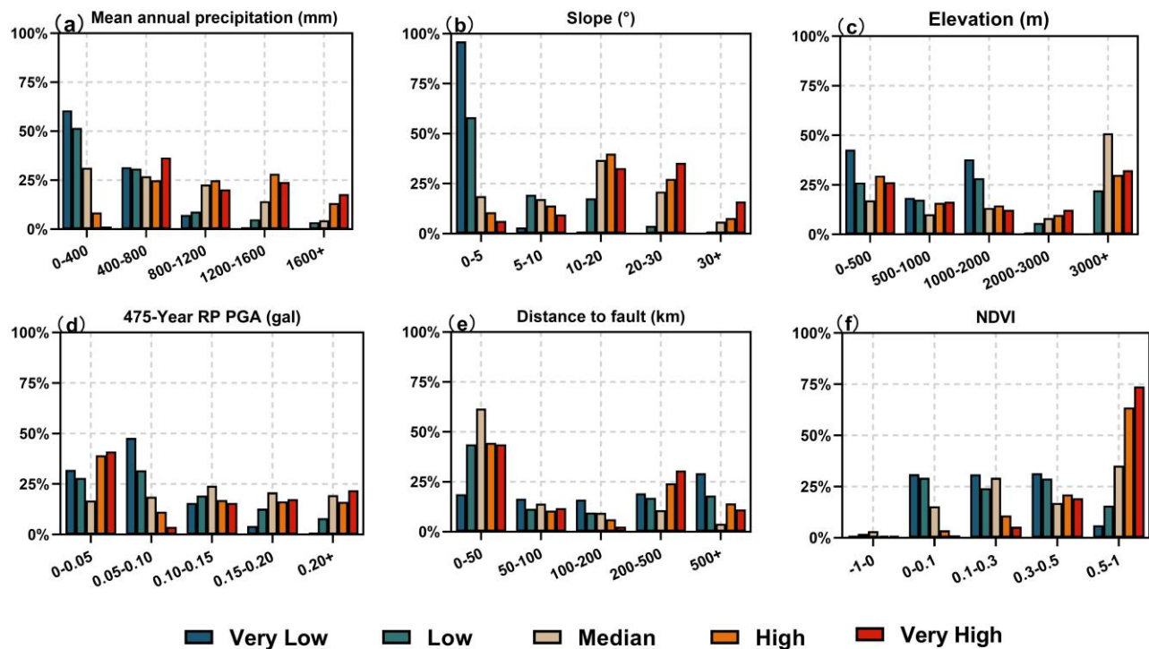
Figure. 5: Area proportions of landslide susceptibility classes across different categories of the top six continuous variables during the historical baseline period (1950–2014): (a) mean annual precipitation, (b) slope, (c) elevation, (d) 475-year RP PGA, (e) distance to fault, and (f) NDVI. Colours indicate susceptibility levels from very low to very high.
