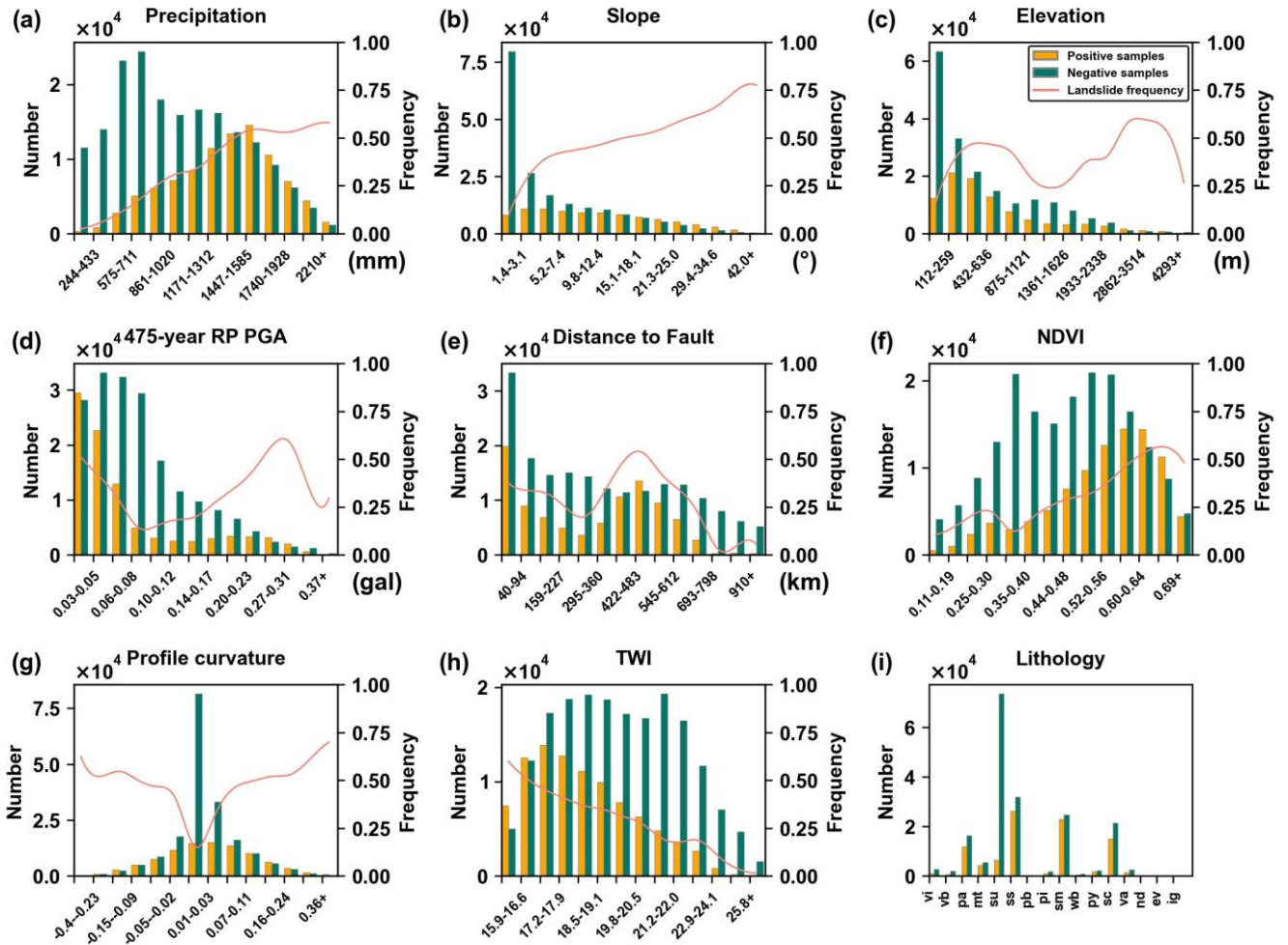
Figure. 10 Relationship between positive and negative samples and conditioning factors. (a) Precipitation: Annual total precipitation, (b) Slope, (c) Elevation, (d) 475-year return period PGA, (e) Distance to Fault, (f) NDVI, (g) Profile curvature, (h) TWI, and (i) Lithology. The red line represents the landslide frequency, calculated as the proportion of positive samples among all samples within each classified interval.
