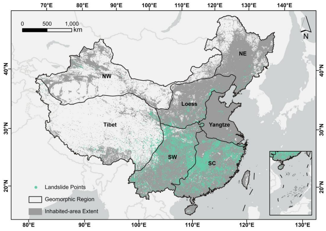
Figure. 1: Spatial distribution of rainfall-induced landslide-related records, inhabited-area extent, and major geomorphic regions in China. The grey background denotes the inhabited-area extent, which was used to define the study area. Geomorphic region boundaries were obtained from https://geocloud.cgs.gov.cn/ . NE: Northeastern wetland ecology region; Yangtze: Huang-Huaihai-Yangtze River Delta plain region; SC: South China bedrock hills region; Loess: Northwest Loess Plateau region; SW: Southwest karst mountain region; NW: Northwest arid desert region; Tibet: permafrost region of the Qinghai-Tibet Plateau. Geological environmental region boundaries by © China Geological Survey (CGS). All rights reserved.
