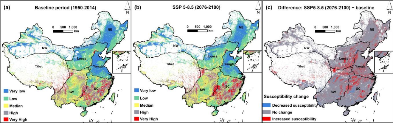
Figure. 8: Spatial pattern of landslide susceptibility within inhabited areas of China during (a) the baseline period (1950–2014), and (b) the long-term future (2076–2100) under the SSP5-8.5, and (c) the spatial change in susceptibility between the two periods. In panel (c), increased susceptibility indicates that the susceptibility class under SSP5-8.5 is higher than that during the baseline period, no change indicates that the susceptibility class remains unchanged, and decreased susceptibility indicates that the susceptibility class becomes lower.
