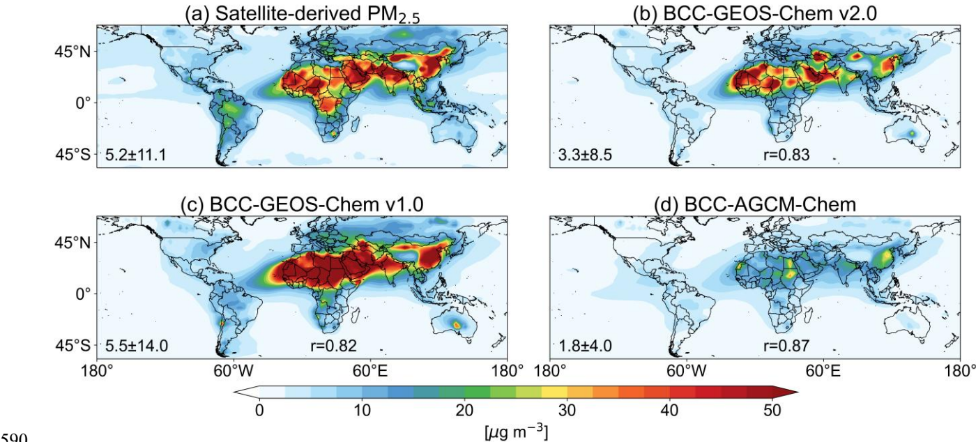
590 Figure 7. Spatial distributions of annual mean Surface fine particulate matter (PM 2.5 ) from (a) Satellite-derived PM 2.5 , (b) BCC-GEOS-Chem v2.0, (c) BCC-GEOS-Chem v1.0, and (d) BCC-AGCM-Chem. Values are averaged over 2012-2014.
