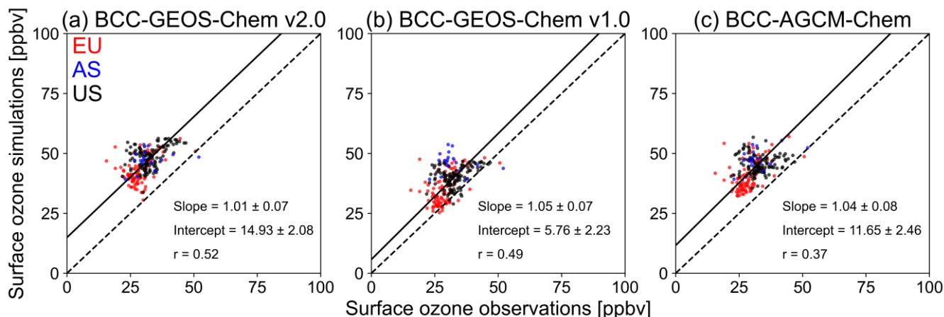
Figure 5. Scatter plots of observed and simulated surface ozone for (a) BCC-GEOS-Chem v2.0, (b) BCC-GEOS-Chem v1.0, and (c) BCC-AGCM-Chem over 2012-2014. The solid lines indicate the regression lines. The dotted lines indicate the 1: 1 line. Observations are averaged to the same model grid.
