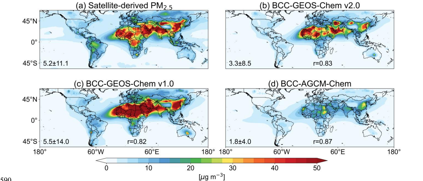
590 Figure 7. Spatial distributions of annual mean Surface fine particulate matter ( \text{PM}_{2.5} ) from (a) Satellite-derived \text{PM}_{2.5} , (b) BCC-GEOS-Chem v2.0, (c) BCC-GEOS-Chem v1.0, and (d) BCC-AGCM-Chem. Values are averaged over 2012-2014.
