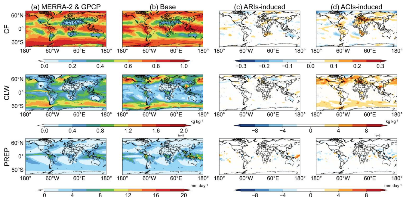
Figure 10. Annual mean cloud properties from (a) MERRA-2 reanalysis data or GPCP satellite data, (b) Base simulation, (c) ARIs-induced, and (d) ACIs-induced. Variables evaluated include the cloud fraction (CF), mass fraction of cloud liquid water (CLW), and total precipitation (PREP).
