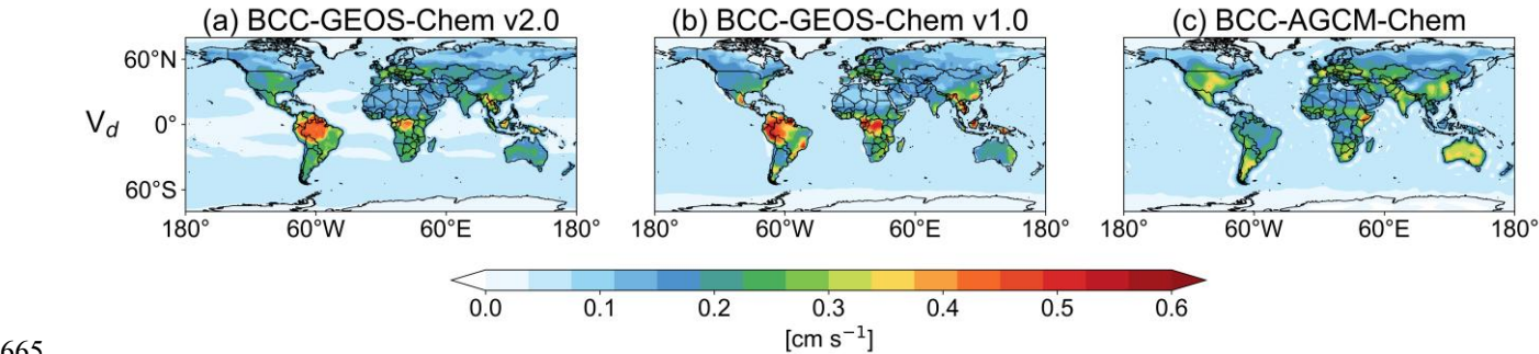
Figure 8. Annual mean distribution of global ozone dry deposition velocity for 2012–2014 from (a) BCC-GEOS-Chem v2.0, (b) BCC-GEOS-Chem v1.0, and (c) BCC-AGCM-Chem.
