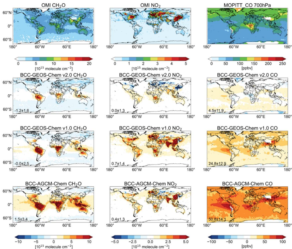
Figure 6. Spatial distributions of global tropospheric \text{NO}_2 column averaged over 2012–2014 from (a) OMI satellite observation, (b) differences between BCC-GEOS-Chem v2.0 and OMI, (c) differences between BCC-GEOS-Chem v1.0 and OMI, and (d) differences between BCC-AGCM-Chem and OMI.
