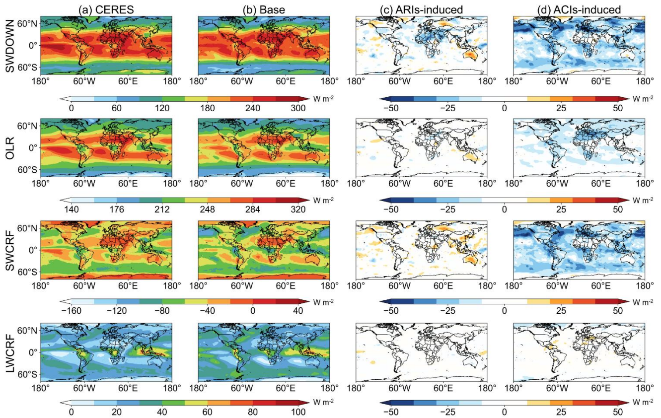
Figure 9. Annual mean radiative properties from (a) CERES satellite observations, (b) Base simulation, (c) ARIs-induced, and (d) ACIs-induced. Variables evaluated include the downward shortwave (SWDOWN) radiation, shortwave cloud radiative forcing (SWCRF), longwave cloud radiative forcing (LWCRF), and outgoing longwave radiation (OLR).
