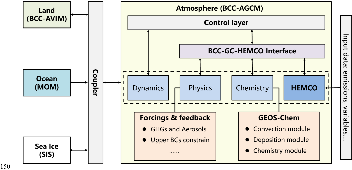
Figure 1. Architectural overview of the BCC-GEOS-Chem v2.0.
