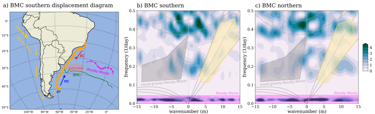
Figure 11: Diagram with the interactions in the BMC region modifying its displacement (a). Frequency and wavenumber diagram during extreme meridional displacement of the BMC separation: b) BMC southern in 2014, c) BMC northern in 1997. The spectrum reveals the frequency and wavenumber in the model SSH outputs band-pass series filtered between 40 and 130 days for the 300 m isobath between latitudes 20°S and 50°S. The diagram is for the transect along the 300m isobath, in orange.
