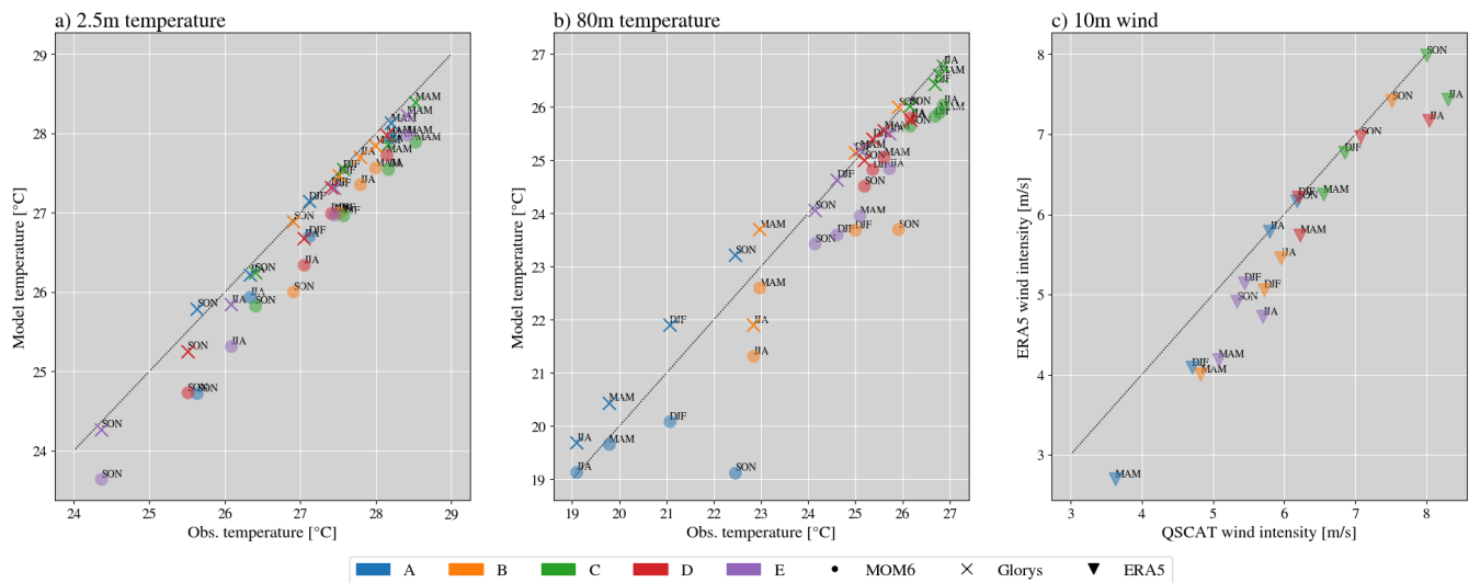
Figure A1: As in Figure 5: Seasonal 2.5-m and 80-m temperatures and 10-m winds, compared against observations. The graphs display the temperature at 2.5 m (a) and 80 m (b) for the model and reanalysis compared to PIRATE buoy observations. In (c), the atmospheric forcing for the model, 10-m wind from ERA5, compared to QSCAT satellite observation (Hoffman and Leidner, 2005). Colors distinguish the buoy sites from A to E. The model data is obtained with the z^* vertical coordinate and marked with circles, extending from 1997 to 2017. The reanalysis from Glorys takes crosses and ERA5 triangles. The seasons are named as DJF, MAM, JJA, and SON.
