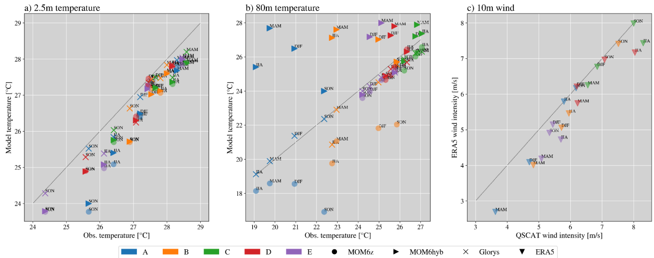
Figure 5: Seasonal 2.5-m and 80-m temperatures and 10-m winds, compared against observations. The graphs display the temperature at 2.5 m (a) and 80 m (b) for the model and reanalysis compared to PIRATE buoy observations. In (c), the atmospheric forcing for the model, 10-m wind from ERA5, compared to QSCAT satellite observation (Hoffman and Leidner, 2005). Colors distinguish the buoy sites from A to E. The model data is plotted with two vertical discretizations: MOM6z takes the z -coordinate system and MOM6hyb uses a hybrid system. The same period of 5 years is considered for the model data. The reanalysis from GLORYS12v1 is marked with crosses and ERA5 triangles. The seasons are named as DJF, MAM, JJA, and SON.
