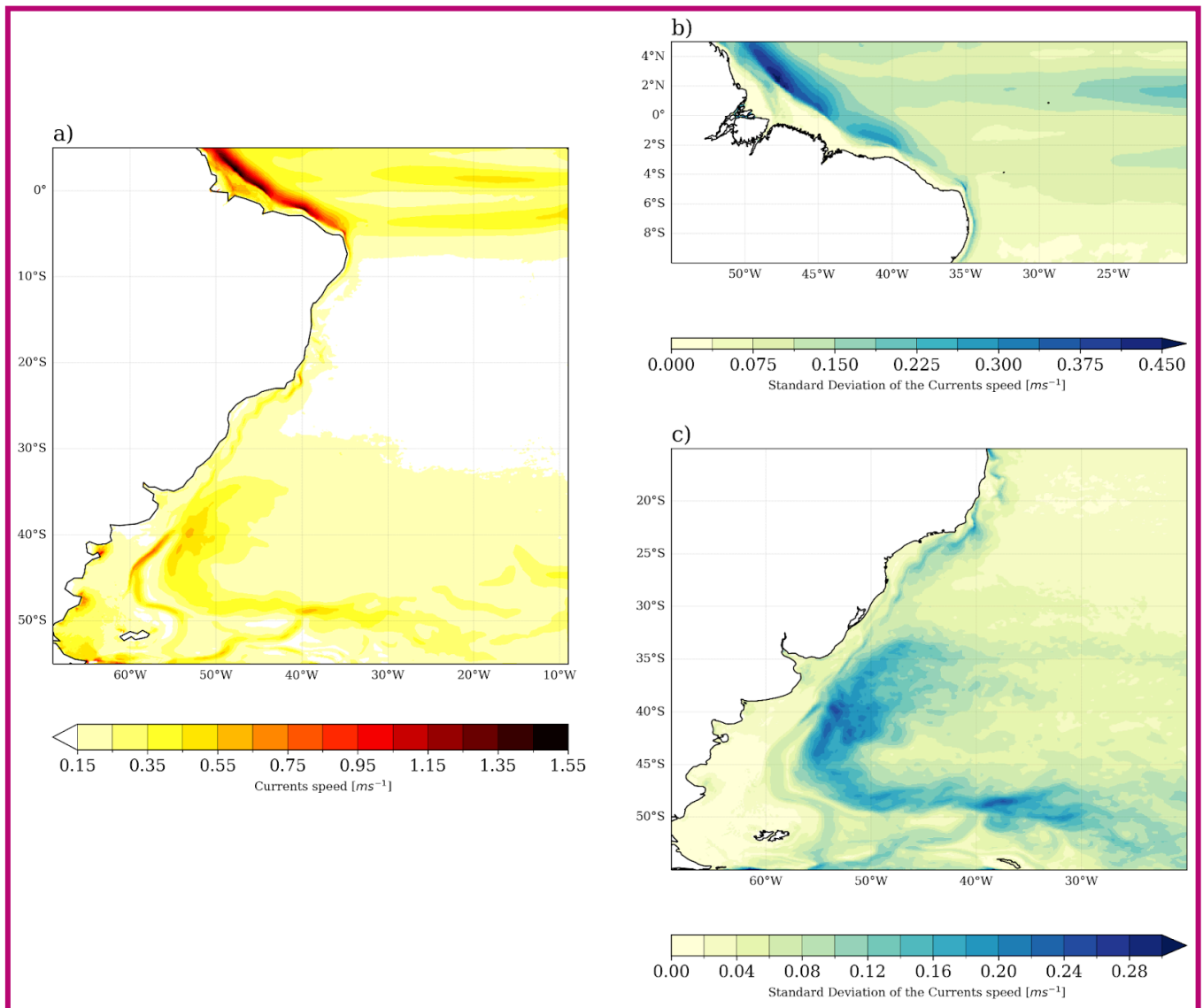
Figure 6: Mean sea surface currents (m/s) (a) and standard deviation of the mean speed (m/s) for the NBC (b) and the BMC (c) regions. The standard deviation considers the monthly variability of speed in the domain. The main BC and MC path appears with currents speed above 0.3 m/s and 0.6 m/s, respectively, while the speed of the NBC is above 1 m/s.
