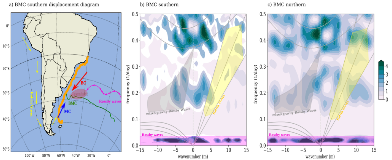
Figure 11: Diagram with the interactions in the BMC region modifying its displacement (a). Frequency and wavenumber diagram during extreme meridional displacement of the BMC separation: b) BMC southern in 2014, c) BMC northern in 1997. The spectrum reveals the frequency and wavenumber in the model SSH outputs band-pass series filtered between 40 and 130 days for the 300 m isobath between latitudes 20°S and 50°S. The diagram is for the transect along the 300m isobath, in orange.
