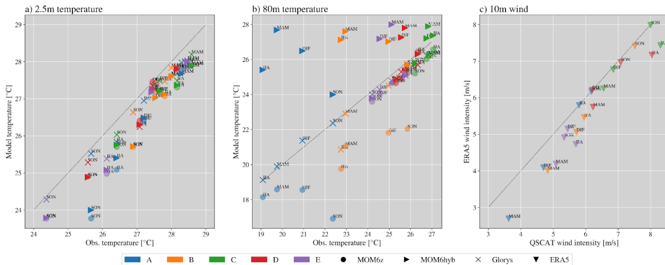
Figure 5: Seasonal 2.5-m and 80-m temperatures and 10-m winds, compared against observations. The graphs display the temperature at 2.5 m (a) and 80 m (b) for the model and reanalysis compared to PIRATE buoy observations. In (c), the atmospheric forcing for the model, 10-m wind from ERA5, compared to QSCAT satellite observation (Hoffman and Leidner, 2005). Colors distinguish the buoy sites from A to E. The model data is plotted with two vertical discretizations: MOM6z takes the z -coordinate system and MOM6hyb uses a hybrid system. The same period of 5 years is considered for the model data. The reanalysis from GLORYS12v1 is marked with crosses and ERA5 triangles. The seasons are named as DJF, MAM, JJA, and SON.
