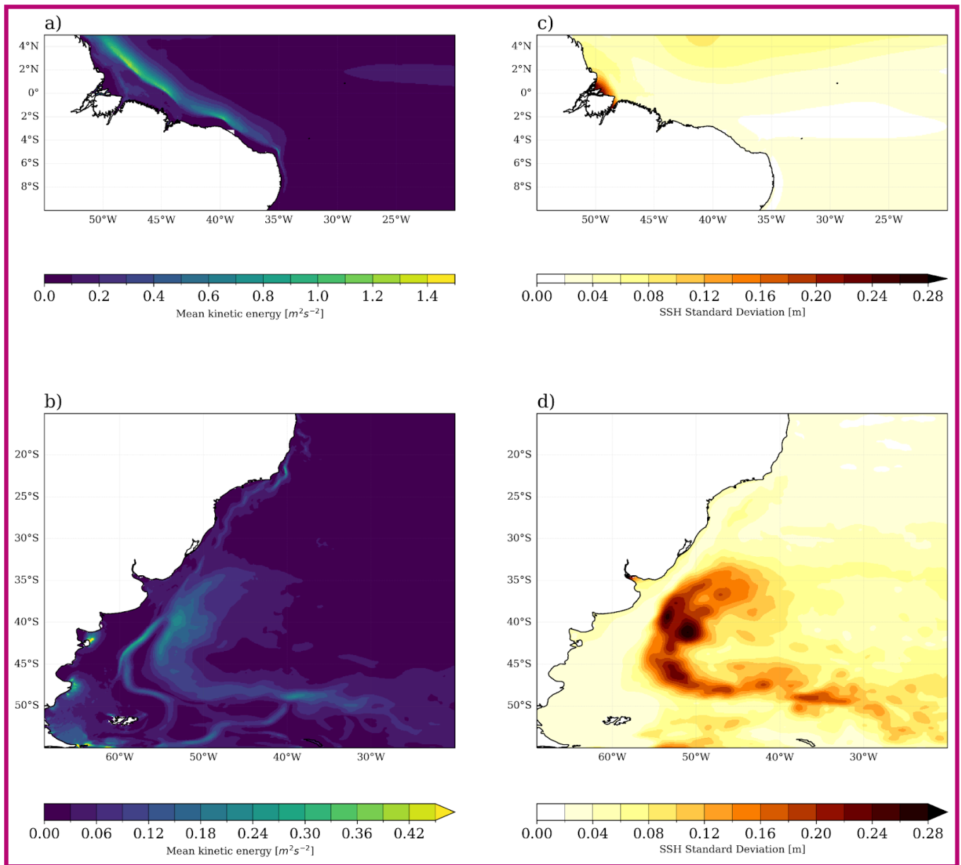
Figure 7: Standard deviations of the Mean Kinetic Energy ( m^2s^{-2} ) (a,b) and SSH (m) (c,d) in the regions of the WBCs. In the latter, fields are std concerning the monthly variability from 1997 until 2017.
