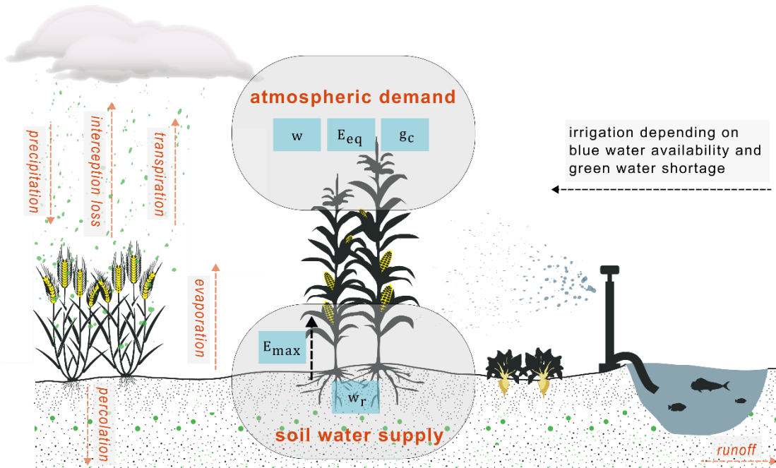
170 Figure 1: Schematic overview of basic processes considered in the calculation of the green water scarcity indicator. See text/equations for abbreviations.
