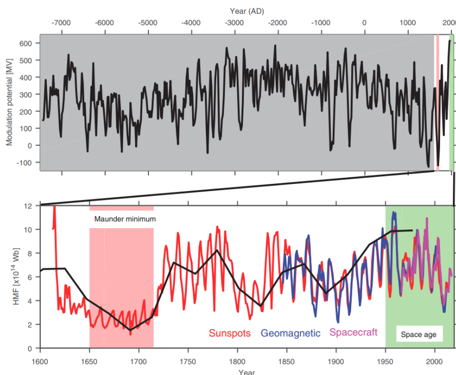
Figure 7. Reconstructions of solar activity from a range of sources, including direct spacecraft measurements, ground-based magnetometers, sunspot observers, and radionuclide information in tree rings and ice sheets. Reprinted from (Owens et al., 2018);
