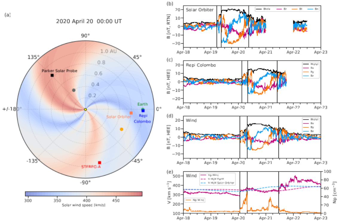
Figure 3. (a) Overview of spacecraft positions in the Heliosphere and in situ solar wind speed data up to 1 AU. (b) Solar Orbiter (c) BepiColombo, (d) Wind, magnetic field data, and (e) the wind proton speed and density (solid lines) and the WSA/HUX solar wind speed at Earth and Solar Orbiter (dashed lines). Vertical lines indicate, from left to right, the shock arrival time and the beginning and end times of the flux rope, determined visually. Reprinted from (Davies et al., 2021).
