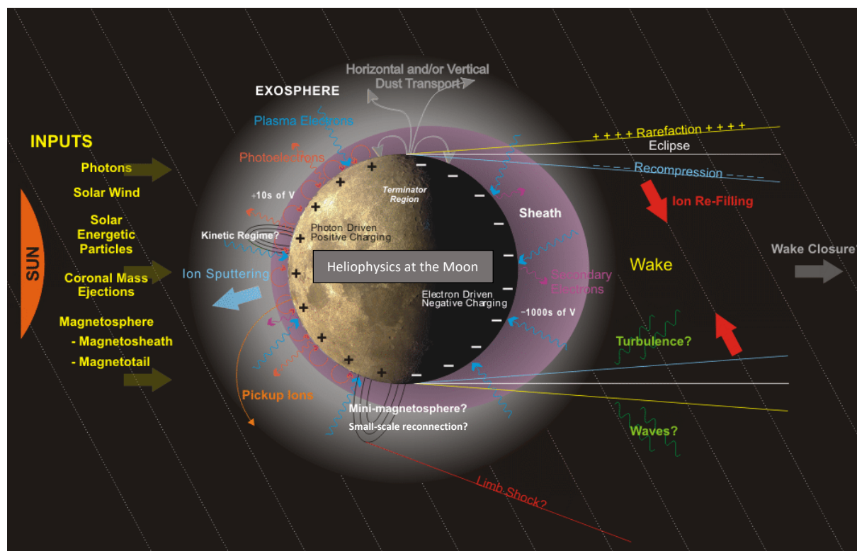
Figure 6. Physical processes acting in the lunar environment. Reprinted from (Halekas et al., 2023).
