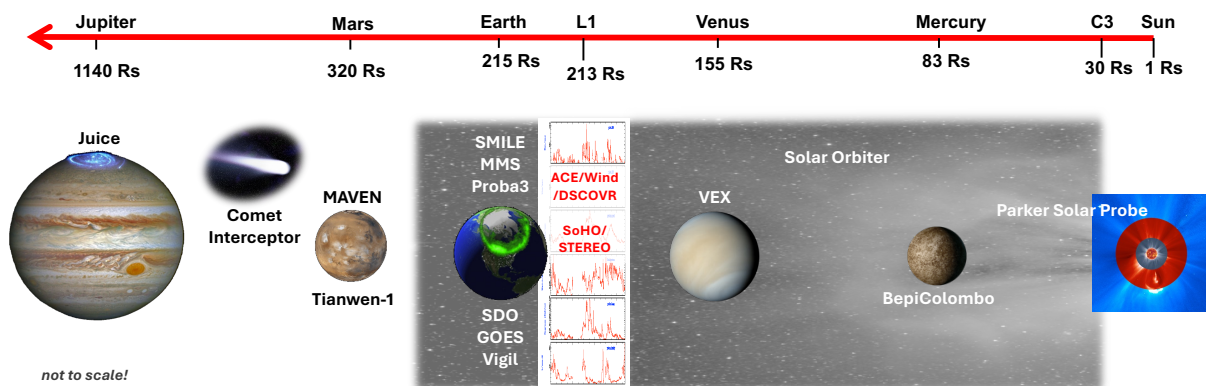
Figure 2. Selection of current, past, and future space missions that carry various types of instruments addressing heliophysics. These missions pursue a wide range of scientific objectives across different disciplines and over large distances, thereby deepening our understanding of the space plasma that fills our solar system. Remote sensing imaging data best cover the inner heliosphere, while in situ measurements provide local information about the plasma and magnetic field environment. Individual images taken from ESA/NASA. Figure adapted from Temmer (2021).
