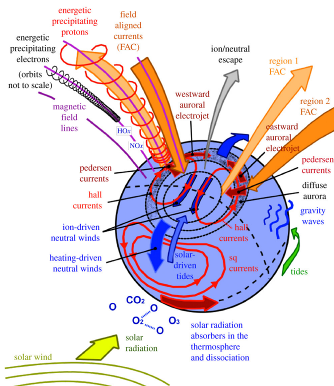
Figure 5. A schematic overview of ionosphere-thermosphere processes and their interaction with the magnetosphere and the solar wind (reprinted with authorisation from (Sarris, 2019)).
