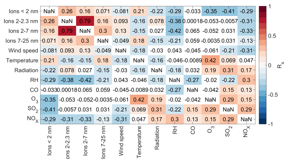
Figure B18. Spearman correlation coefficients between different variables during the day (10–15 h) in the summer (June–August). Each square corresponds to the correlation coefficient between the variables on the x- and y-axes and the colour indicates the strength of the correlation with the square being white if the p-value was above 0.05.
