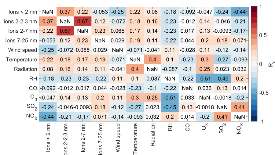
Figure B14. Spearman correlation coefficients between different variables for the whole dataset. Each square corresponds to the correlation coefficient between the variables on the x- and y-axes and the colour indicates the strength of the correlation with the square being white if the p-value was above 0.05.
