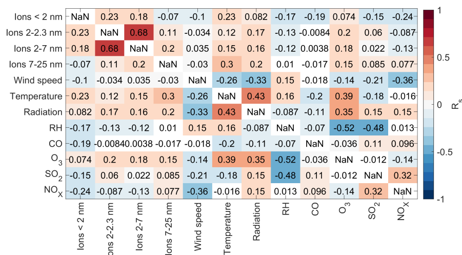
Figure B15. Spearman correlation coefficients between different variables in marine air. Each square corresponds to the correlation coefficient between the variables on the x- and y-axes and the colour indicates the strength of the correlation with the square being white if the p-value was above 0.05.
