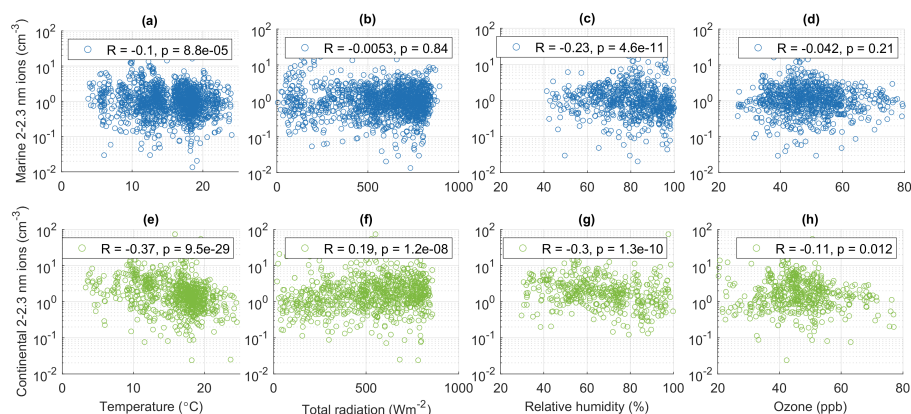
Figure B13. Concentration of 2–2.3 nm ions as a function of a) temperature, b) total radiation, c) relative humidity, and d) ozone only including data from summer and 10–15 h. The upper panel with blue data points contain data only from the marine wind sector and the lower panels with green data points data from the continental wind sector.
