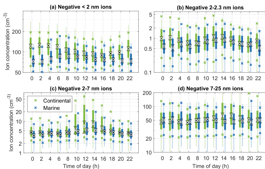
Figure B11. Diurnal cycles of ions in different size ranges for coastal and continental air when DMPS data is available. The black dots indicate the medians, the triangles indicate the confidence interval of the medians, the boxes the 25th–75th percentiles, the crosses the 10th and 90th percentiles, and the whiskers cover approximately 99.3 % of the data.
