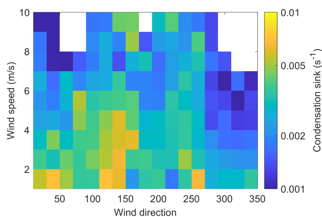
Figure B12. Average condensation sink in wind direction and wind speed bins. Note that the data are included only if the wind speed and direction bin has at least 10 data points and the condensation sink data are available only when data from all particle instruments is available (22.5.2023–29.6.2023 and 2.1.2024–24.6.2024)
