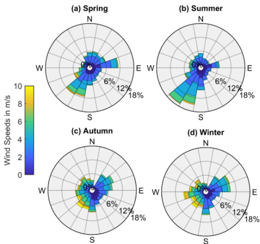
Figure B4. Wind roses for Tvärminne for different seasons.
