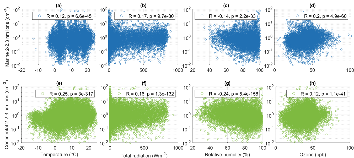
Figure 9. Concentration of 2–2.3 nm ions as a function of a) temperature, b) total radiation, c) relative humidity, and d) ozone in marine (blue) and continental (green) wind sectors
