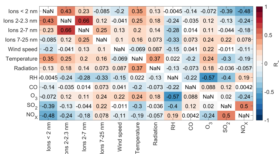
Figure B16. Spearman correlation coefficients between different variables in air coming from the land. Each square corresponds to the correlation coefficient between the variables on the x- and y-axes and the colour indicates the strength of the correlation with the square being white if the p-value was above 0.05.
