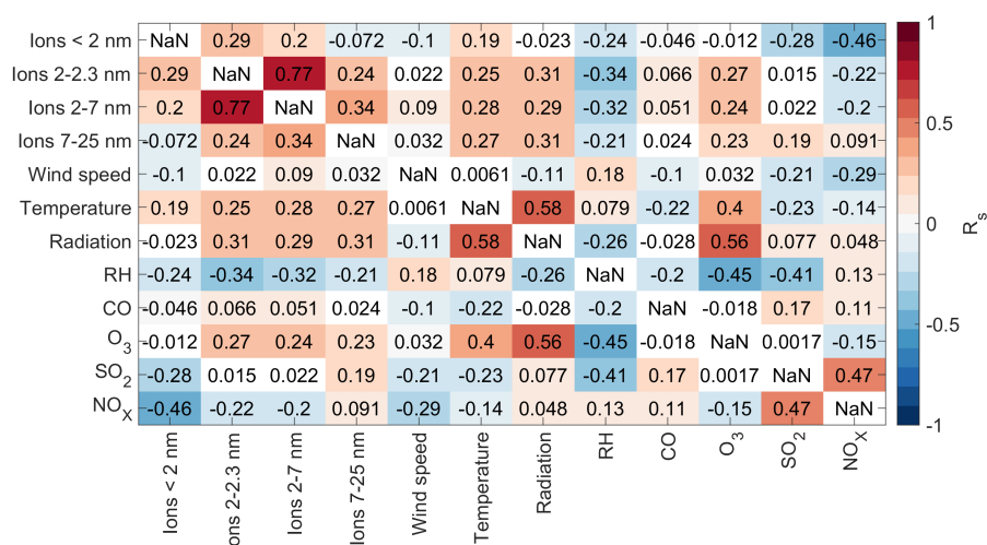
Figure B17. Spearman correlation coefficients between different variables during the day (10–15 h). Each square corresponds to the correlation coefficient between the variables on the x- and y-axes and the colour indicates the strength of the correlation with the square being white if the p-value was above 0.05.
