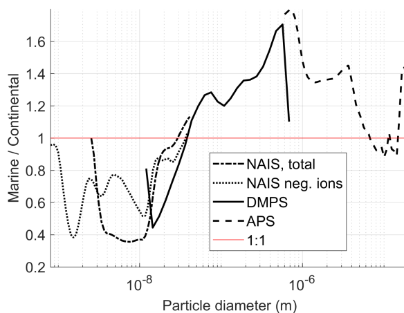
Figure B10. Average marine size distribution divided by average continental size distribution.
