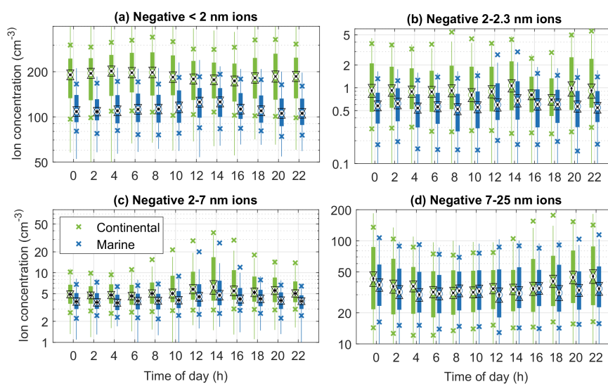
Figure B8. Diurnal cycles of ions in different size ranges for coastal and continental air in the autumn (September-November). The black dots indicate the medians, the triangles indicate the confidence interval of the medians, the boxes the 25th–75th percentiles, the crosses the 10th and 90th percentiles, and the whiskers cover approximately 99.3 % of the data.
