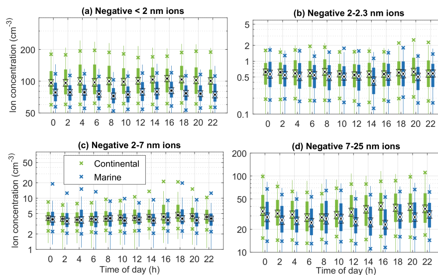
Figure B9. Diurnal cycles of ions in different size ranges for coastal and continental air in the winter (December-February). The black dots indicate the medians, the triangles indicate the confidence interval of the medians, the boxes the 25th–75th percentiles, the crosses the 10th and 90th percentiles, and the whiskers cover approximately 99.3 % of the data.
