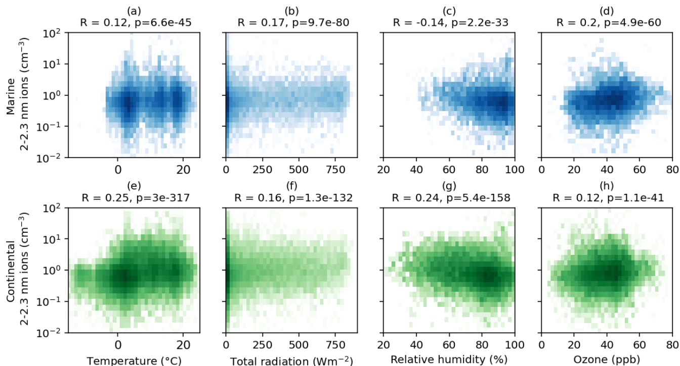
Figure 9. Concentration of 2–2.3 nm ions as a function of temperature (a and e) temperature , b ) total radiation , c ) relative humidity (c and g), and ozone (d and h) ozone in marine (blue, upper panels) and continental (green, lower panels) wind sectors. The transparency of the colour indicates the relative number of data points with more data where the colour is dark.
