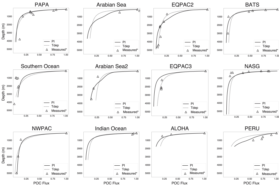
290 Figure 7. Site-specific POC flux attenuation. Measured values are denoted with open triangles (*see Table 2 for source references). As in previous figures, solid lines are preindustrial control and dashed lines are Tdep. All flux attenuations are normalized to POC flux at 150 meters.
