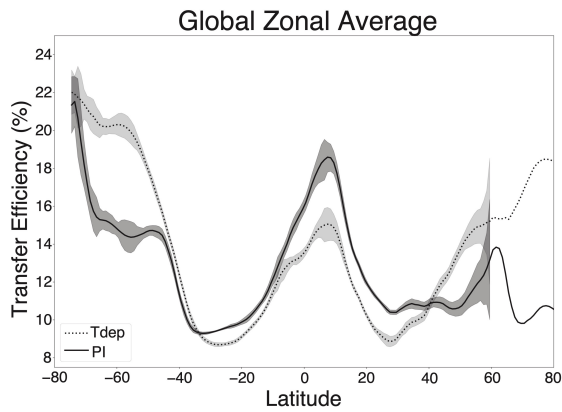
240 Figure 5. Global zonal average transfer efficiency. Preindustrial control results are shown as a solid line, and Tdep results as a dashed line. Interannual variability for the final 30 years of the run analysed here is shown as shaded 1- \sigma bands. The highest interannual variability occurs in the highly productive Southern Ocean, Equatorial Upwelling regions, and high northern latitudes. 1- \sigma bands are not shown north of 60N, where internal variability exceeds the range of transfer efficiency displayed due to sea ice impacts on primary productivity. ▼
