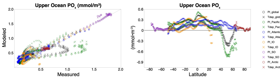
Figure 10. Data-model comparison. Upper ocean phosphate content (left panel) as in Figure 8 for preindustrial control (O’s) and Tdep (X’s) simulations versus World Ocean Atlas (WOA23). Difference between modeled upper ocean nutrient content and WOA23 upper ocean nutrient content (right panel) by latitude. Color is basin-specific as indicated.
