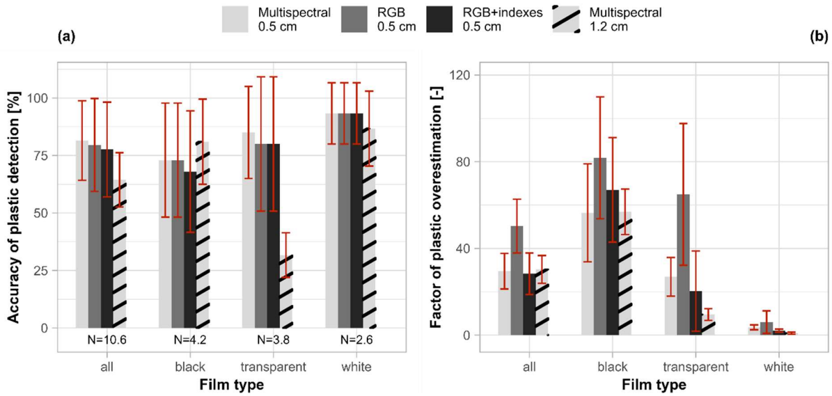
385 Figure 7 — On the left side, accuracy (i.e., producer accuracy) of plastic detection with four different datasets (a), separated by film and aggregated (i.e., 'all'). Error bars represent the standard deviation of the producer accuracy within the 5-fold cross-validation cross-validation ; the numbers below the bars (N) represent the average number of points used for validation. On the right side, factor of plastic overestimation of four different datasets, separated by film and aggregated (b). The factor of plastic overestimation was calculated as the ratio between the detected number and the expected number of plastic-covered pixels. Error bars represent the standard deviation of the overestimation within the 5-fold cross-validation cross-validation .
