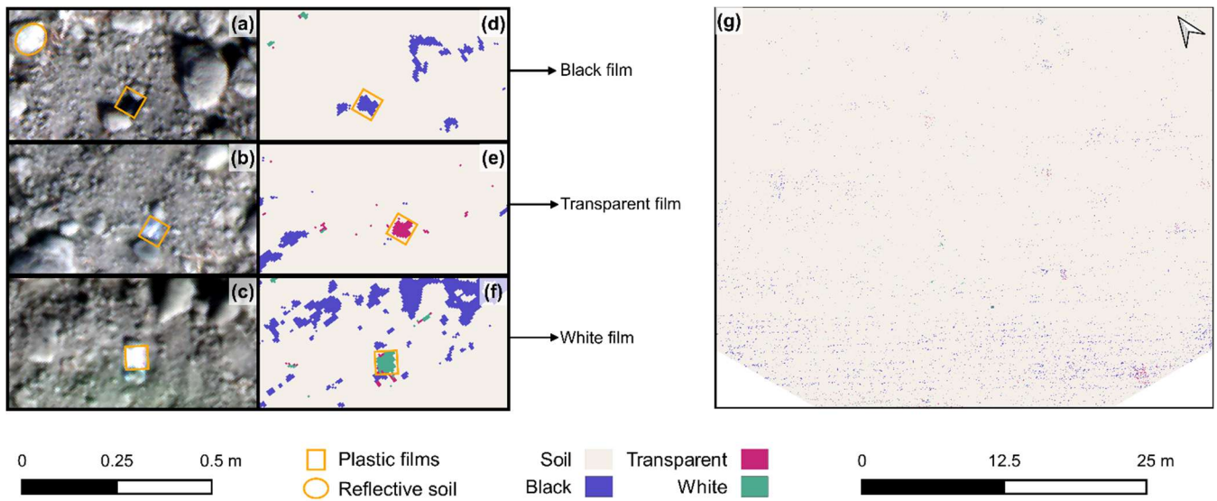
Figure 8 — Detail of the true colour images (a–c) and associated classification results (d–f) obtained with the multispectral 0.5 cm dataset. The classified map is shown in panel (g). On-In images (a–f), the exact location of the plastic films is highlighted. On-In image (a), the example of a highly reflective soil region is highlighted. The location of the plastic films placed on the field is highlighted in Fig. 2a.
