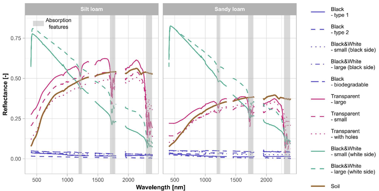
330 Figure 3 — Spectra of pristine plastic films and of soils used as background. On the left side, spectra acquired on silt loam; on the right side, spectra acquired on sandy loam. Film colours are represented by different colours, and variation—variations within film colours are represented by line shapes. Regions of absorption features are highlighted in light grey. Film names refer to Table 1.
