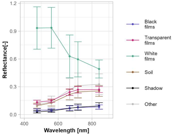
380 Figure 6 — Reflectance of plastic films divided by colour (i.e., black, transparent, white), compared to soil reflectance, shadow, and other non-plastic objects found on the experimental site.
