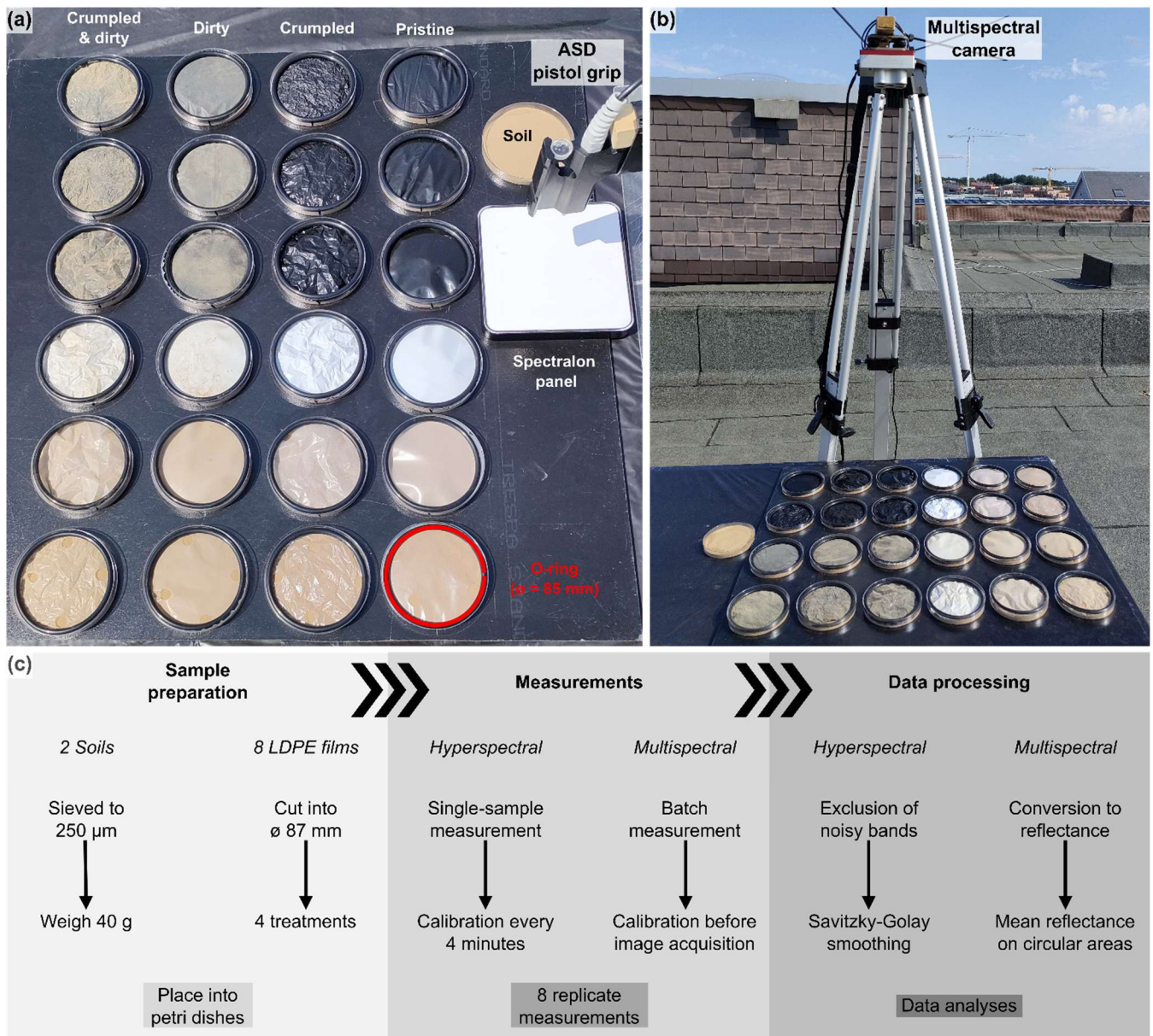
125 | Figure 1 — Experimental setup used for acquiring reflectance measurements of plastic films from a spectroradiometer (i.e., ASD) (a) and a multispectral camera (b), and workflow used (c). The same batch of samples is represented on the left (a) and on the right part of the image (b). On the left side (a), columns were labelled according to the treatment; different rows show different film types, from top to bottom: Black - biodegradable, Black - type 1, Black&White - small (black side), Black&White - small (white side), Transparent - large, Transparent - with holes. Film names refer to Table 1 Table-4 .
