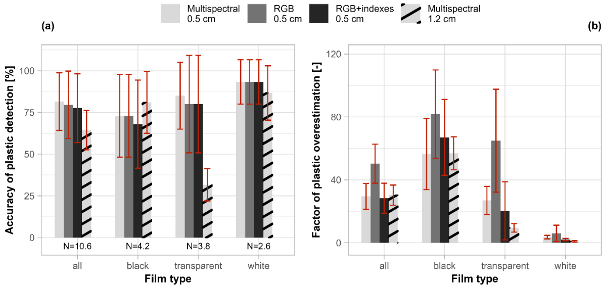
370 Figure 7 – On the left side, accuracy (i.e., producer accuracy) of plastic detection with four different datasets (a), separated by film and aggregated (i.e., ‘all’). Error bars represent the standard deviation of the producer accuracy within the 5-fold cross validation; the numbers below the bars (N) represent the average number of points used for validation. On the right side, factor of plastic overestimation of four different datasets, separated by film and aggregated (b). The factor of plastic overestimation was calculated as the ratio between the detected number and the expected number of plastic-covered pixels. Error bars represent the standard deviation of the overestimation within the 5-fold cross validation.
