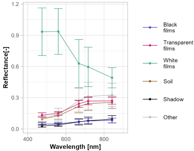
365 Figure 6 – Reflectance of plastic films divided by colour (i.e., black, transparent, white), compared to soil reflectance, shadow, and other non-plastic objects found on the experimental site.
