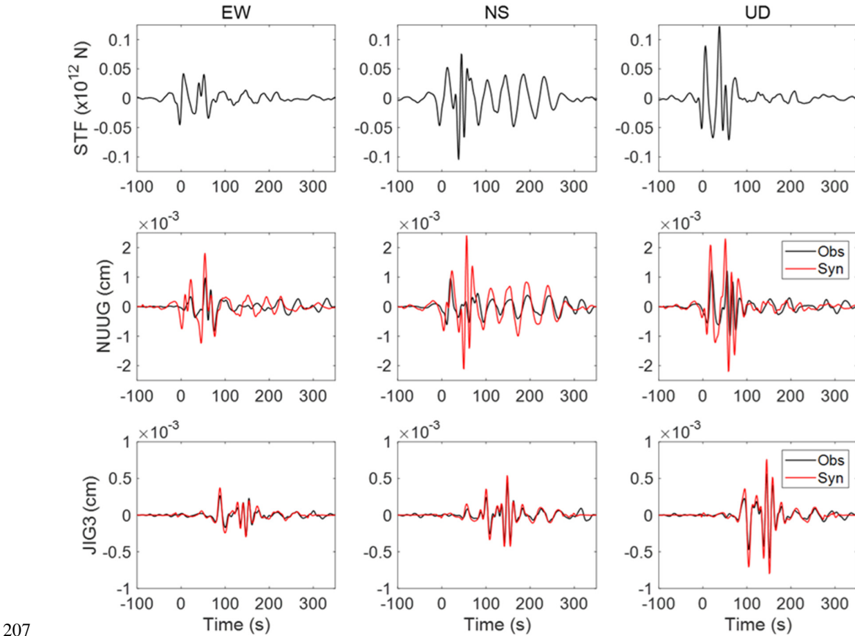
Figure 3: Source time function and waveform fitting. The X-axis shows the time after the origin of the landslide. Columns show the EW, NS, and UD components from the left. Top: Source time function obtained from the waveform inversion with the frequency of 0.02-0.1 Hz. Middle: Comparison between the observed (black) and synthetic (red) waveforms at NUUG station, not included in the inversion. Note that the horizontal components at NUUG station were oriented to 79 and 169 degrees from North, so they were rotated correctly. Bottom: Comparison for the JIG3 station used in the inversion.
