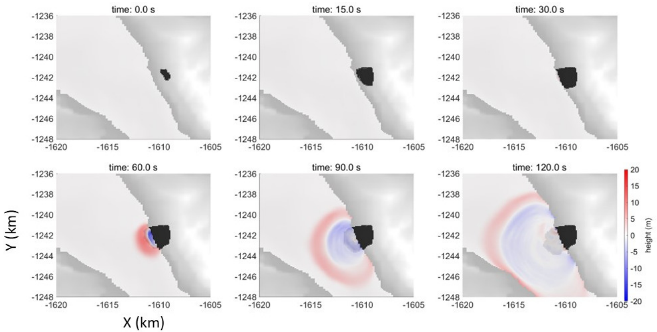
227 Figure 4: Snapshot of the simulation of landslide and tsunami generation. The black area indicates an ongoing landslide on 228 the target slope. The landslide arrives at the sea in around 30 seconds. The generated tsunami height is shown in the colour 229 scale in meters. The map uses the Polar Stereographic projection coordinates (EPSG:3996, true scale set at 75°N). The map 230 scale is in kilometres.
