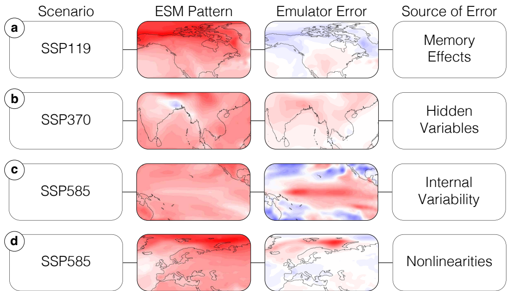
Figure 1. Potential sources of emulator error by scenario; emulator . Emulator errors shown here are meant for illustrative purposes only; we introduce experiments which reproduce these errors in simplified climate models (e.g. box models) in Sect. 3. (a) Pattern scaling emulator trained on historical and SSP585 , tested against SSP119 in 2100; error over northern North America results from memory effects. (b) Pattern scaling emulator trained on historical , tested against SSP370 in 2050; error over India and SE Asia results from hidden variables (aerosols not contained in training data). (c) High-order polynomial pattern scaling emulator trained on historical , tested against SSP585 in 2020; error results from overfitting on internal variability. (d) Pattern scaling emulator trained on historical , tested against SSP585 in 2100; error results from nonlinear feedbacks in the Arctic. All ScenarioMIP data shown are taken from the MPI Grand Ensemble (O'Neill et al., 2016; Maher et al., 2019).
