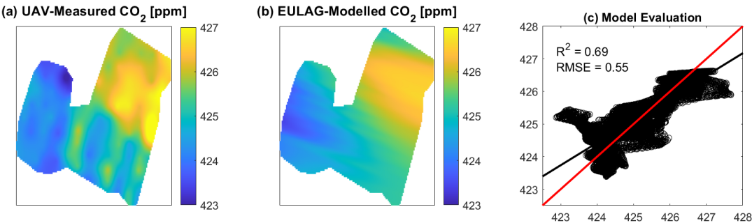
Figure 4: Evaluation of modelled \text{CO}_2 concentration fields at 10m height for Simulation 1 corresponding to the lc_5 configuration. Panel (a) shows a grid survey of the observed concentrations as measured by the UAV, panel (b) the corresponding modeled total concentrations. Panel (c) plots the results of the linear regression applied to modelled concentration vs. observed concentration. It must be noted that here we removed the spatial-temporal average modeled concentration from the modeled concentration values and added the UAV-observed spatial-temporal average, thus, accounting for the difference in background concentrations, which is constant offset in this case. Concentrations are reported in ppm.
