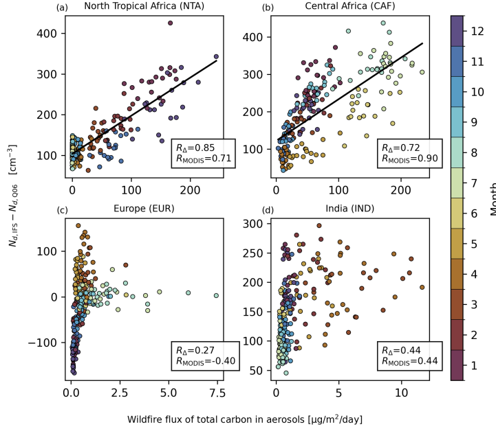
Figure 13. Scatter plot of wildfire flux of total carbon in aerosols (WFTCA) from the GFAS system and differences between simulated and MODIS ‘Q06’ monthly N_d (2003–2020). R_{\Delta} and R_{MODIS} indicate the Pearson’s correlation coefficients between WFTCA and respectively, the difference \Delta = N_{d,IFS} - N_{d,Q06} ( R_{\Delta} ), and N_{d,Q06} ( R_{MODIS} ).
