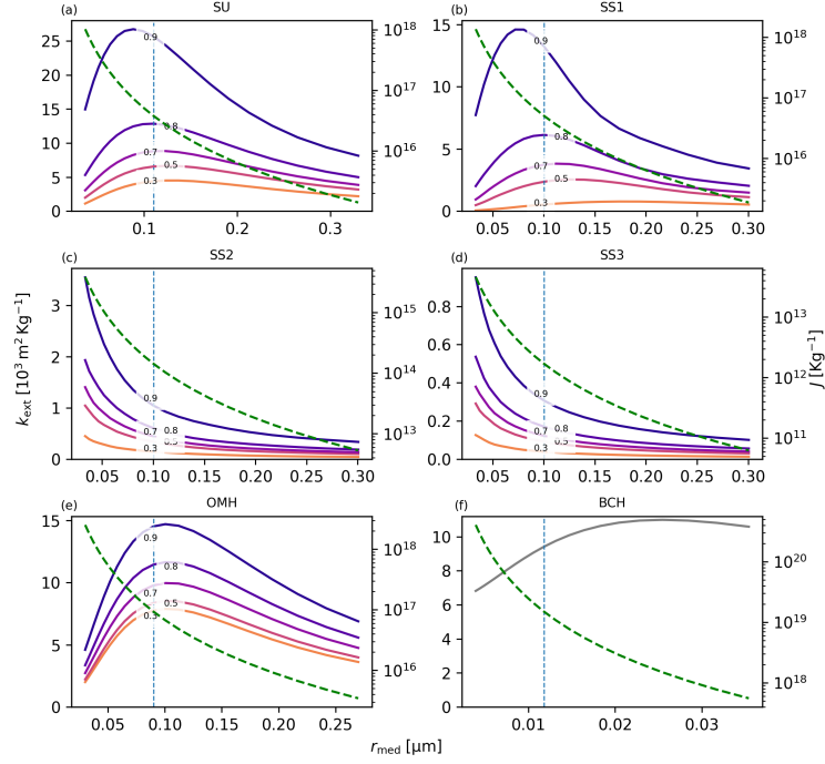
Figure 1. Mass extinction coefficient k_{\text{ext}} at 550 nm and number concentration per unit mass J (as defined in Equation 2) as a function of the median radius r_{\text{med}} of the number PSD for the hydrophilic aerosol species listed in Table 1. Labels indicate selected relative humidity values. Nitrates and ammonium are not shown, but their optical properties are very close to sulfates for the purpose of this discussion. The dashed green line shows the number of particles per unit mass J as a function of r_{\text{med}} and its scale is given on the right of each plot. For each tracer, the vertical dashed line indicates the default dry median radius according to Table 1. For sea salt, the ratio between the median radii of the two modes r_{\text{med},2}/r_{\text{med},1} was kept constant, and the dashed line indicates the location of the finer mode.
