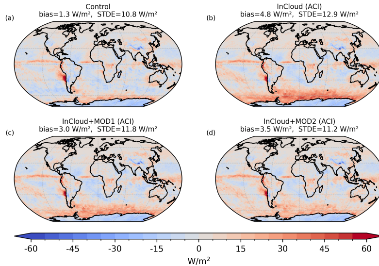
Figure 9. Mean top-of-atmosphere (TOA) shortwave (SW) radiation flux (outgoing), difference of CERES minus IFS difference for the season DJF 2023-2024 2023-2024, with global bias and error standard deviation (STDE) on monthly means for each experiment. For the control simulation (a) N_d does not depend on aerosols; for in panels (b), (c) and (d) N_d is diagnosed from aerosols (label ACI) using optimal PSDs from the InCloud setup. These use the default IFS IN-SCAV configuration (b), MOD1 (c) and MOD2 (d). Details are provided in the text.
