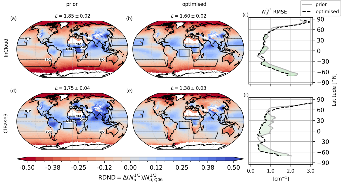
Figure 3. Offline-simulated mean N_d for the 18-year-period-of-18-year optimisation period from prior (IFS-COMPO default) (a, d) and optimised (b, ee ) aerosol PSDs, shown both-in-as relative differences in N_d^{1/3} (RDND) maps (a, b, d, e) and zonal N_d^{1/3} RMSE (c, f) with respect to the MODIS N_d optimisation target, Q06. These are for the optimisation setups InCloud (aerosols diagnosed at cloud level - panels a, b, c) and ClBase3 (aerosols diagnosed three model levels below cloud base - panels d, e, f). Positive-differences-Negative RDND values indicate that MODIS N_d (Q06) values are-higher-than-those-exceed the simulated values . Labelled boxes indicate regions used for regional evaluation and are presented later in Table 3 and Figure 4. For each map, the corresponding loss function \mathcal{L} value (see Equation 7) is reported.
