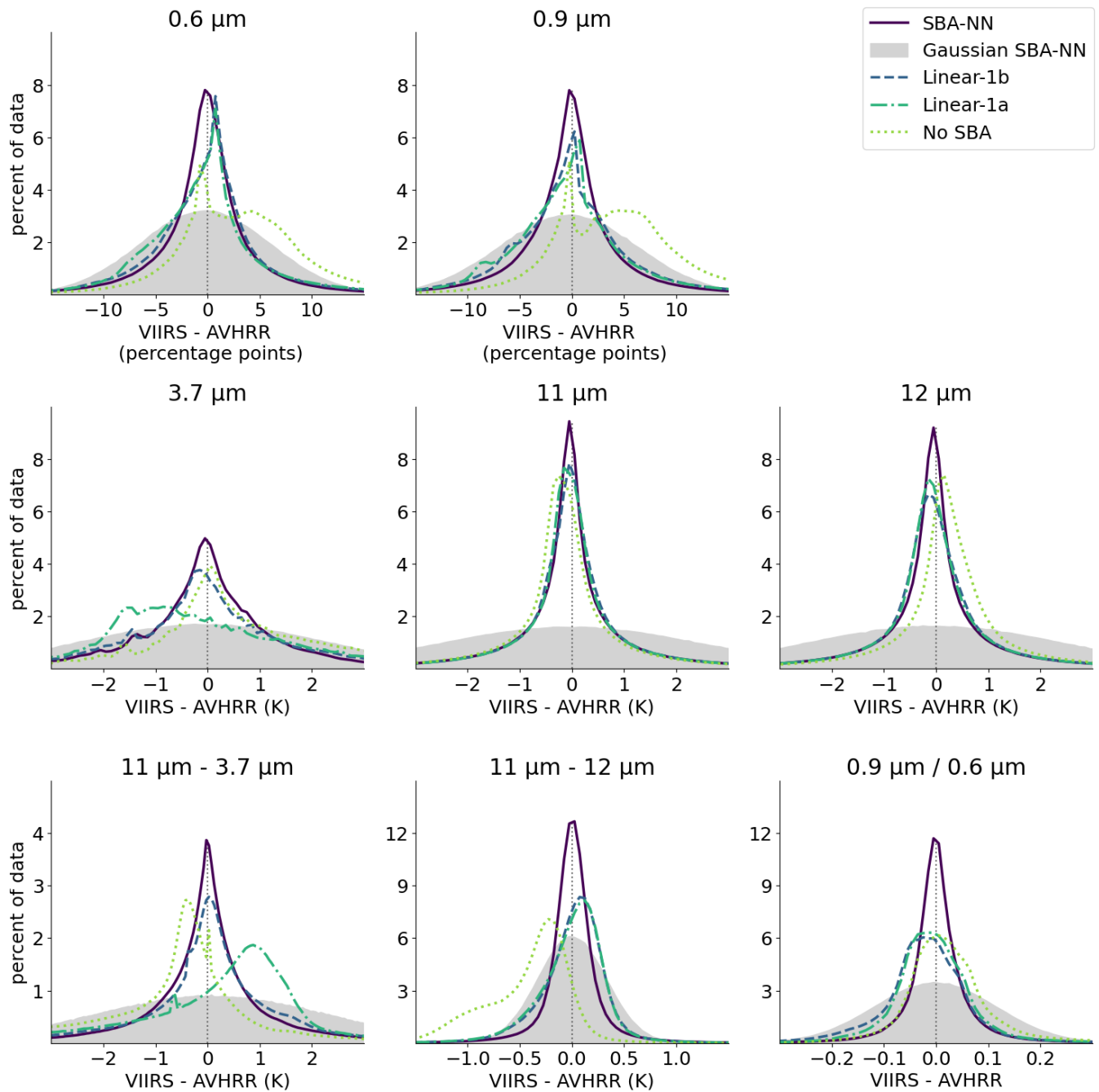
Figure 6: Frequency distributions of differences between simulated and real AVHRR radiances and brightness temperatures. For reference, also the original AVHRR and VIIRS channel deviations are shown (green dotted curve = No SBA in the legend). The upper two panels show results for all 5 AVHRR channels, while the bottom panels show
