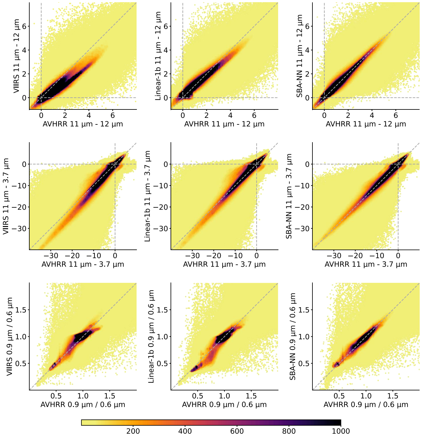
Figure 5: Results for selected channel differences and ratios. The figure shows merged results for all three daytime categories. Uppermost panels: Results for original and simulated brightness temperature differences (K) between AVHRR channels 4 and 5 (11-12 \mu\text{m} ). Middle panels: Results for original and simulated brightness temperature
