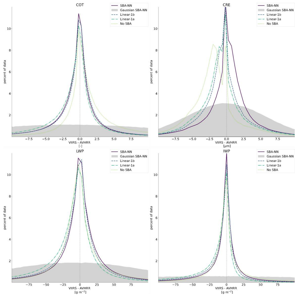
510 Figure 7: Frequency distributions of CPP differences between products based on VIIRS-simulated and real AVHRR radiances. For reference, also products based on uncorrected VIIRS radiances are shown (green dotted curve = No SBA in the legend).
