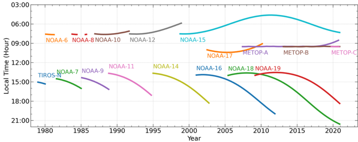
195 Figure 2: Local solar times at equator observations for all AVHRR-carrying NOAA satellites from TIROS-N to NOAA-19 and EUMETSAT's METOP A/B/C satellites. Shown are all data that were used for the CLARA-A3 CDR processing. The figure shows ascending (northbound) equator crossing times for afternoon satellites (NOAA-7 to NOAA-19) and descending (southbound) equator crossing times for morning satellites (NOAA-12 to NOAA-17 and METOP A/B/C). Corresponding night-time observations take place 12 hours earlier/later. To be noticed is that Suomi-NPP has a stable orbit with equator crossing time at 13:30.
