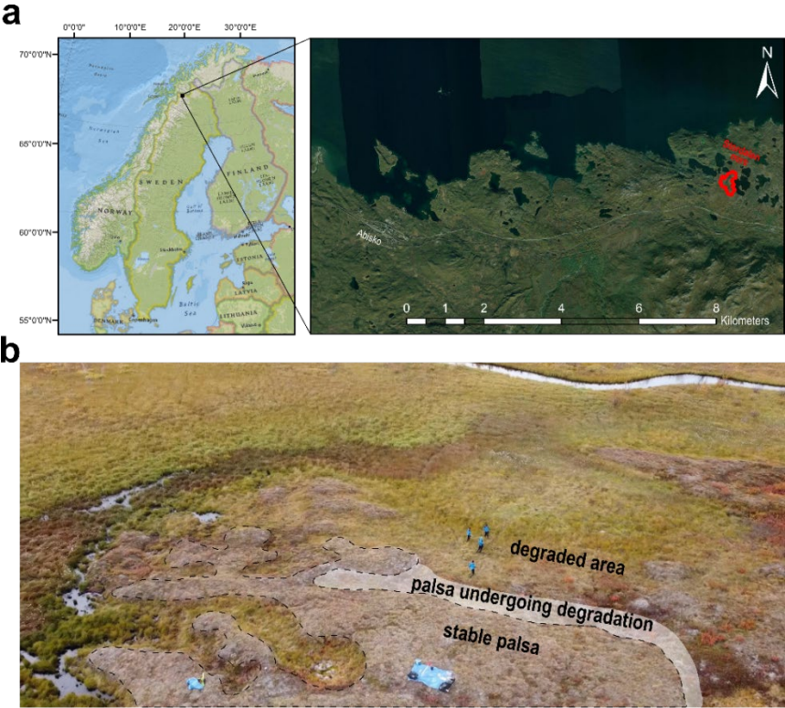
140 Figure 1: Location and photograph of the degradation gradient studied. (a) Map of the study site at the Stordalen mire, Abisko Sweden. Map created with ArcMap® 10.8. Basemap sources: National Geographic (© National Geographic et al., 2011) and World Imagery (© Esri and Maxar, 2022). The projected coordinate system is EPSG: 3006. Delineation adapted from Christensen et al. (2004) in red; (b) Illustration of the degradation gradient showing ground subsidence in the field (photo credit: Maxime Thomas)
