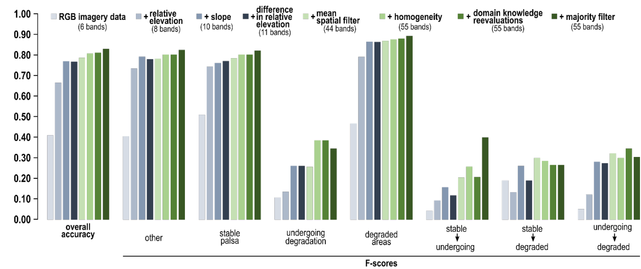
Figure C1: Performance evaluation of the biennial (2019 – 2021) model. (a) Mean permutation importance (scikit-learn built-in function) of each input data in the model, measured as the decrease in accuracy when the input data values are randomly shuffled. The error bars indicate the standard deviation of importance across 10 permutations. (b) Evolution of the overall accuracy and F-scores of the classes based on the input data for the classification. Mean spatial filter = mean of pixel values in 3 \times 3 , 5 \times 5 and 7 \times 7 moving windows. Homogeneity = texture attribute 'homogeneity' based on the gray-level co-occurrence matrix applied within a 21 \times 21 moving window. Domain knowledge reevaluation = refinement using elevation differences and model scores to ensure alignment with domain knowledge (see section 2.4). majority filter = filter using windows of increasing size up to 11 \times 11 pixels, to reduce noise and enhance classification consistency.
