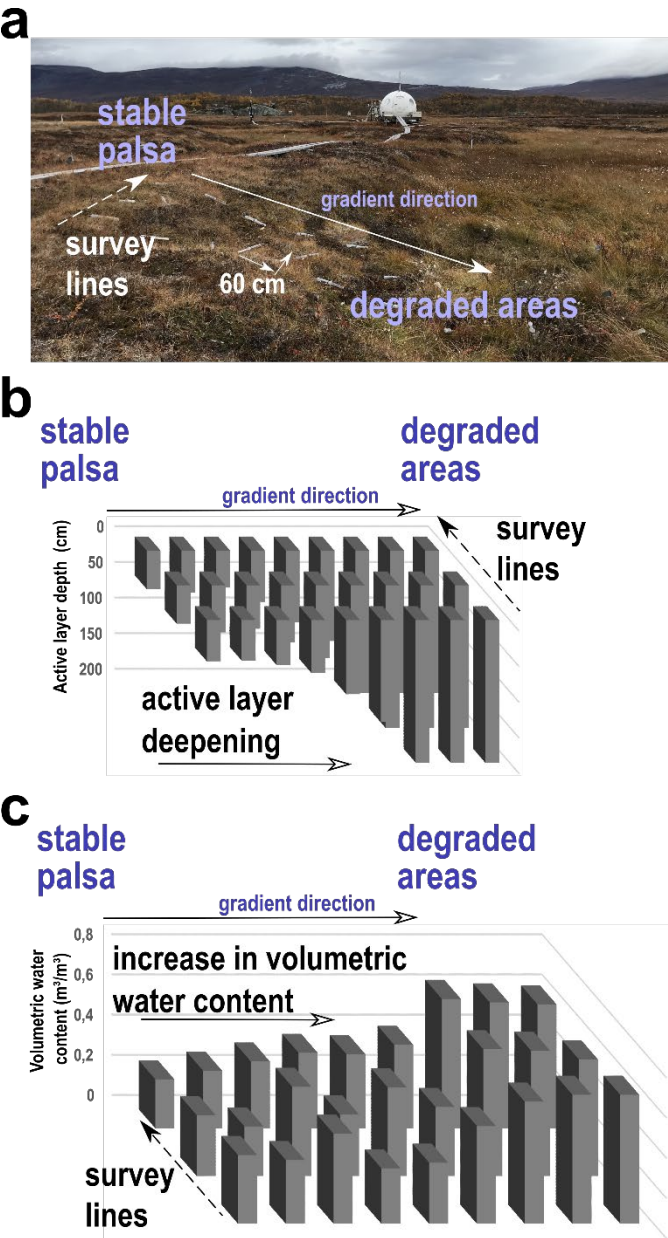
Figure A2: Conceptual model and illustration of the permafrost degradation gradient at the Stordalen Mire. (a) measuring grid along the gradient (photo: S. Opfergelt; Sept 30, 2021) where point-to-point distance is indicated for scale; (b) evolution of active layer depth along the gradient; (c) evolution of the volumetric water content along the gradient
