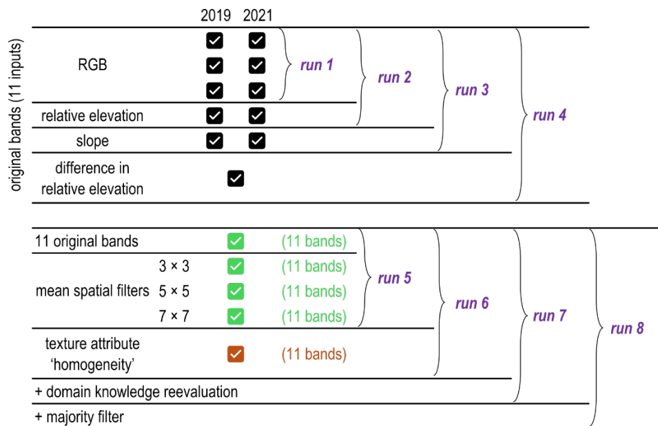
540 Figure A5: Workflow of the different runs of the model with successive additional data inputs and post-processing steps.
