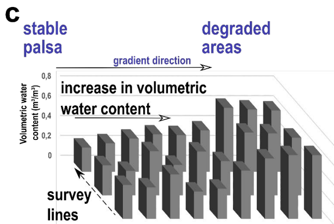
Figure A2: Conceptual model and illustration of the permafrost degradation gradient at the Stordalen Mire. (a) measuring grid along the gradient (photo: S. Opfergelt; Sept 30, 2021) where point-to-point distance is indicated for scale; (b) evolution of active layer depth along the gradient; (c) evolution of the volumetric water content along the gradient
