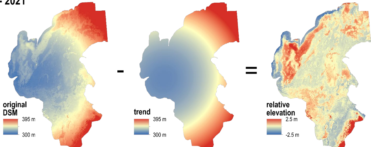
Figure A3: Removing of the bowl-shape effect from elevation data (DSM) for (a) 2019 and (b) 2021. The processing involves (i) extraction of the original elevation band on a regular 5 m x 5 m grid; (ii) on this grid, exclusion of the data that diverge by more than 3 times the standard deviation, and calculation of the second-order trend from those data that from the original elevation data; (iii) calculation of residuals by subtraction of the 2nd-order trend from the original data. The result represents the relative elevation data (corrected DSM)
