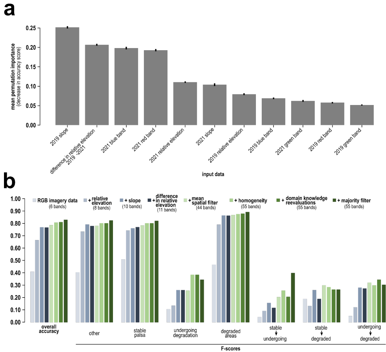
Figure C1: Performance evaluation of the biennial (2019 – 2021) model. (a) Mean permutation importance (scikit-learn built-in function) of each input data in the model, measured as the decrease in accuracy when the input data values are randomly shuffled. The error bars indicate the standard deviation of importance across 10 permutations. (b) Evolution of the overall accuracy and F-scores of the classes based on the input data for the classification. Mean spatial filter = mean of pixel values in 3 \times 3 , 5 \times 5 and 7 \times 7 moving windows. Homogeneity = texture attribute ‘homogeneity’ based on the gray-level co-occurrence matrix applied within a 21 \times 21 moving window. Domain knowledge reevaluation = refinement using elevation differences and model scores to ensure alignment with domain knowledge (see section 2.4). majority filter = filter using windows of increasing size up to 11 \times 11 pixels, to reduce noise and enhance classification consistency.
