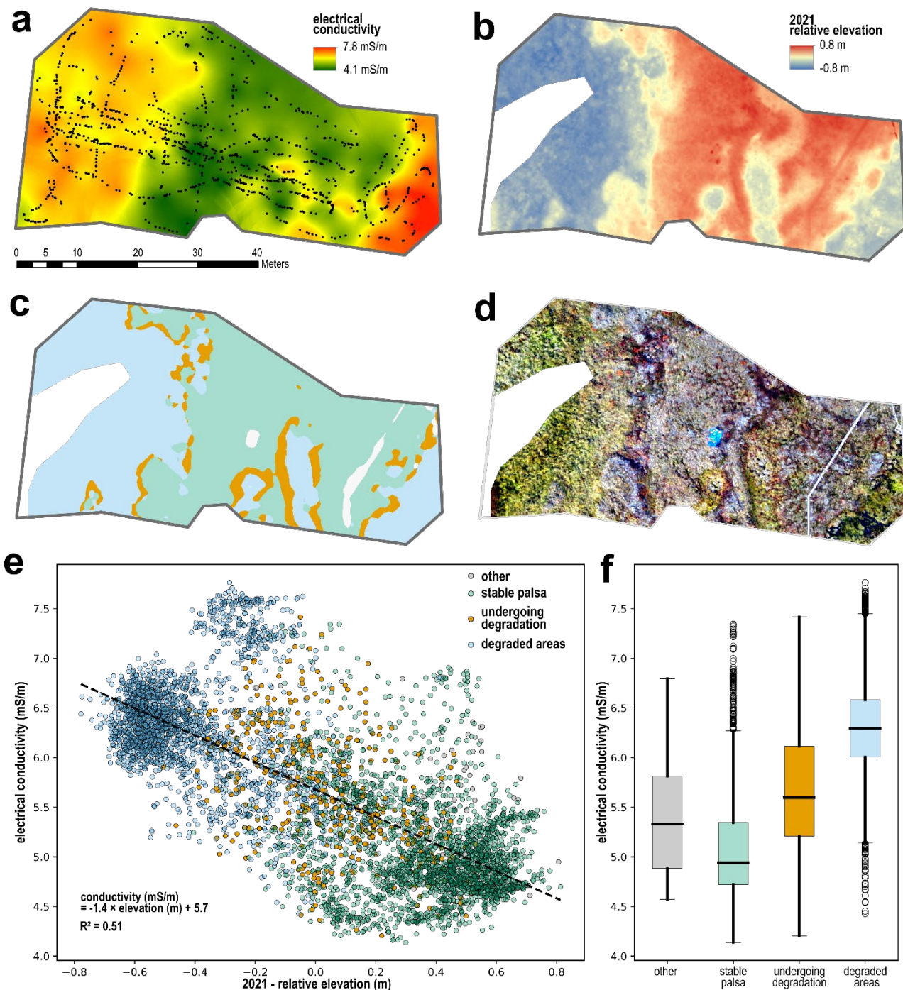
440 Figure 7: Evolution of electrical conductivity data and comparison with the results of the biennial classification model (between 2019 and 2021). (a) Continuous map of electrical conductivity obtained by simple kriging of point data; (b) Relative elevation data corrected by removal of the bowl-shape effect; (c) Classification model results for 2021 (see Fig. 4b for the entire model); (d) RGB imagery data for 2021; (e) Linear regression between electrical conductivity and relative elevation for the different classes; (f) Boxplots of the electrical conductivity per land cover class. Data processing extent as in Fig. 2a . Color code as in Fig. 4 .
