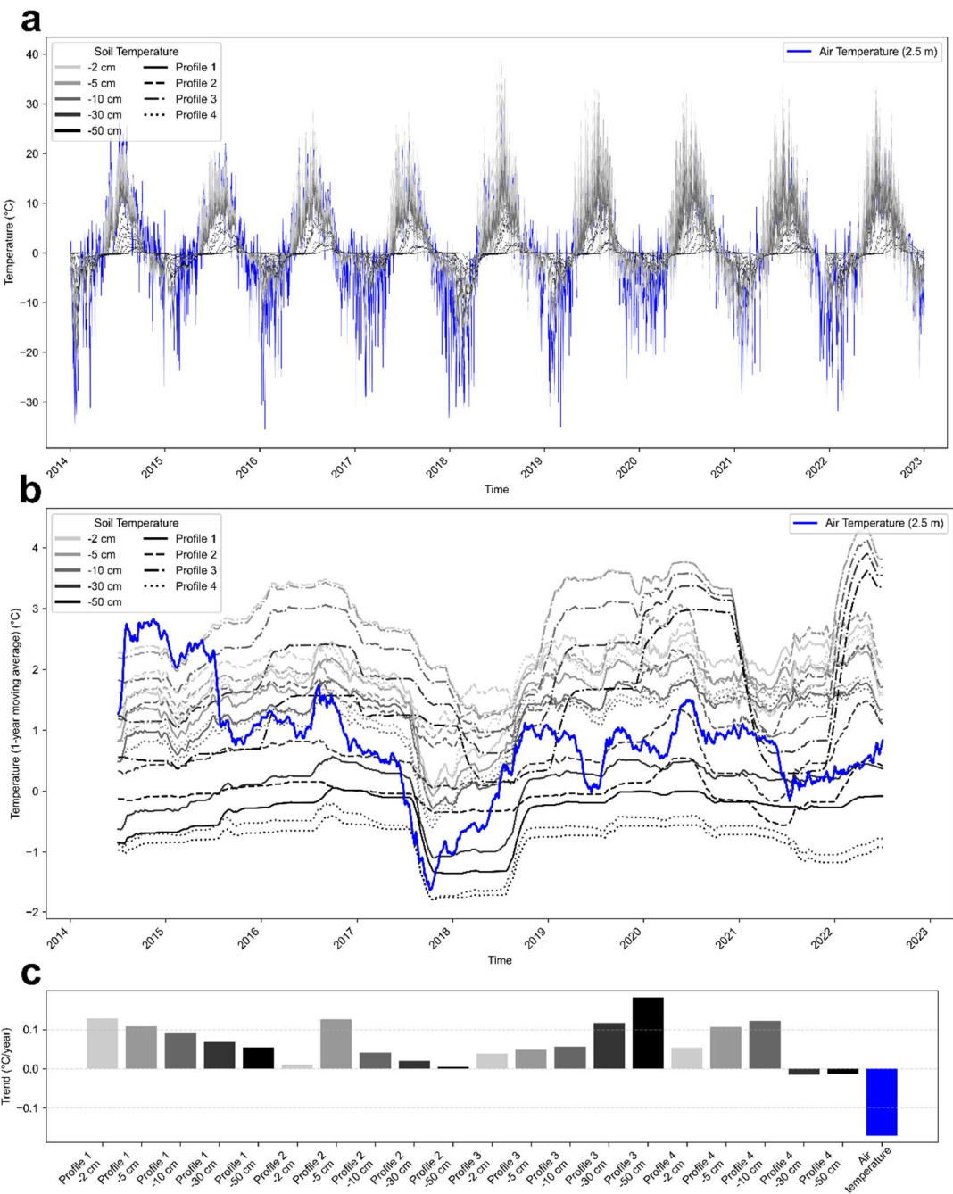
535 Figure A-1 : Air and ground temperatures at Stordalen between 2014 and 2022. (a) half-hourly air temperature at 2.5 m and soil temperatures from 4 profiles at 2, 5, 10, 30, and 50 cm depth (ICOS Sweden, 2023); (b) annual moving averages calculated on these same data; (c) significant trends in temperature changes calculated from moving averages (p-values < 10 -3 ).
