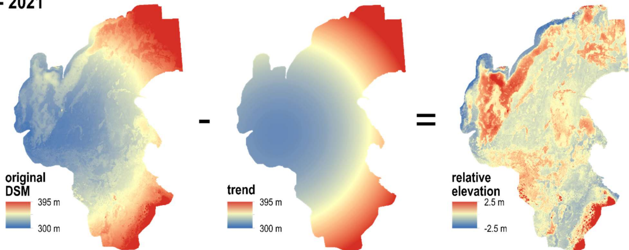
Figure A-3: Removing of the bowl-shape effect from elevation data (DSM) for (a) 2019 and (b) 2021. The processing involves (i) extraction of the original elevation band on a regular 5 m x 5 m grid; (ii) on this grid, exclusion of the data that diverge by more than 3 times the standard deviation, and calculation of the second-order trend from those data that from the original elevation data; (iii) calculation of residuals by subtraction of the 2nd-order trend from the original data. The result represents the relative elevation data (corrected DSM)
