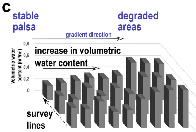
|540 Figure A-2: Conceptual model and illustration of the permafrost degradation gradient at the Stordalen Mire. (a) measuring grid along the gradient (photo: S. Opfergelt; Sept 30, 2021) where point-to-point distance is indicated for scale; (b) evolution of active layer depth along the gradient; (c) evolution of the volumetric water content along the gradient
