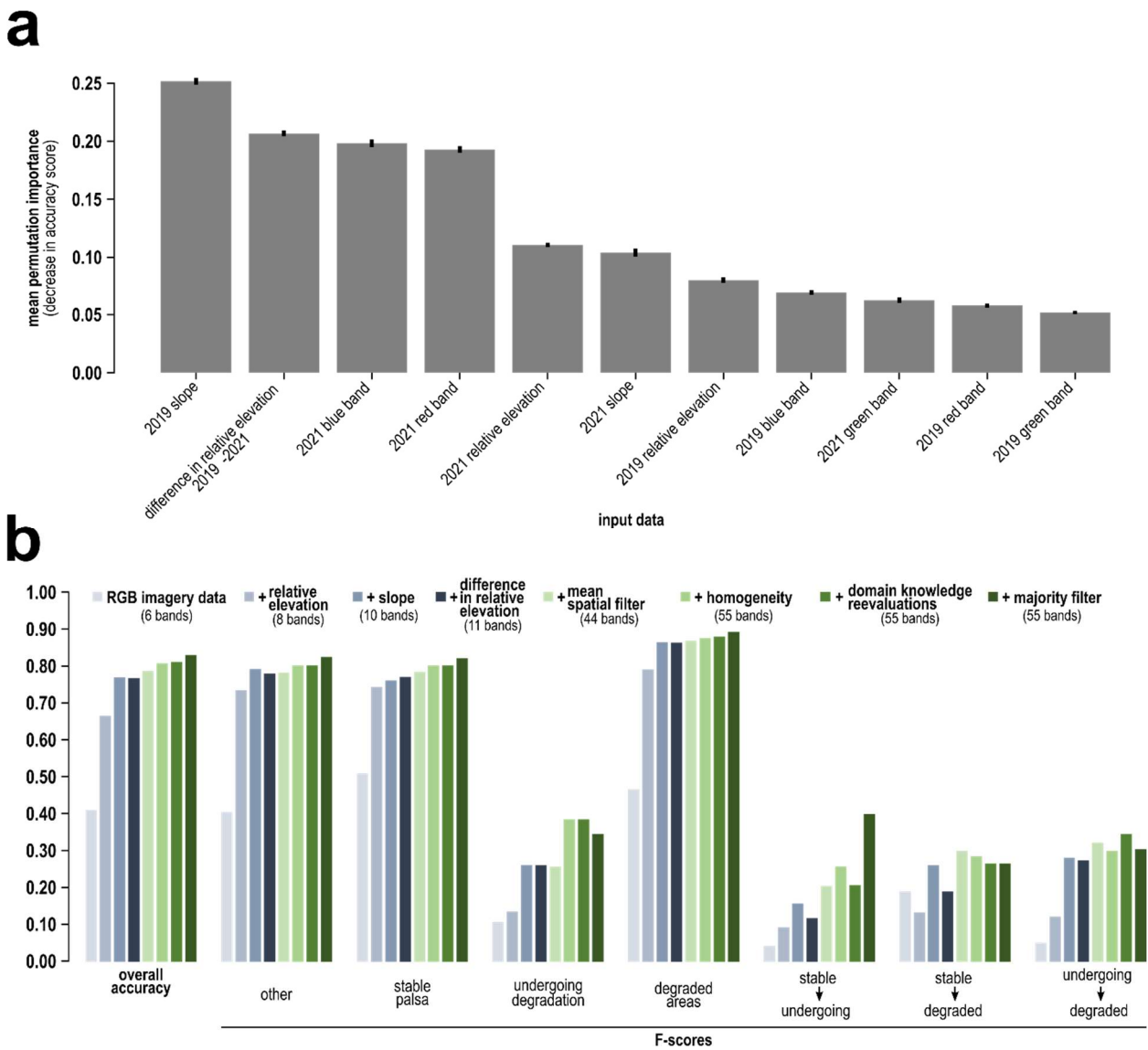
Figure C-1: Performance evaluation of the biennial (2019 – 2021) model. (a) Mean permutation importance (scikit-learn built-in function) of each input data in the model, measured as the decrease in accuracy when the input data values are randomly shuffled. The error bars indicate the standard deviation of importance across 10 permutations. (b) Evolution of the overall accuracy and F-scores of the classes based on the input data for the classification. Mean spatial filter = mean of pixel values in 3 \times 3 , 5 \times 5 and 7 \times 7 moving windows. Homogeneity = texture attribute ‘homogeneity’ based on the gray-level co-occurrence matrix applied within a 21 \times 21 moving window. Domain knowledge reevaluation = refinement using elevation differences and model scores to ensure alignment with domain knowledge (see section 2.4). majority filter = filter using windows of increasing size up to 11 \times 11 pixels, to reduce noise and enhance classification consistency.
