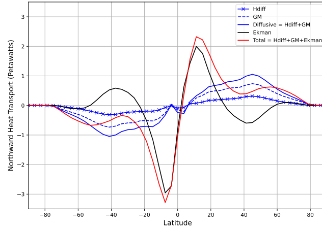
Figure 5. Contribution of each ocean heat transport (OHT) term towards the northward meridional OHT (in Petawatts, red line) for Case 7 (all OHT on) of the oblique aquaplanet simulation. Horizontal diffusion (crossed blue) and Gent-McWilliams (dashed blue) together make up the total diffusive transport (solid blue), while Ekman transport is in black.
