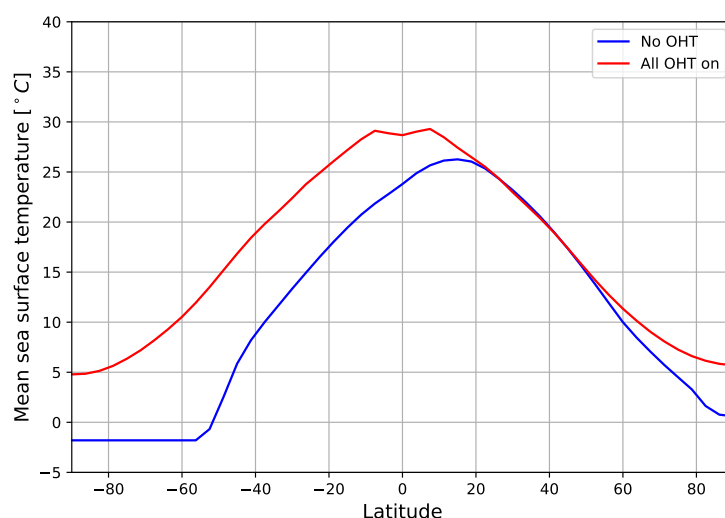
Figure 10. Ocean heat transport (OHT) suppresses hemispheric climate asymmetries caused by initialisation biases: zonally averaged sea surface temperatures for our oblique aquaplanet setup, with OHT disabled (blue) and enabled (red).
