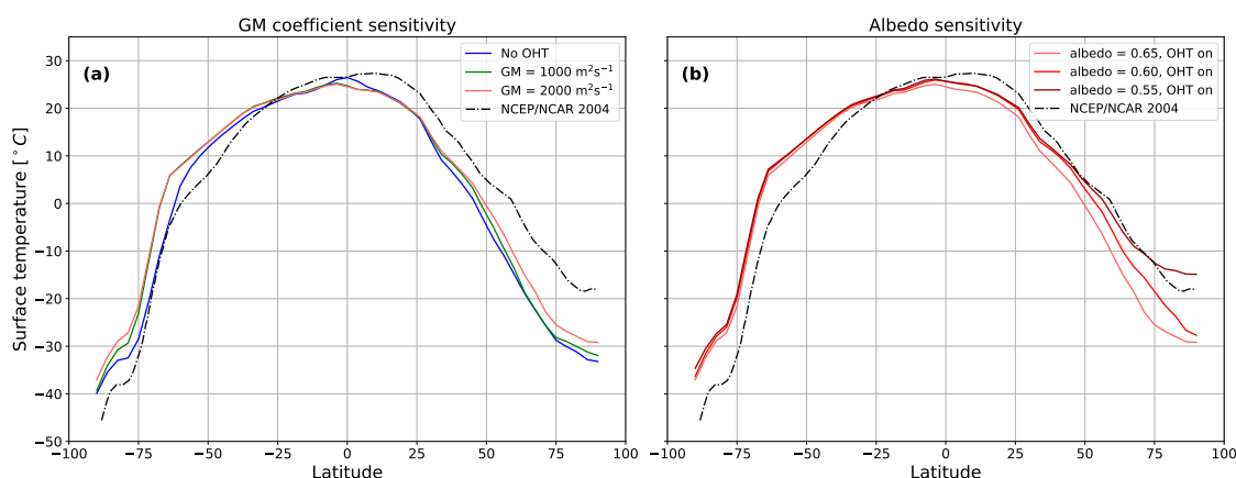
Figure 11. Zonally averaged surface air temperature for modern Earth simulations under two different sensitivity experiments. (a) Gent-McWilliams (GM) coefficient sensitivity test comparing model simulations with two different GM values against NCEP/NCAR reanalysis (black dashed line). (b) Albedo sensitivity test comparing model simulations with three different sea ice/snow albedo values against reanalysis data.
