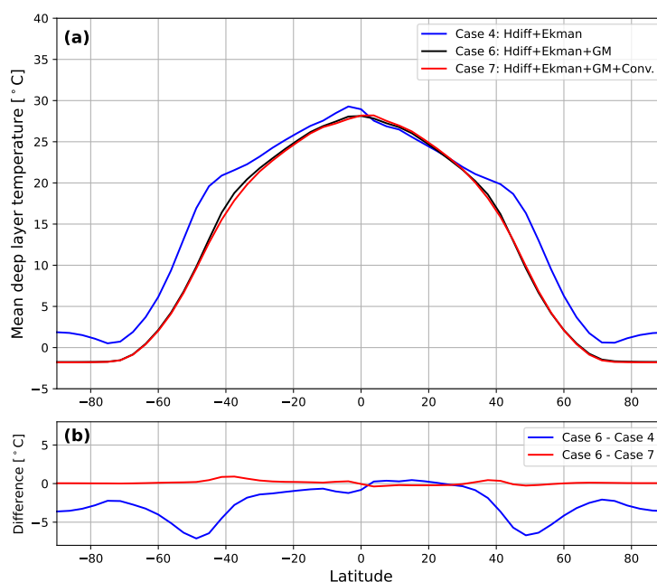
Figure 9. Gent-McWilliams (GM) restratification mimics the effect of convective adjustment: Zonally averaged deep ocean layer temperatures in the aquaplanet simulations. (a) Mean deep layer temperature (in °C) for cases including horizontal diffusion and Ekman transport (blue), with the addition of GM (black), and finally with convective adjustment (red). (b) Differences between selected simulations.
