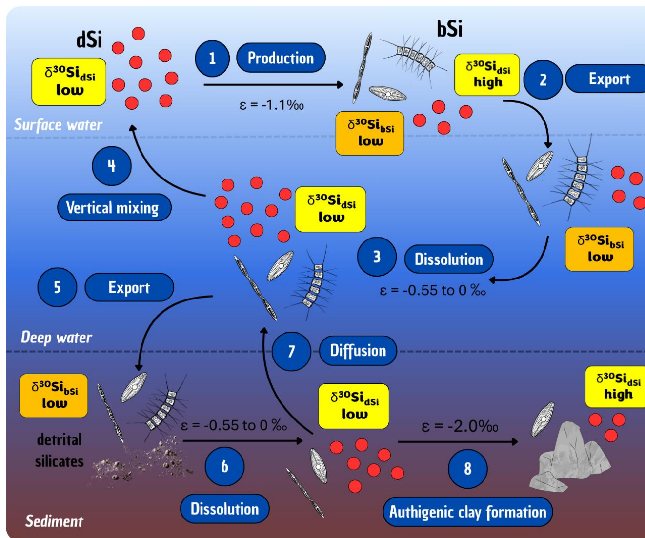
Fig. 4: Schematics of the silicon (Si) cycle and isotope fractionation during various oceanic processes, using diatoms as a model for the biogenic silica ( \text{bSi} ) component. The dissolved silica ( \text{dSi} ) pool is depicted by red dots, with its isotopic composition represented by yellow squares. The \text{bSi} and detrital silicate pools are illustrated with representative symbols (diatoms, sediments, rocks), and their isotopic composition are shown as orange squares.
