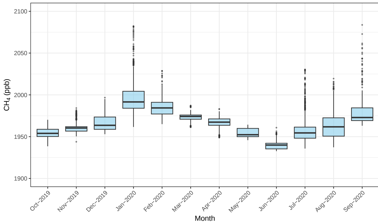
Monthly CH 4 Distributions (Oct 2019 – Sep 2020)
