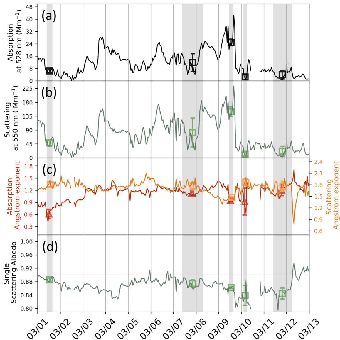
Figure 4: \text{PM}_{10} aerosol optical properties observed by the aerosol system at LABS, the gray-shaded intervals represent continuous cloud events. (a) absorption coefficient; (b) scattering coefficient; (c) Absorption Ångström Exponent (AAE, red) and Scattering Ångström Exponent (SAE, orange); (d) Single Scattering Albedo (SSA), and gray dash line means \text{SSA} = 0.9 .
