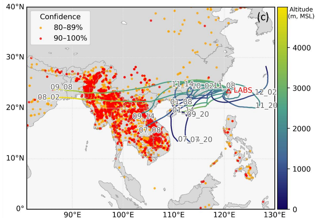
Figure 2: (a) Himawari 8 true color satellite image and (b) surface chart from Central Weather Administration (CWA) at 08 LT (UTC +8), March 7, 2024. (c) Fire points data from March 1 to March 12, 2024, were plotted together with the timing of major cloud events (DD_HH, LT) using 72-hour backward trajectories. Fire hotspot data were obtained from MODIS onboard Terra and Aqua, considering only those with confidence levels above 80%. The backward trajectories were calculated using the NOAA HYSPLIT model ( GFS\ 0.25^{\circ} \times 0.25^{\circ} ) and displayed at 6-hour intervals.
